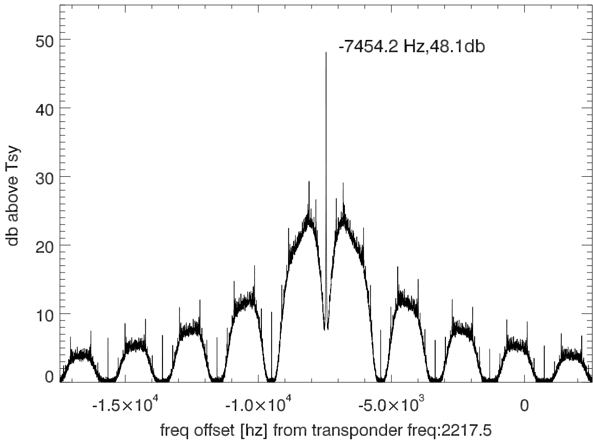
isee3 140613:201909 (UTC) spectra after doppler correction. PoIB
