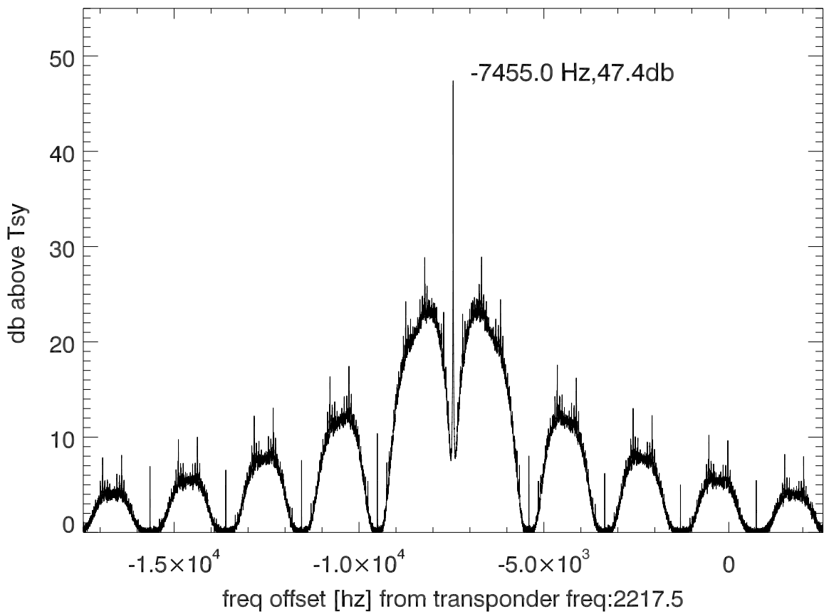
isee3 140613:193641 (UTC) spectra after doppler correction. PoIB
