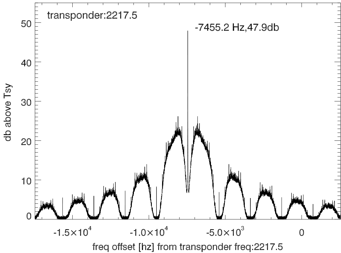
isee3 140613:192914 (UTC) spectra after doppler correction. PolA
