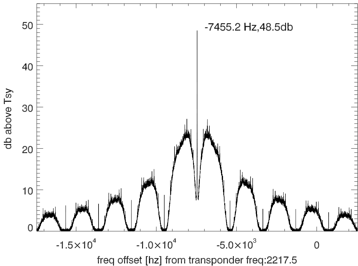
isee3 140613:192914 (UTC) spectra after doppler correction. PolB
