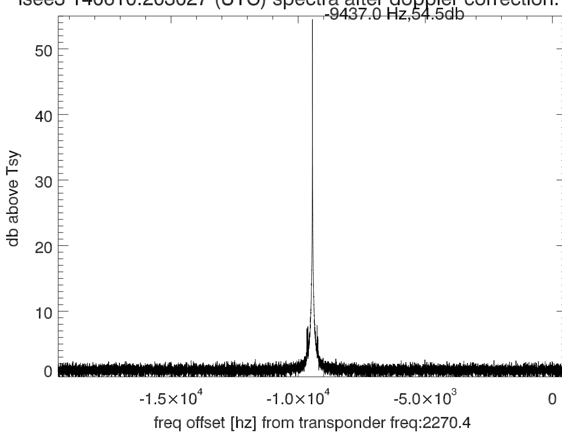
isee3 140610:203027 (UTC) spectra after doppler correction. PoIB
