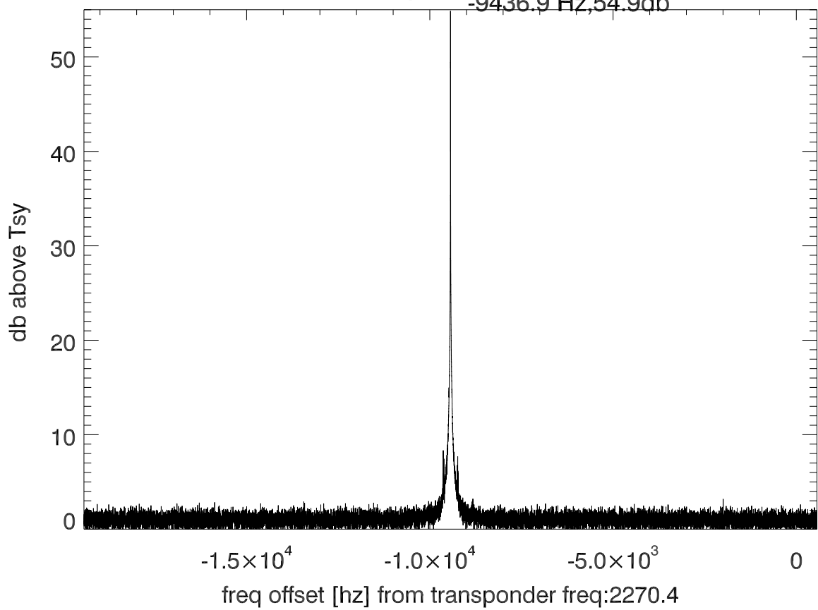
isee3 140610:201859 (UTC) spectra after doppler correction. PolB
