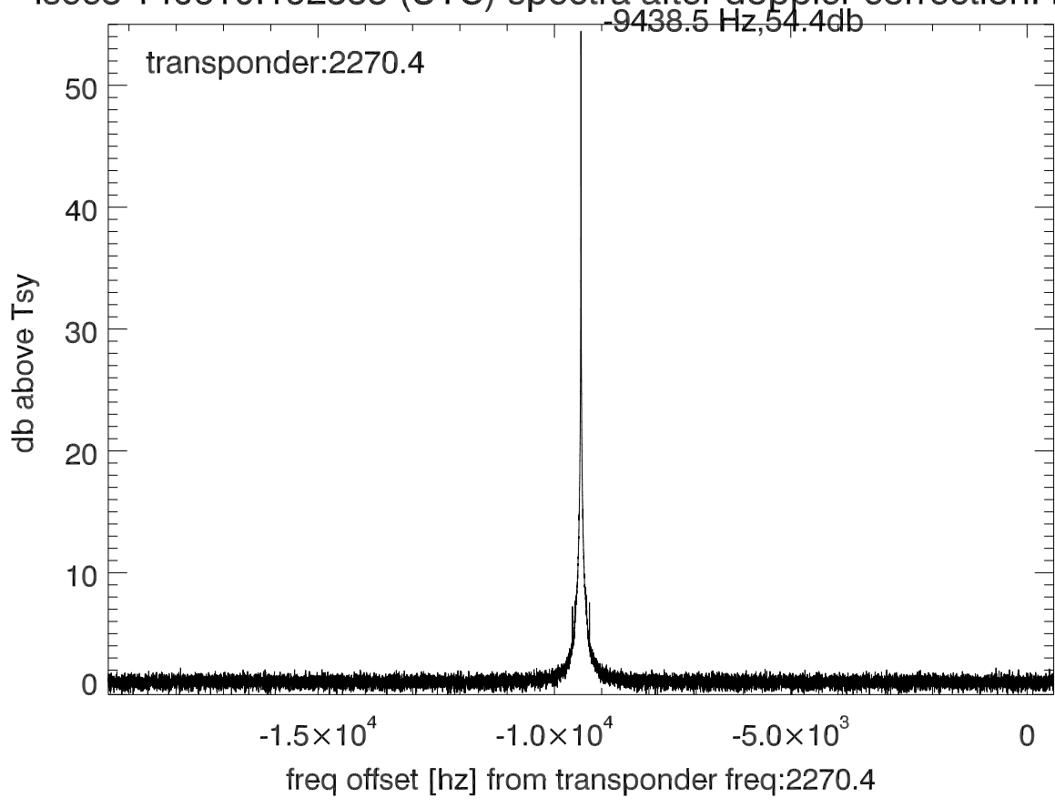
isee3 140610:192553 (UTC) spectra after doppler correction. PolB
