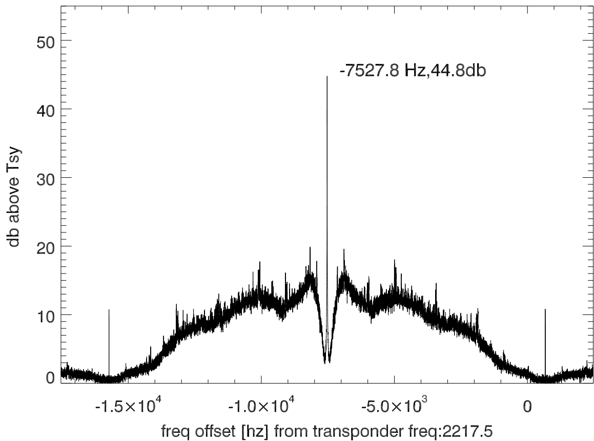
isee3 140610:204309 (UTC) spectra after doppler correction. PolB
