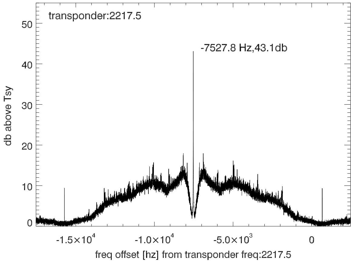
isee3 140610:204309 (UTC) spectra after doppler correction. PolA
