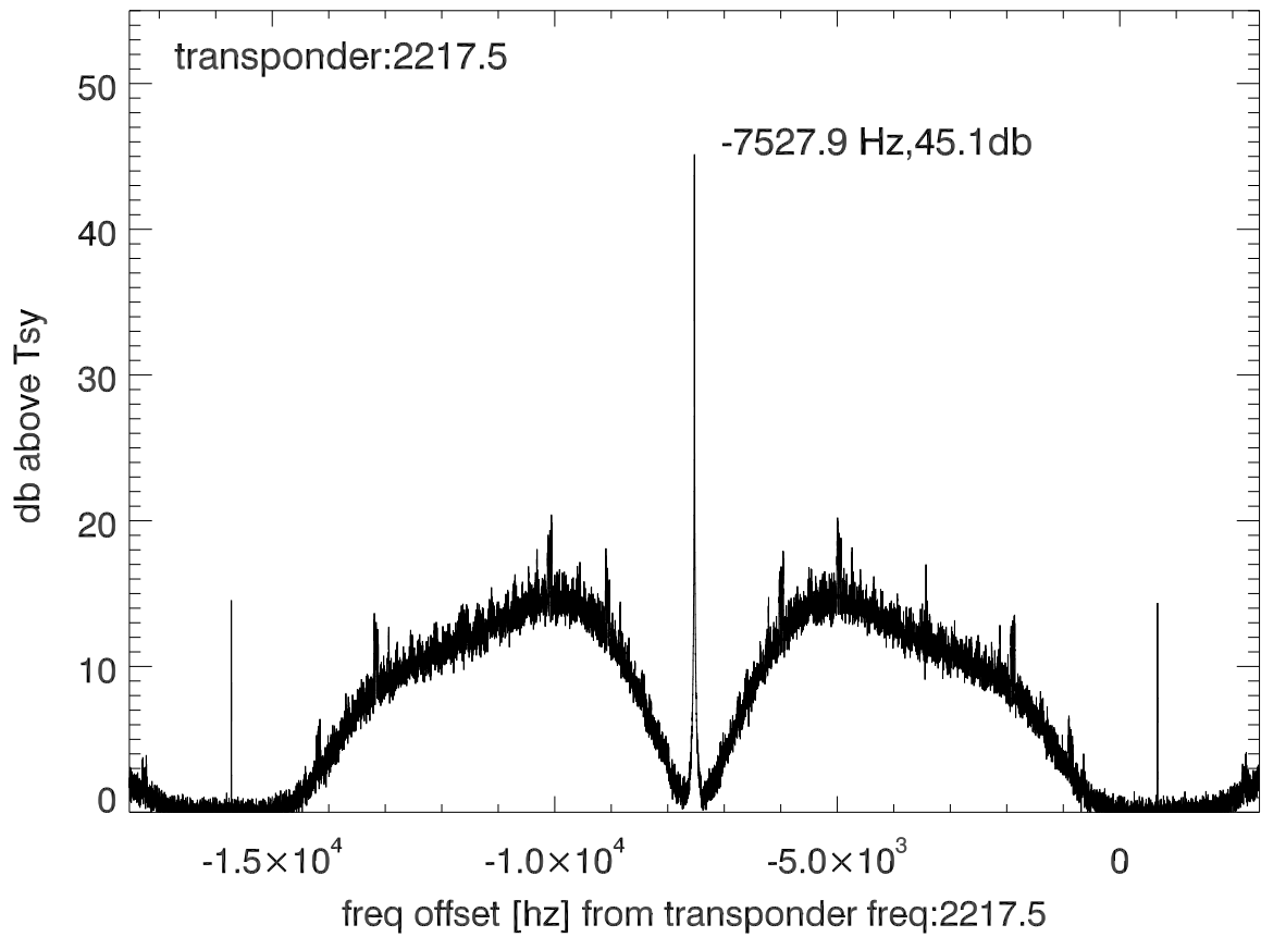
isee3 140610:203027 (UTC) spectra after doppler correction. PolA
