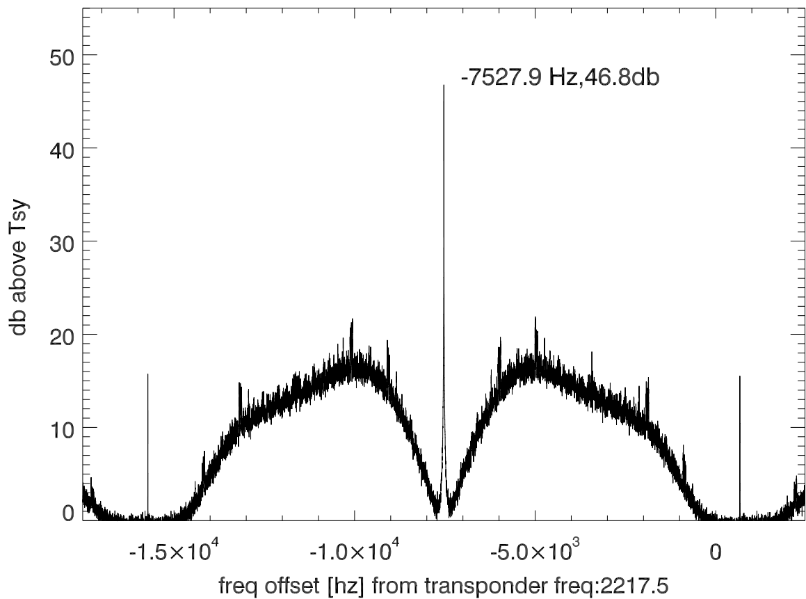
isee3 140610:203027 (UTC) spectra after doppler correction. PolB
