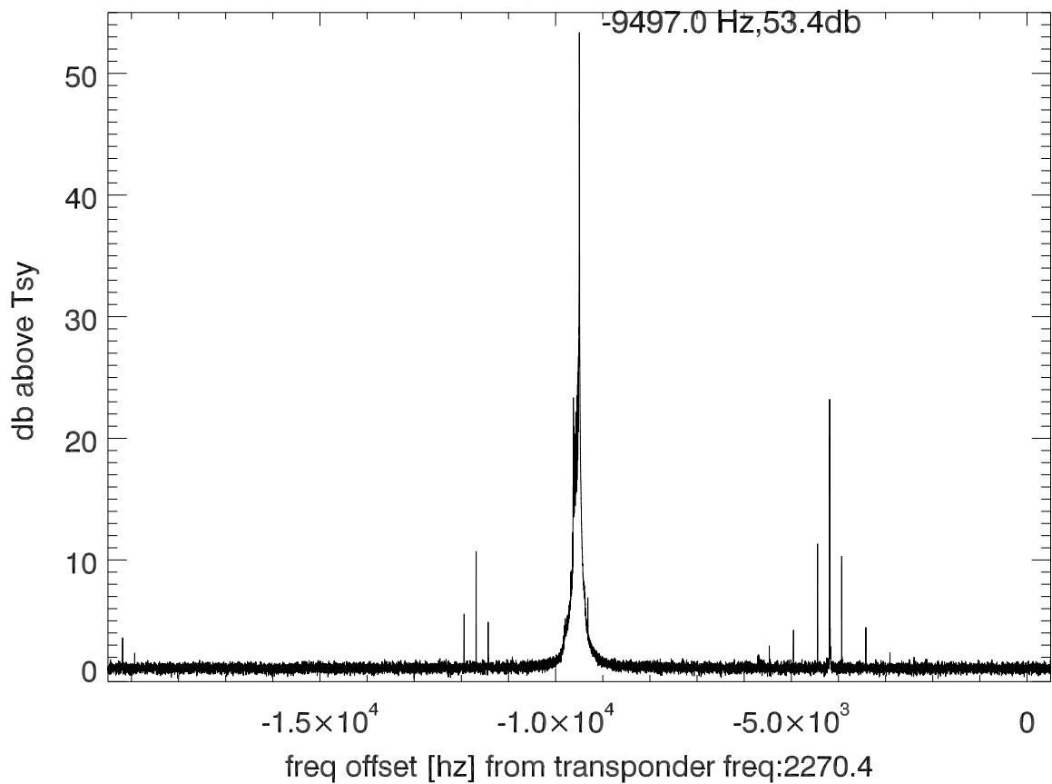
isee3 140609:201412 (UTC) spectra after doppler correction. PolB
