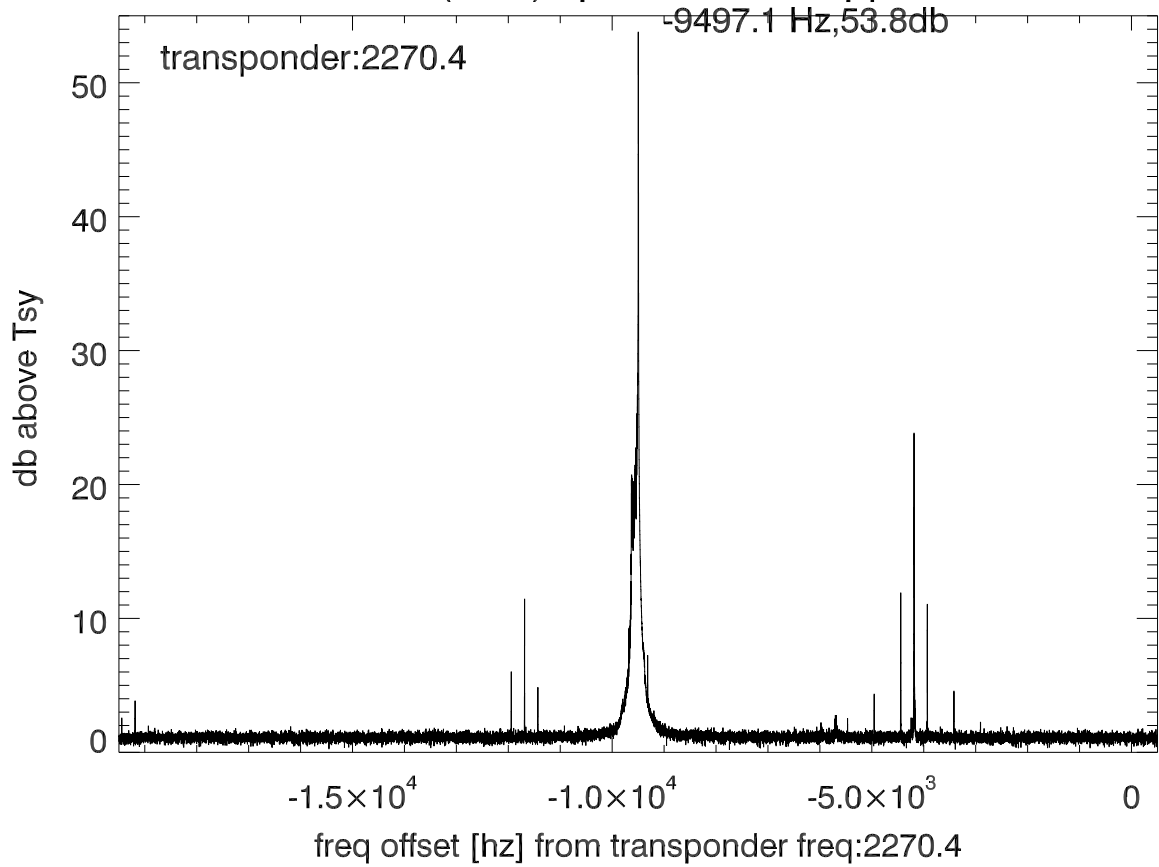
isee3 140609:201412 (UTC) spectra after doppler correction. PolA
