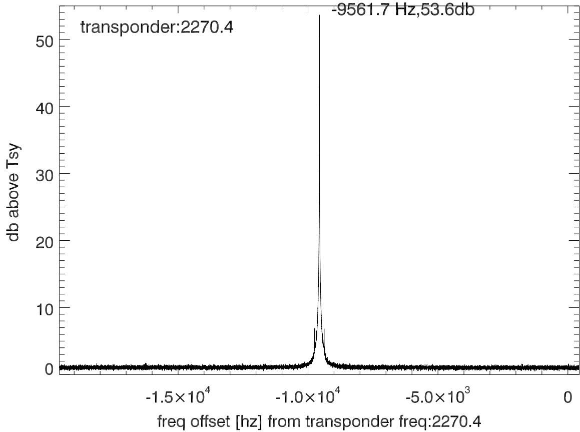
isee3 140608:203241 (UTC) spectra after doppler correction. PolA
