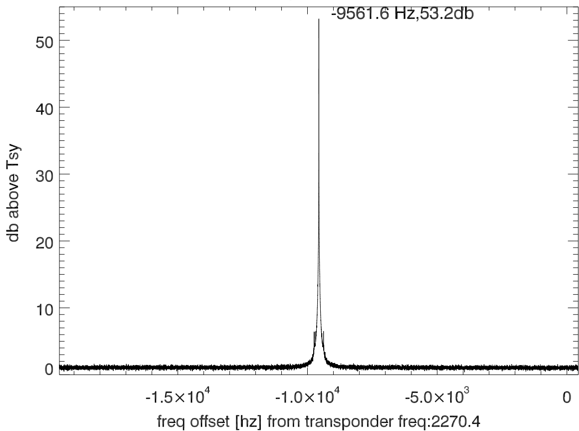
isee3 140608:203241 (UTC) spectra after doppler correction. PolB
