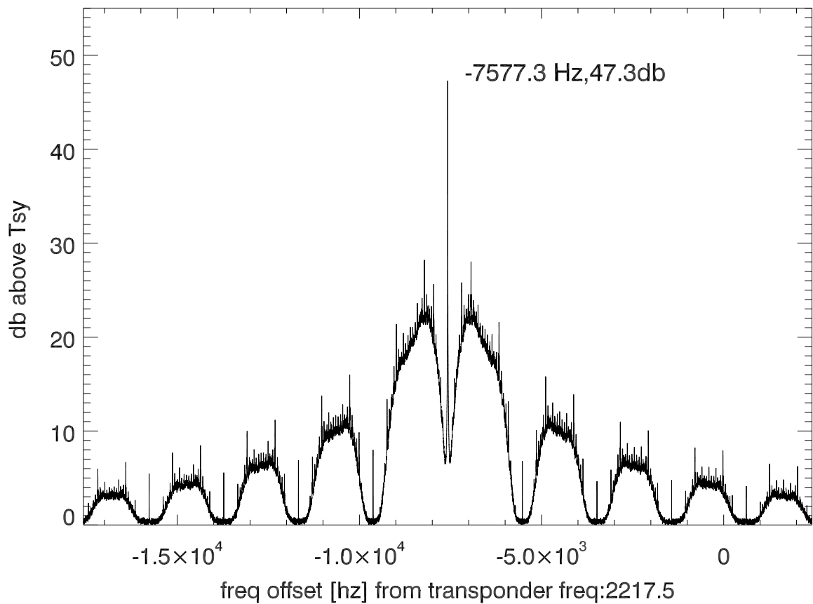
isee3 140608:203241 (UTC) spectra after doppler correction. PoIB
