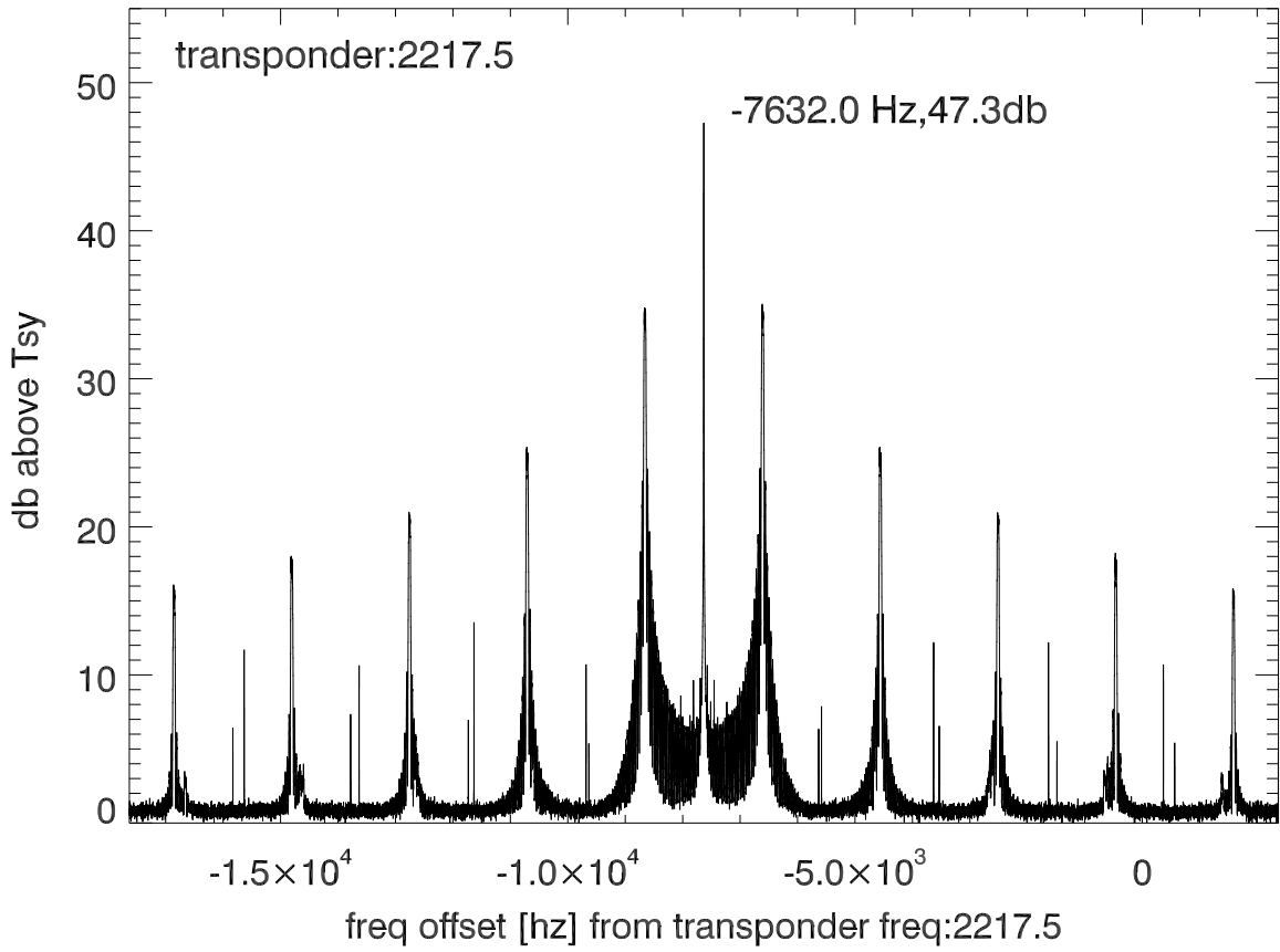
isee3 140606:194126 (UTC) spectra after doppler correction. PolA
