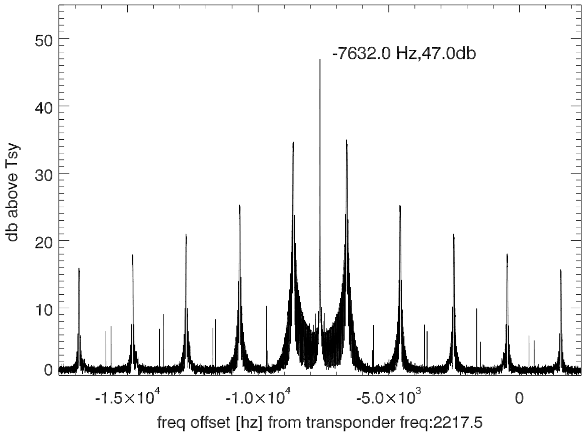
isee3 140606:194126 (UTC) spectra after doppler correction. PolB
