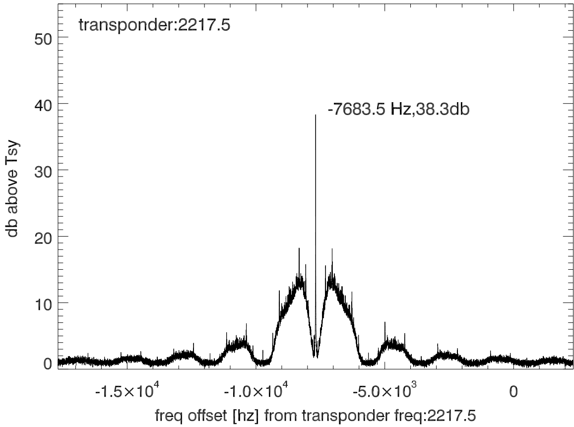
isee3 140604:203629 (UTC) spectra after doppler correction. PoIA
