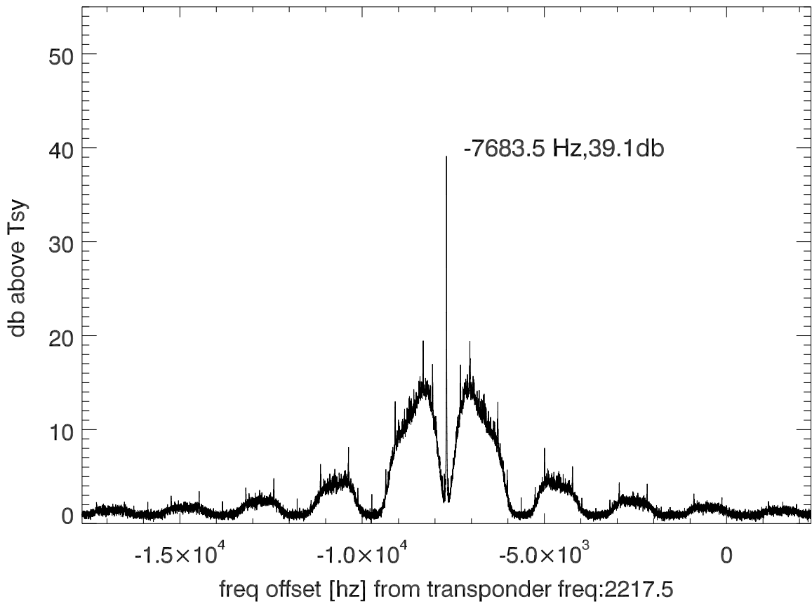
isee3 140604:203629 (UTC) spectra after doppler correction. PoIB
