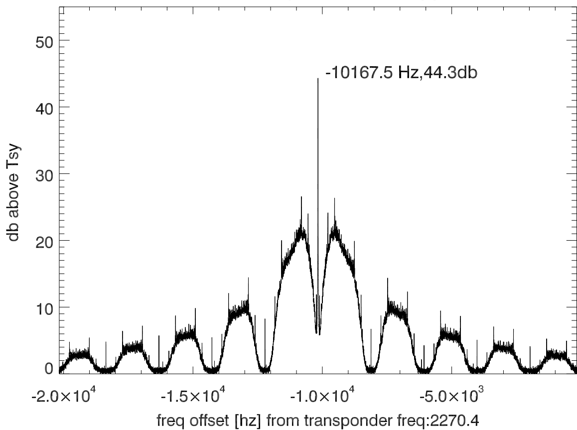
isee3 140530:204621 (UTC) spectra after doppler correction. PoIB
