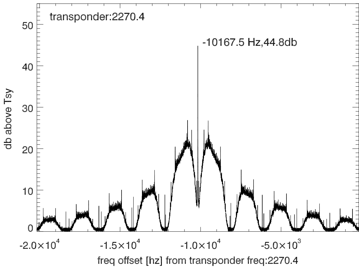
isee3 140530:204621 (UTC) spectra after doppler correction. PoIA
