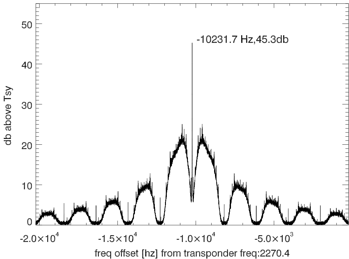
isee3 140529:202021 (UTC) spectra after doppler correction. PoIB
