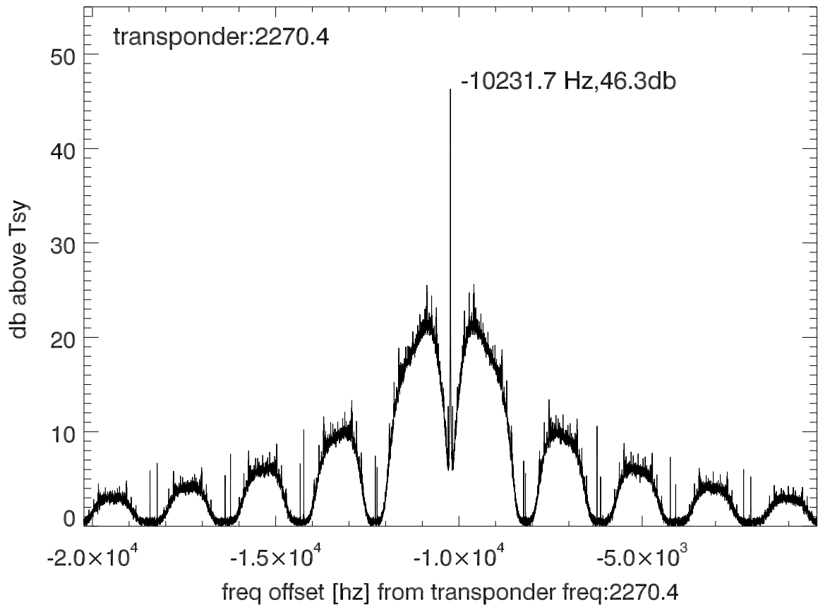
isee3 140529:202021 (UTC) spectra after doppler correction. PoIA
