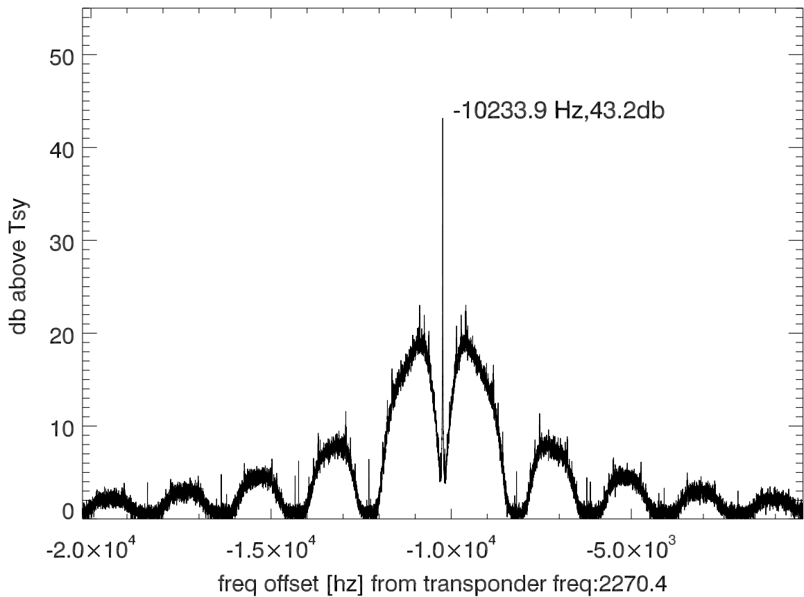
isee3 140529:190756 (UTC) spectra after doppler correction. PolB
