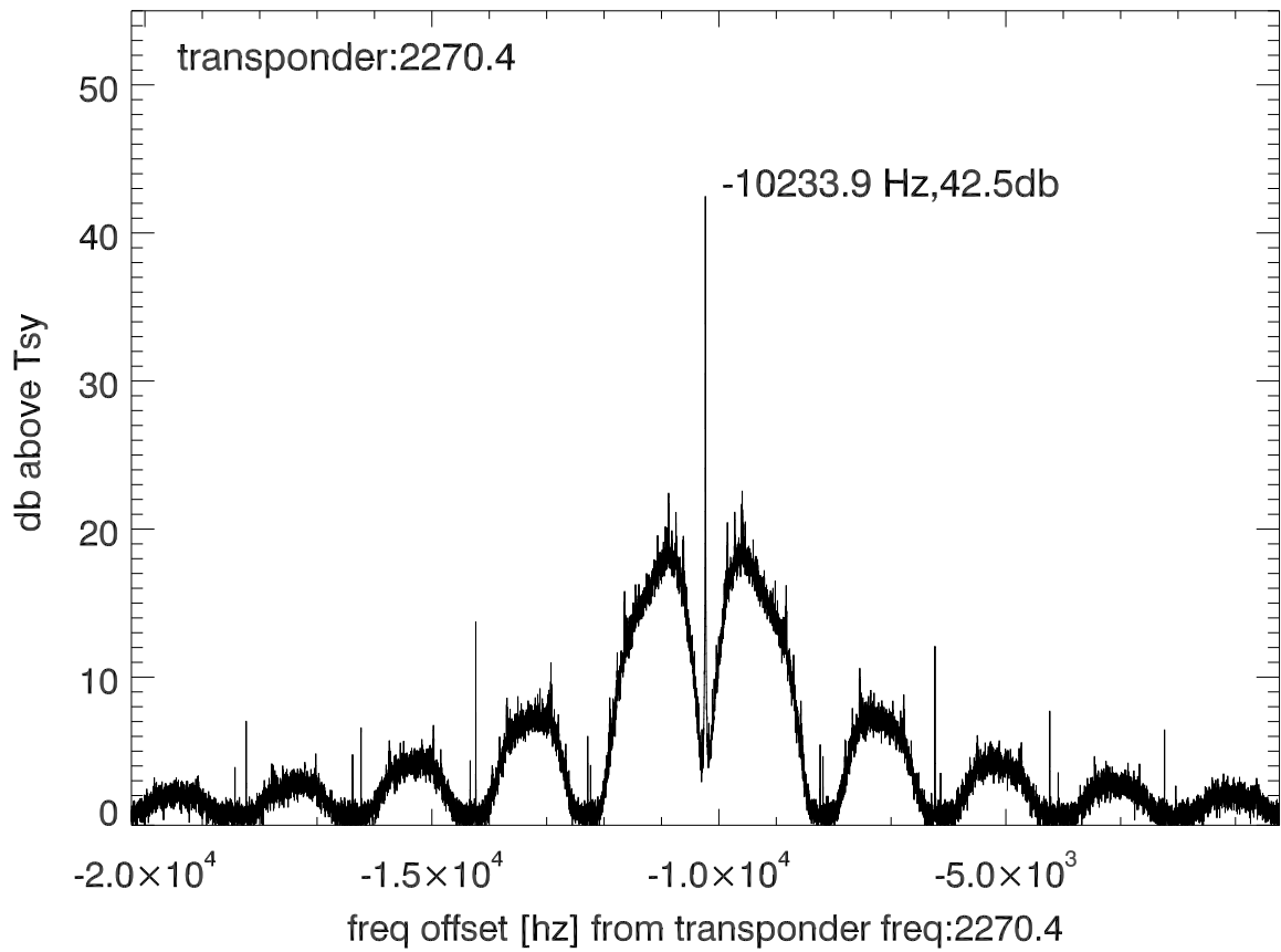
isee3 140529:190756 (UTC) spectra after doppler correction. PolA
