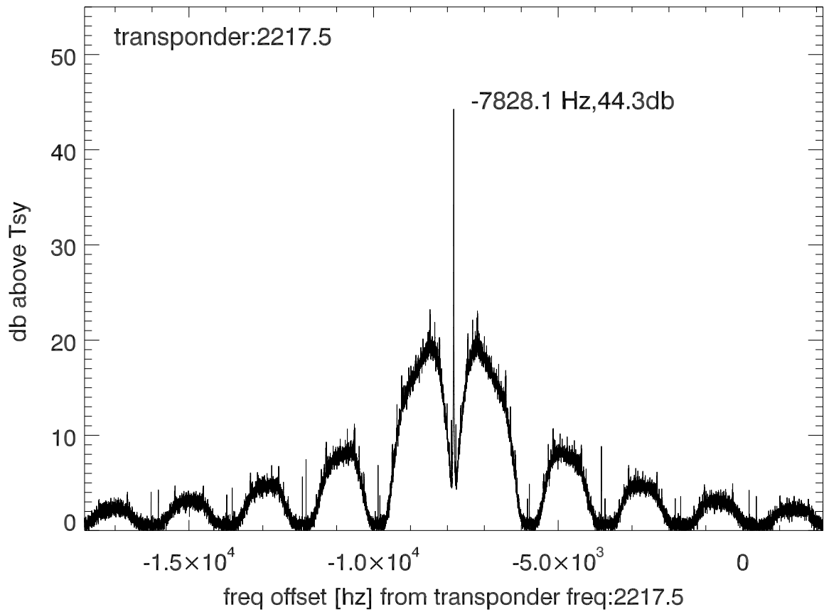
isee3 140529:204102 (UTC) spectra after doppler correction. PolA
