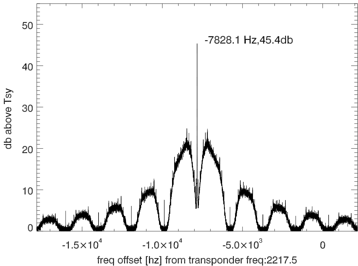
isee3 140529:204102 (UTC) spectra after doppler correction. PolB
