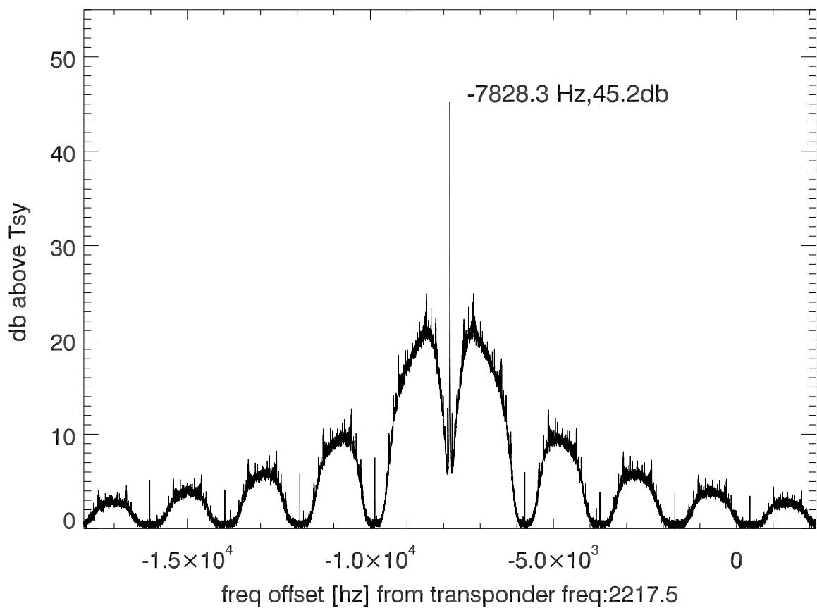
isee3 140529:203235 (UTC) spectra after doppler correction. PoIB
