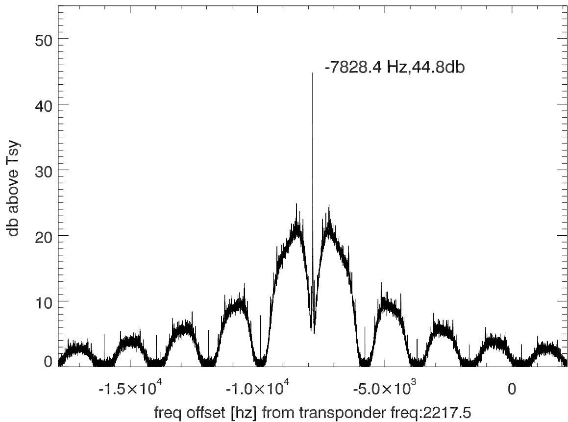
isee3 140529:202605 (UTC) spectra after doppler correction. PoIB
