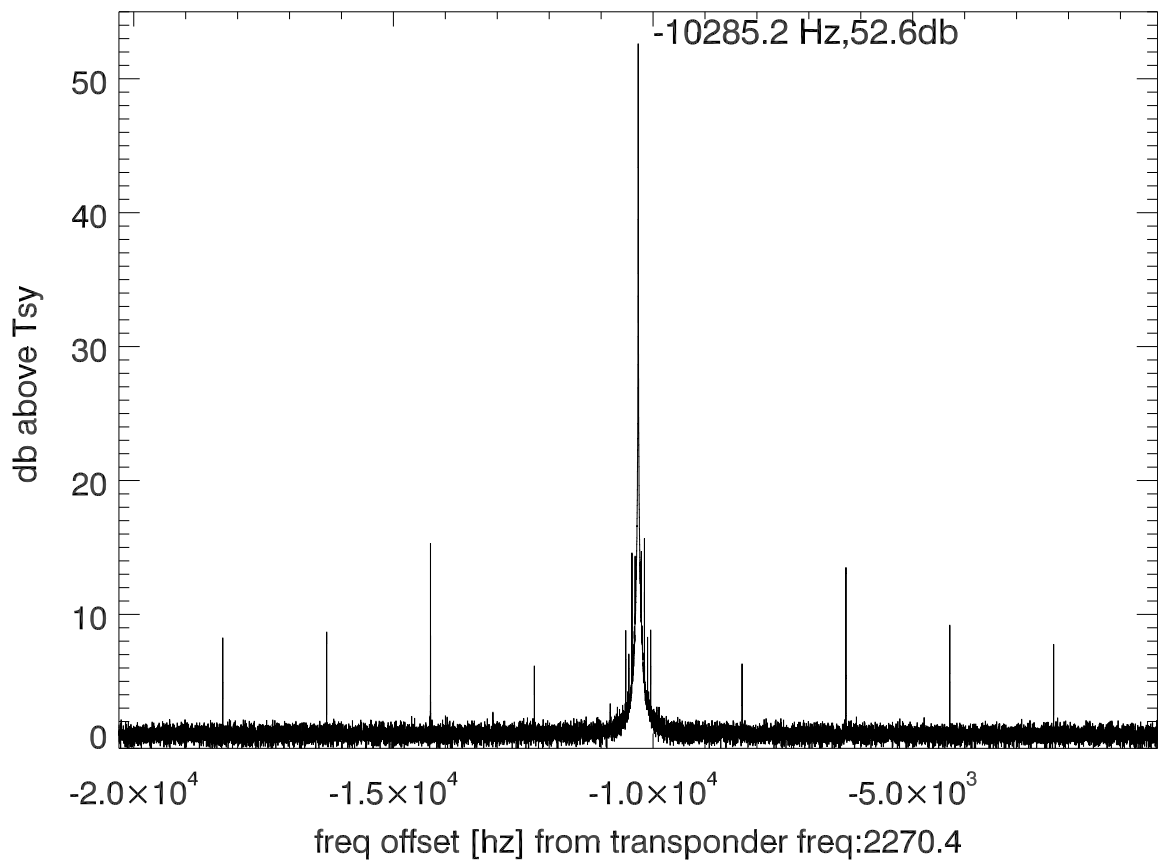
isee3 140528:192603 (UTC) spectra after doppler correction. PoIB
