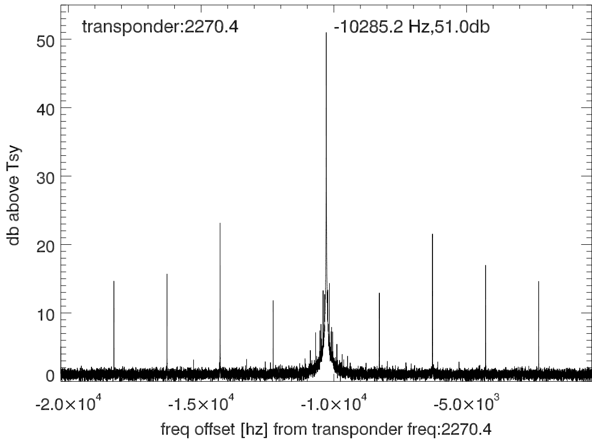
isee3 140528:192603 (UTC) spectra after doppler correction. PoIA
