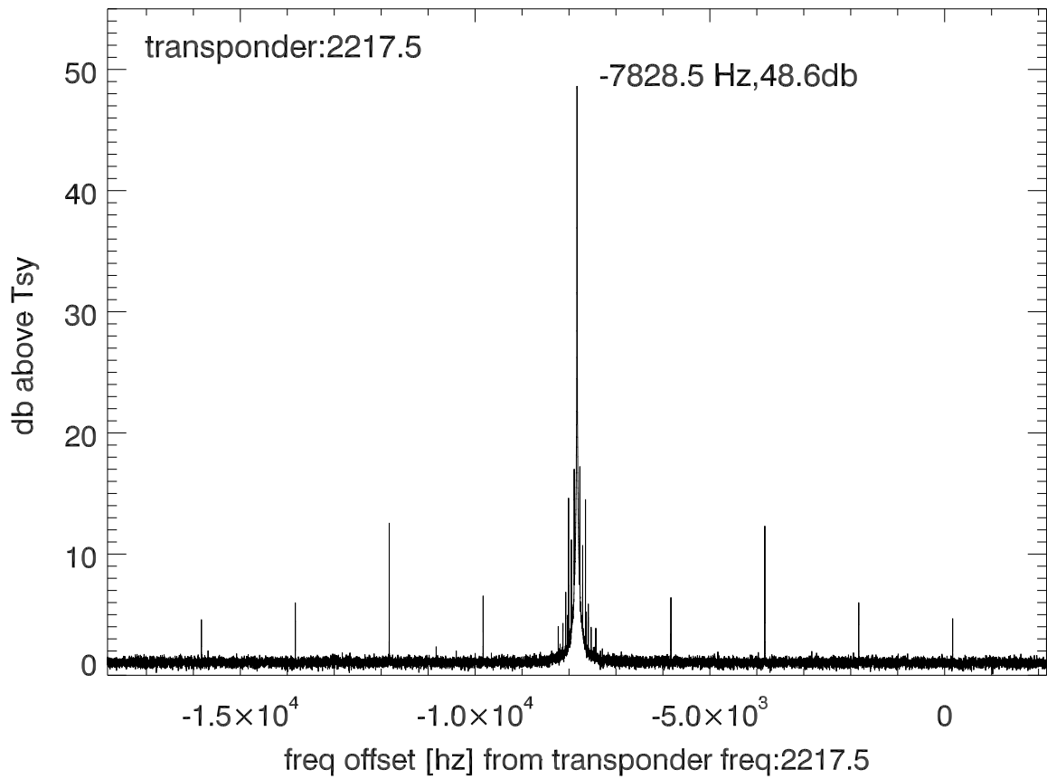
isee3 140528:205204 (UTC) spectra after doppler correction. PolA
