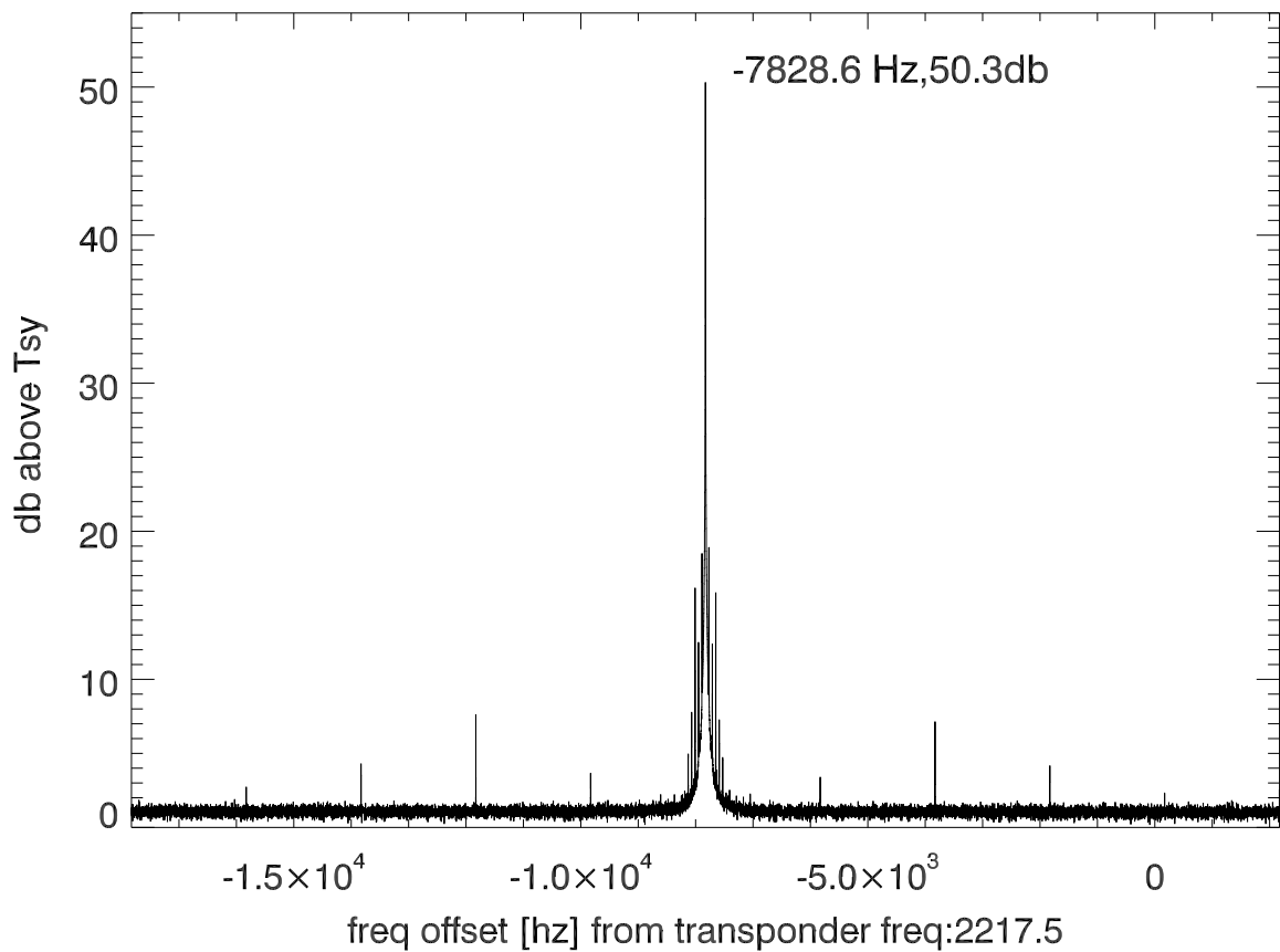
isee3 140528:205204 (UTC) spectra after doppler correction. PolB
