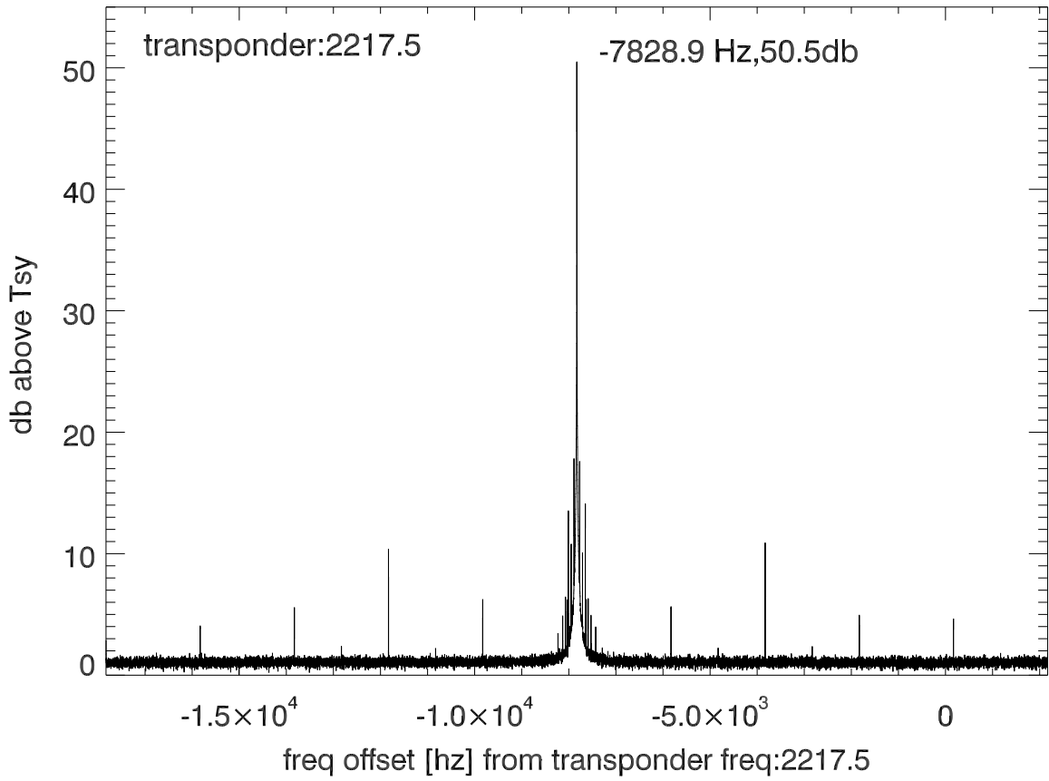
isee3 140528:204658 (UTC) spectra after doppler correction. PolA
