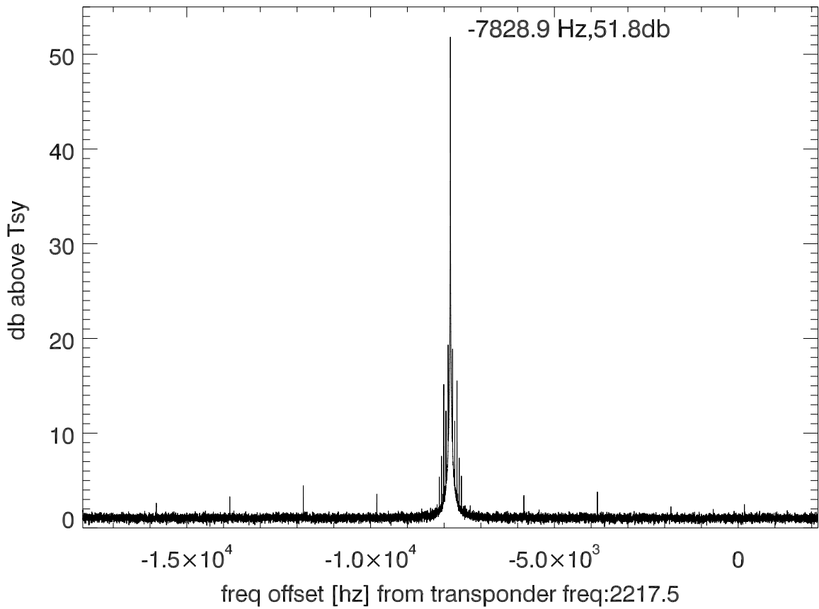
isee3 140528:204658 (UTC) spectra after doppler correction. PolB
