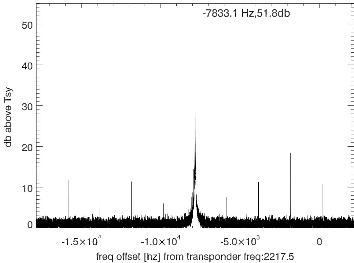
isee3 140528:193708 (UTC) spectra after doppler correction. PolB
