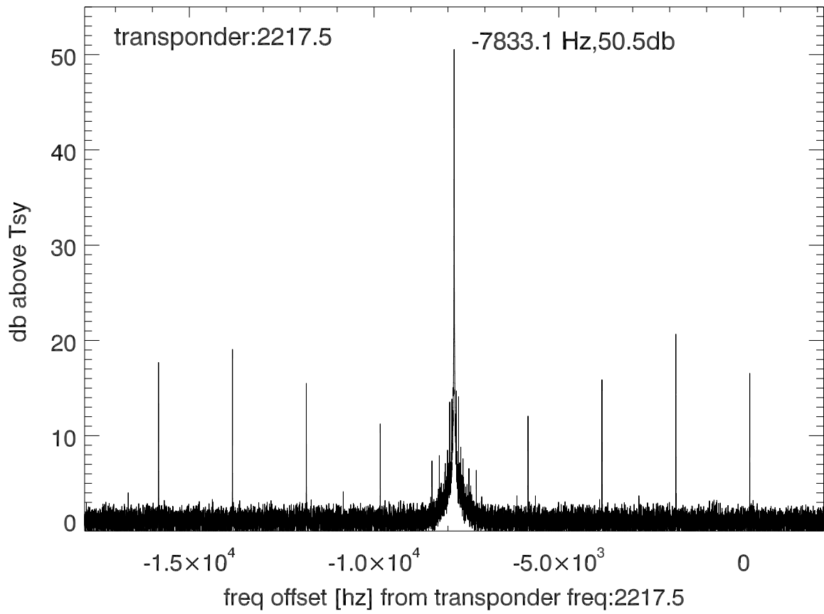
isee3 140528:193708 (UTC) spectra after doppler correction. PolA
