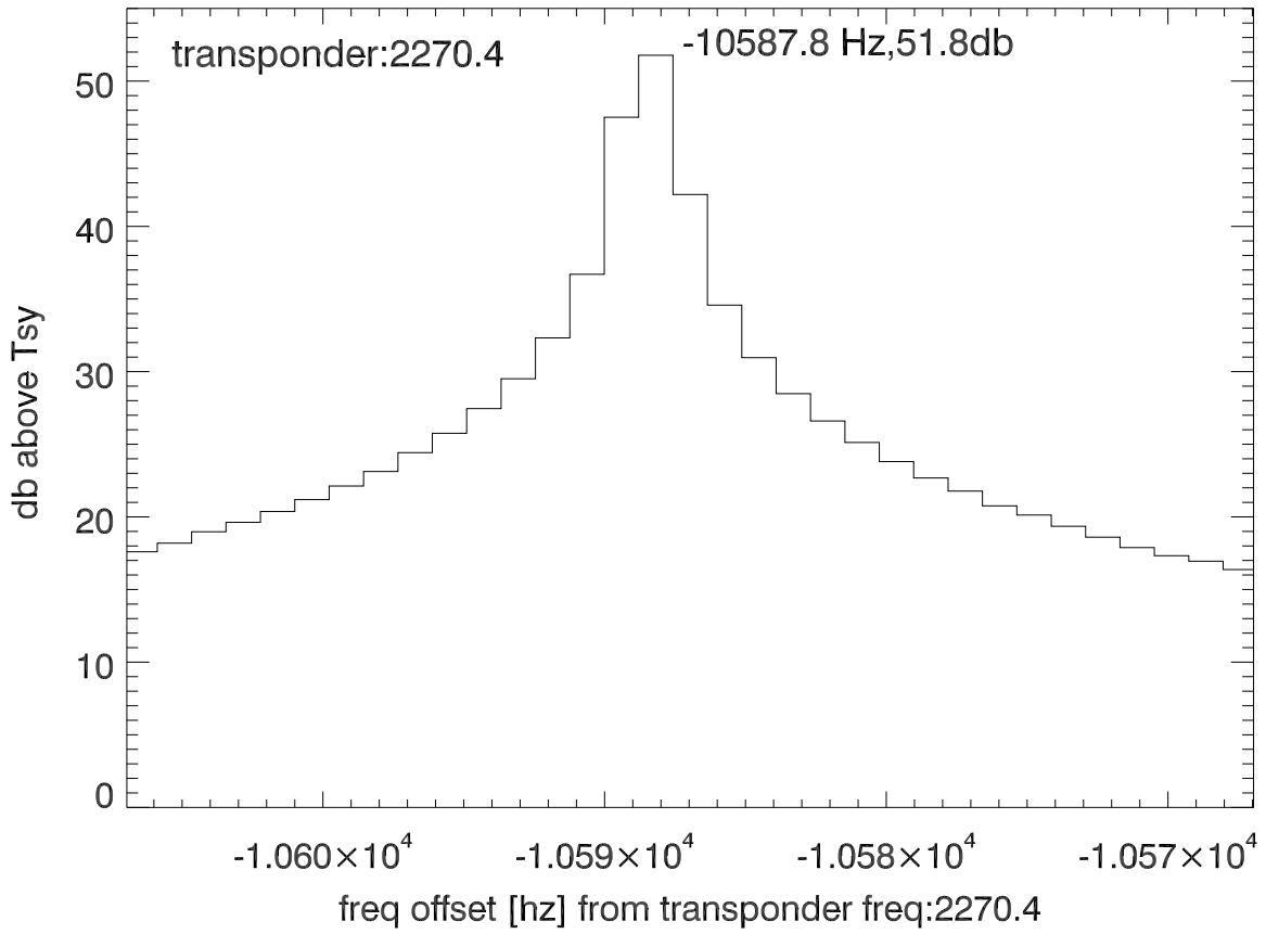
isee3 140523:203835 (UTC) spectra after doppler correction. PolA
