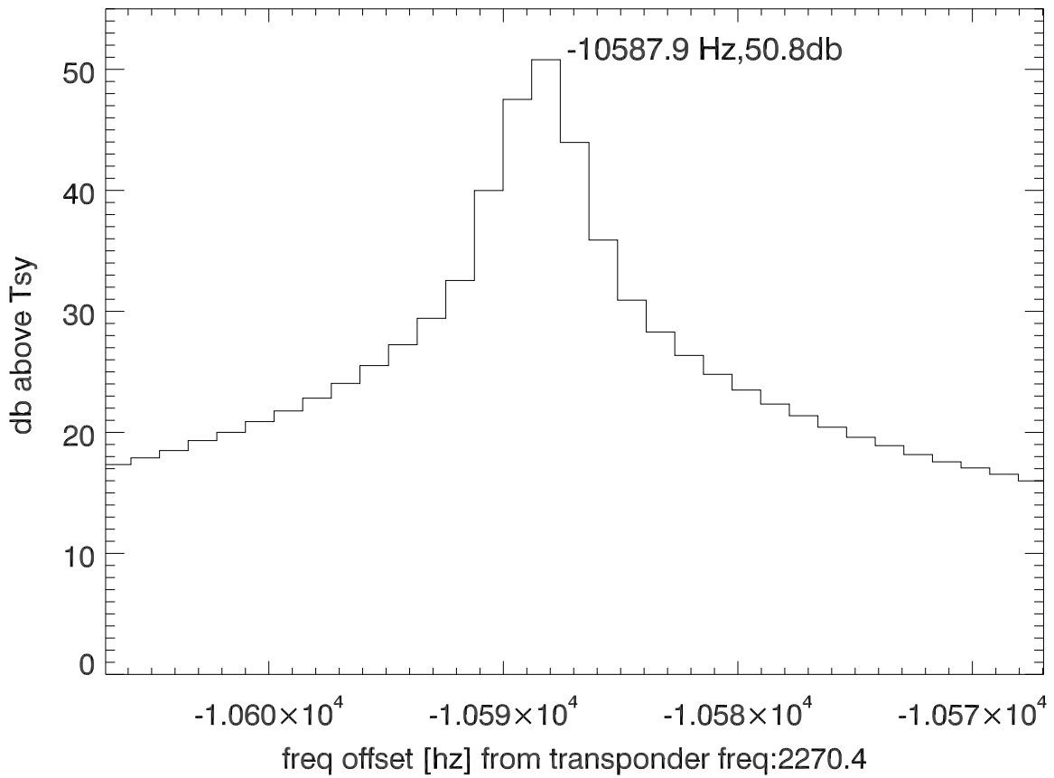
isee3 140523:203835 (UTC) spectra after doppler correction. PolB
