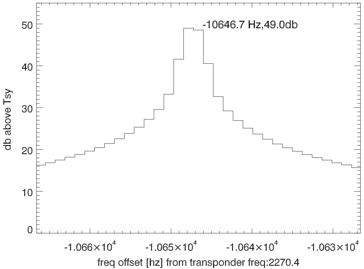
isee3 140522:205851 (UTC) spectra after doppler correction. PolB
