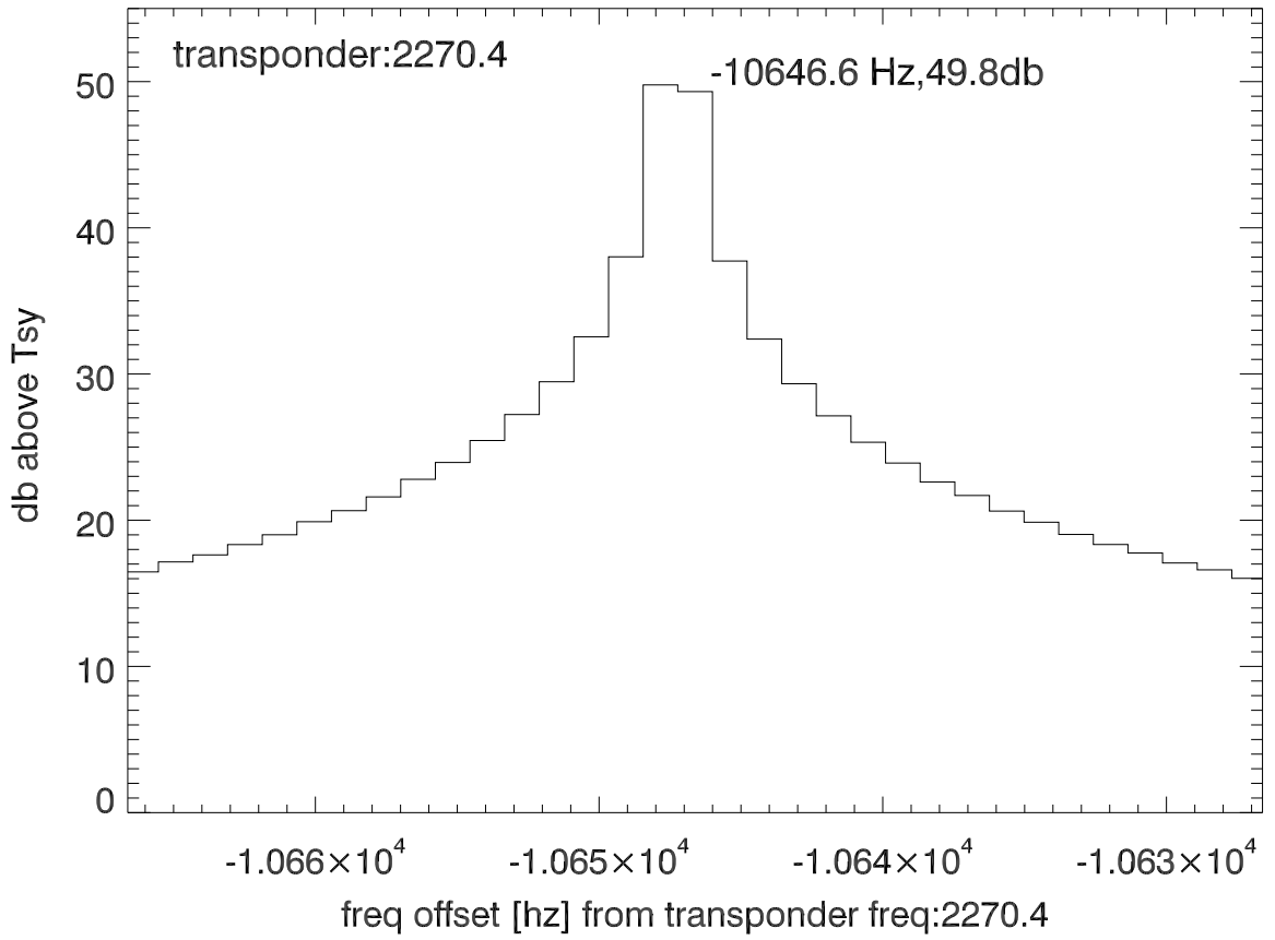
isee3 140522:205851 (UTC) spectra after doppler correction. PolA
