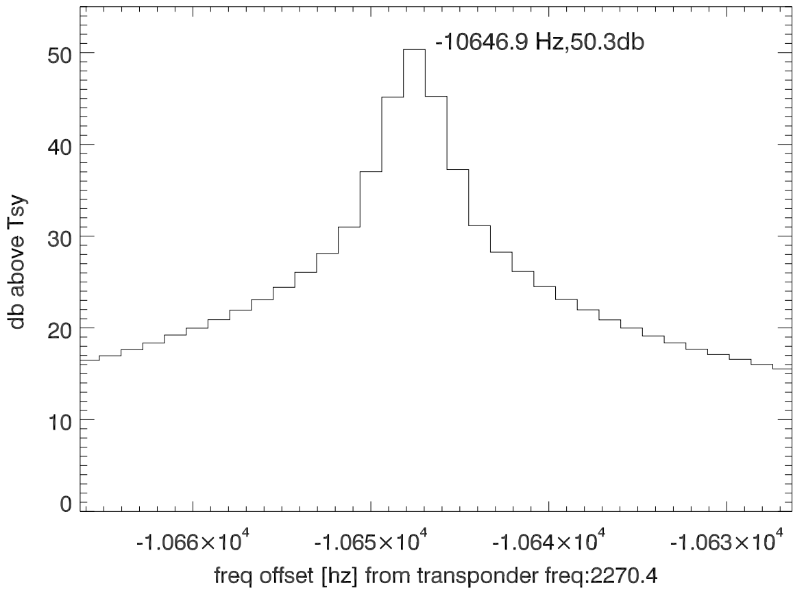
isee3 140522:205129 (UTC) spectra after doppler correction. PolB
