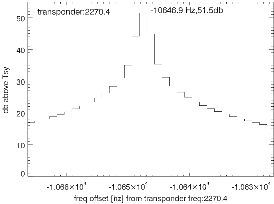
isee3 140522:205129 (UTC) spectra after doppler correction. PolA
