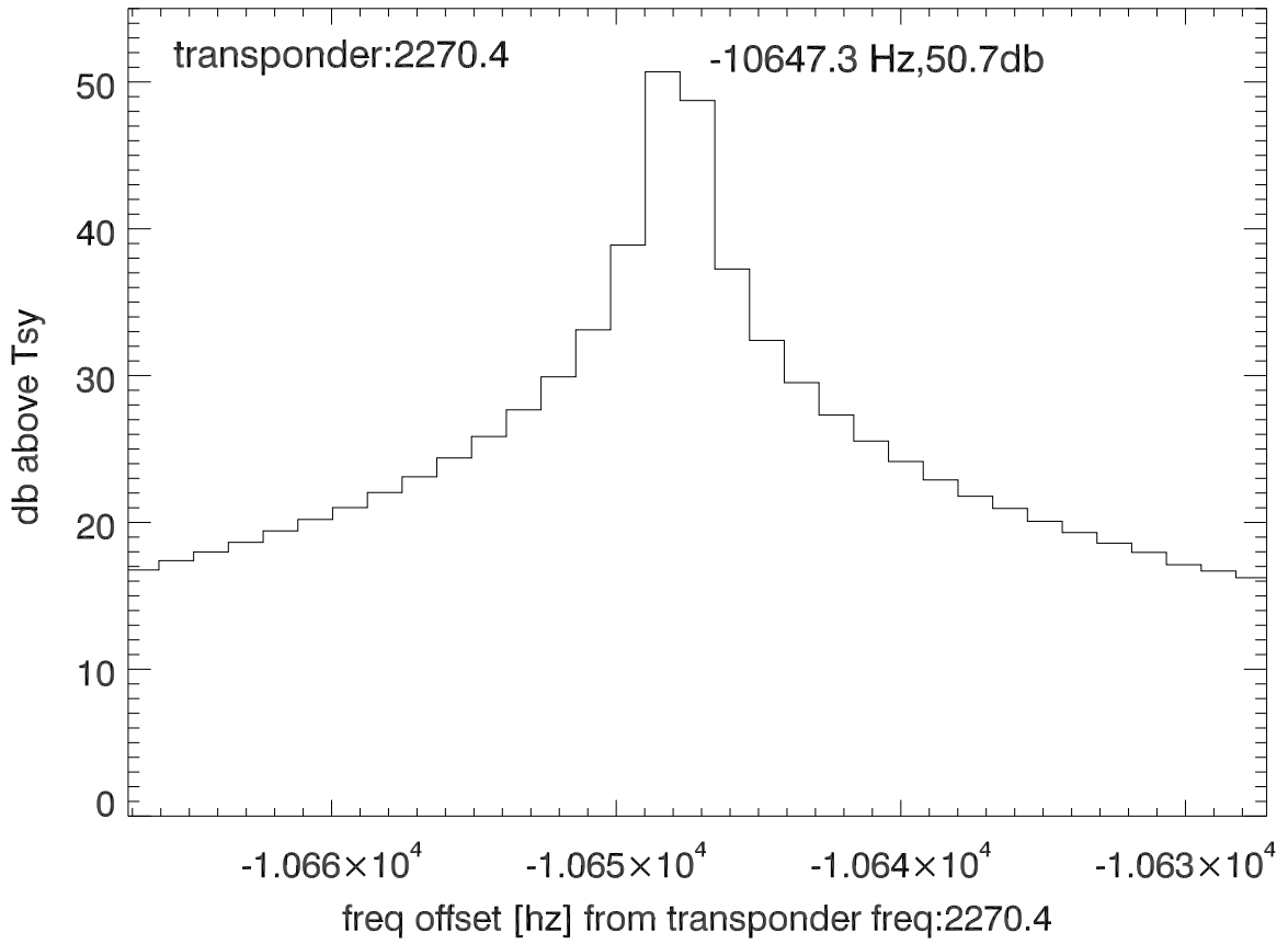
isee3 140522:204422 (UTC) spectra after doppler correction. PolA
