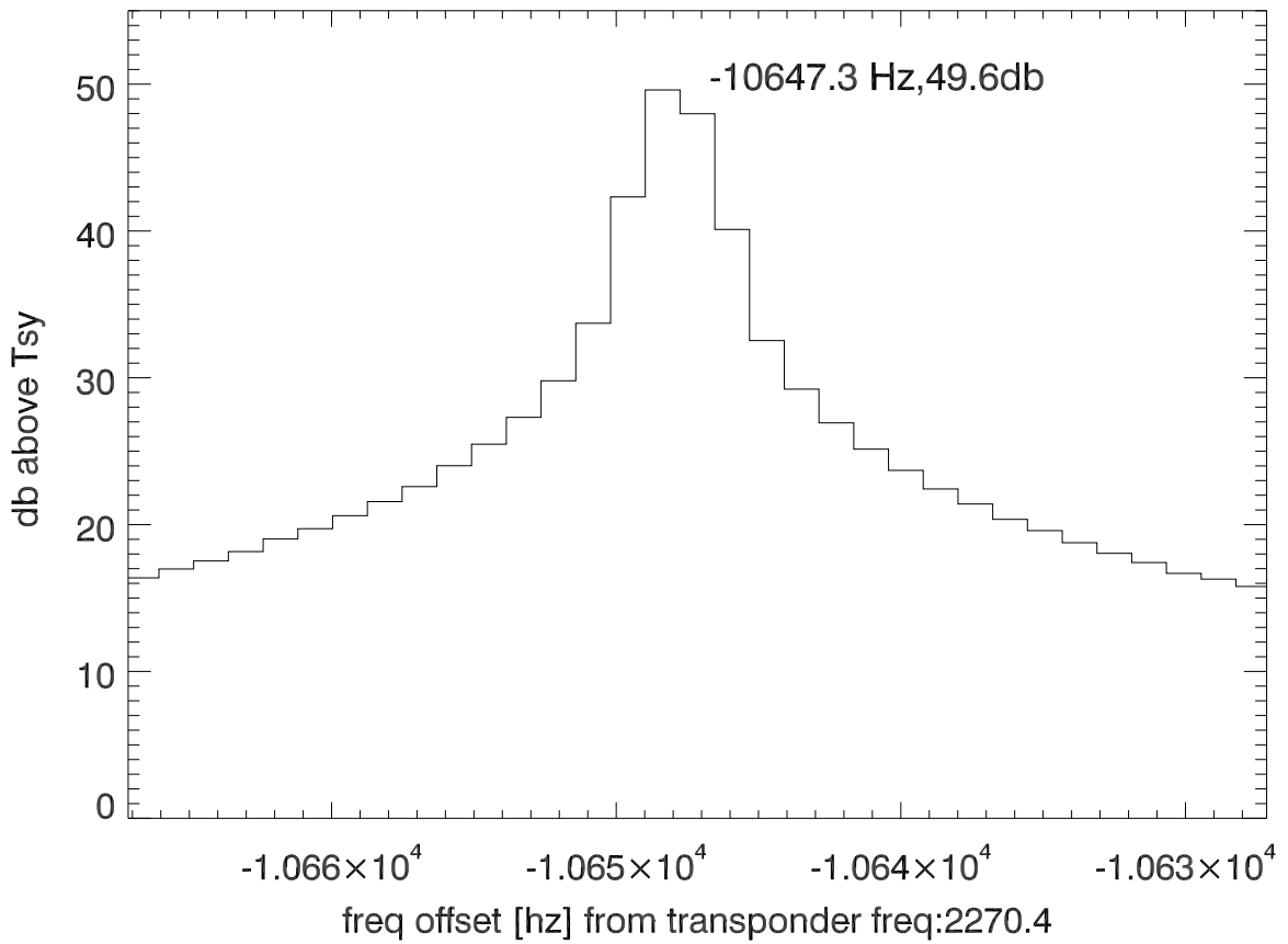
isee3 140522:204422 (UTC) spectra after doppler correction. PolB
