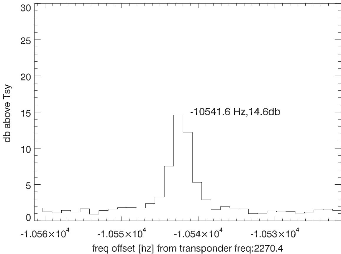
isee3 140409:194957 (UTC) spectra after doppler correction. PoIB
