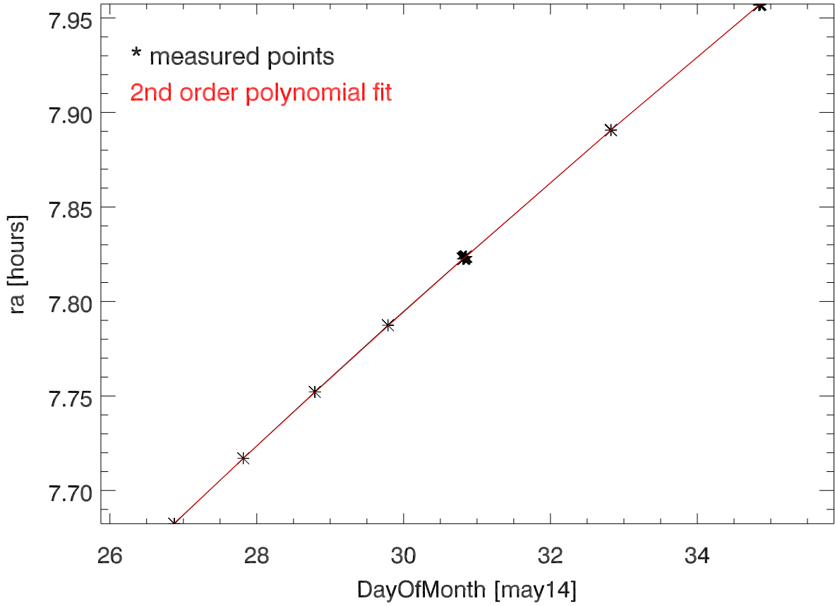
isee3 measured positions J2000. RA
