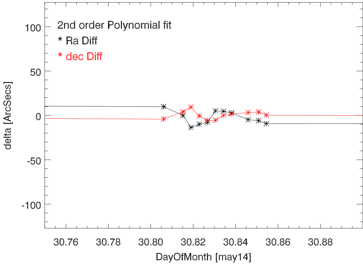
Measured - Fit positions(J2000)
