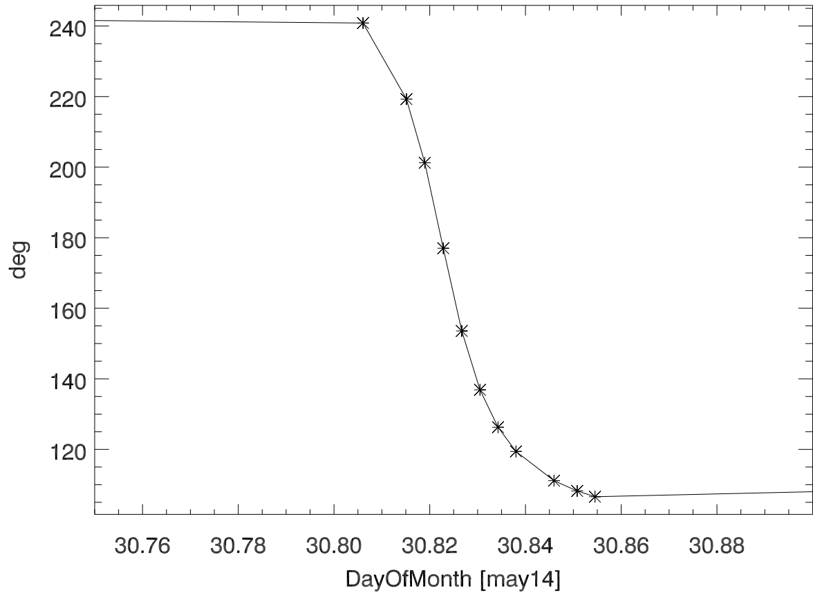
azimuth center of patterns
