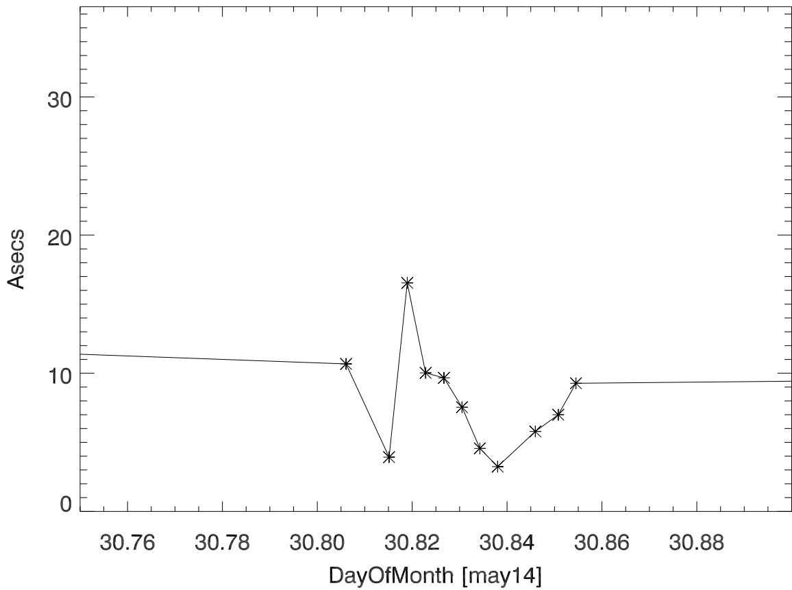
Add ra,dec errors in quadrature
