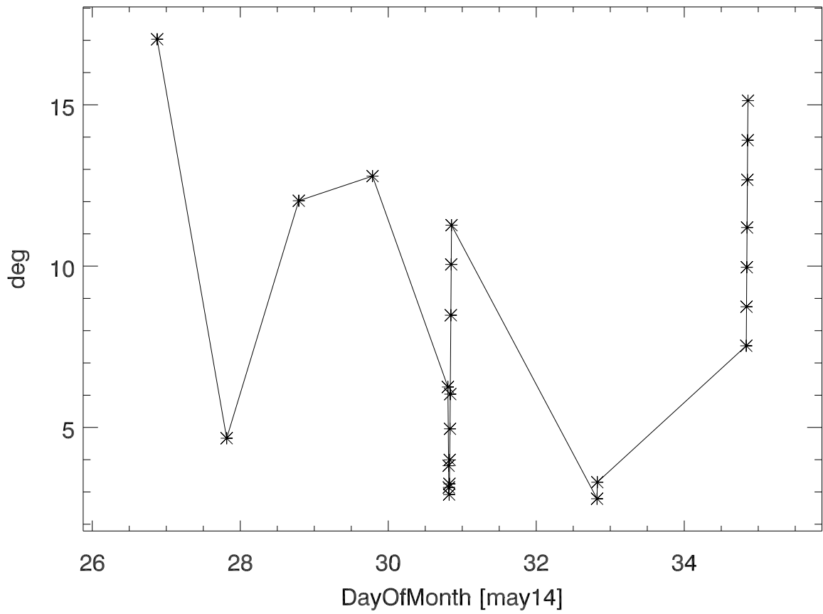
za center of patterns
