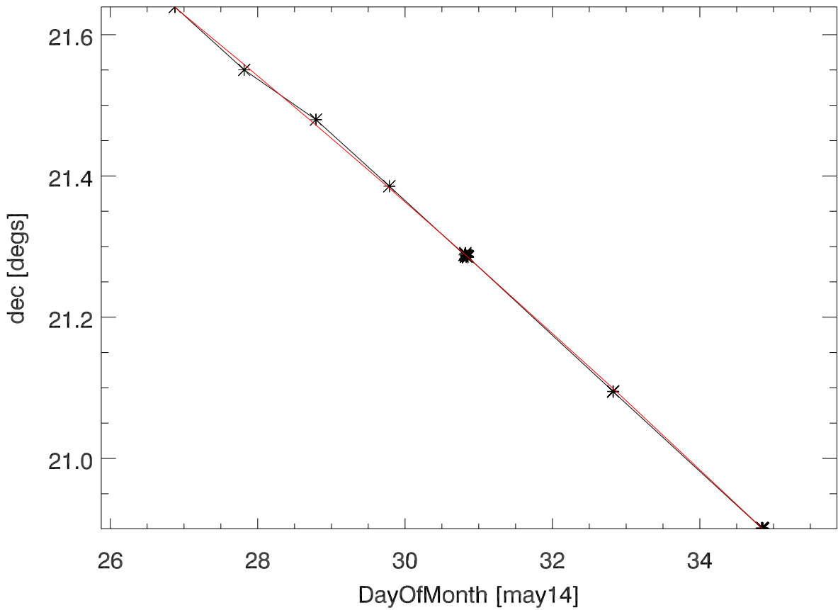
decPosition (J2000) [deg]
