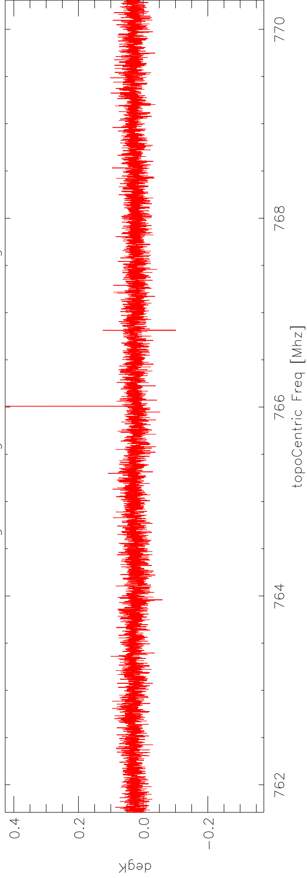
a2621 data averaged through 01nov11TMC-1 avg:0.03 rms:0.02
