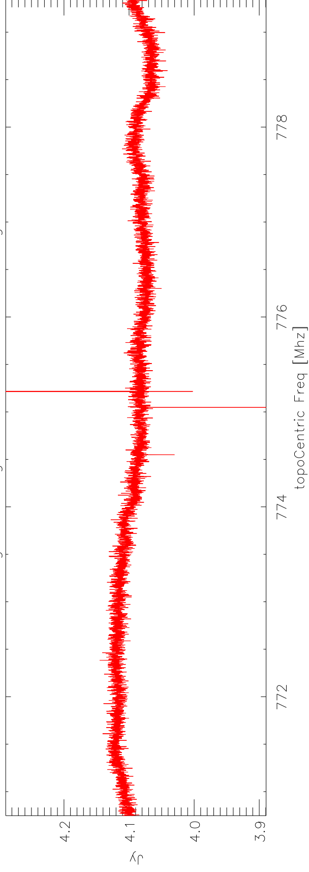
a2621 data averaged through 01nov11IC-443-G1 avg:4.09 rms:0.02
