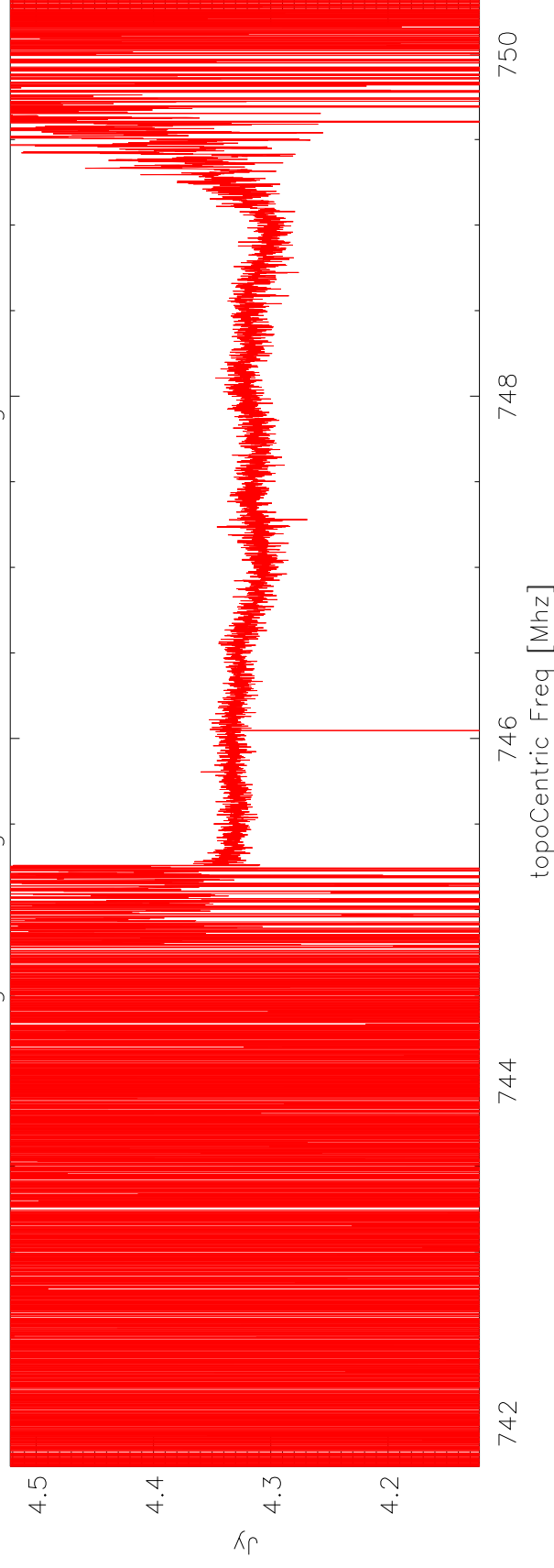
a2621 data averaged through 01nov11IC-443-G1 avg:4.26 rms:2.31
