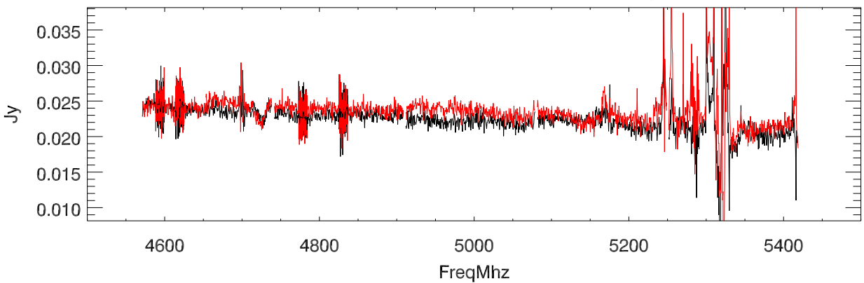
(on/off - 1) :G192.61-0.14 date:20110223 fNum:06000 patNum:15 smo:51
