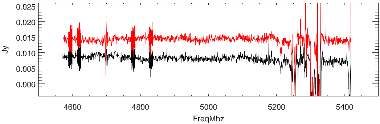
(on/off - 1) :G192.71+0.04 date:20110223 fNum:05200 patNum:13 smo:51
