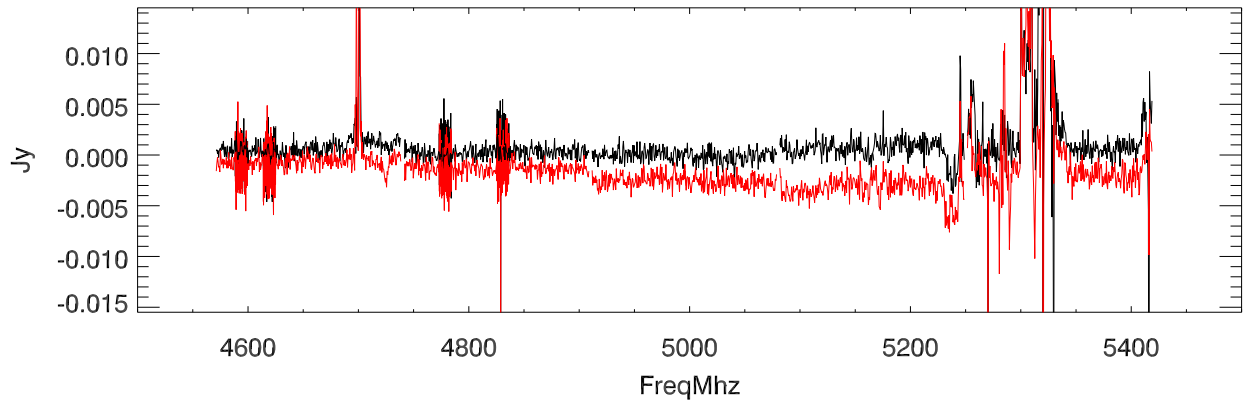
(on/off - 1) :G192.77+0.10 date:20110223 fNum:05600 patNum:14 smo:51
