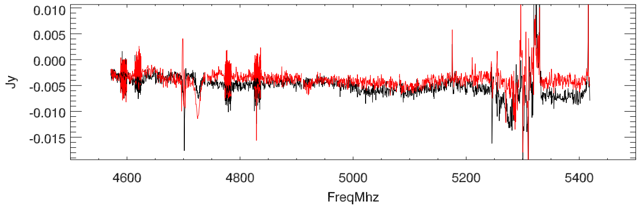
(on/off - 1) :G192.63-0.15 date:20110223 fNum:04800 patNum:12 smo:51
