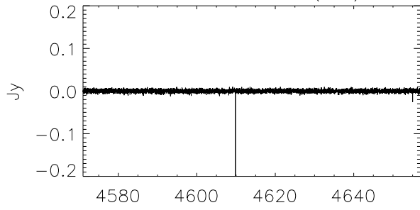
G203.04+1.76 (WB)
