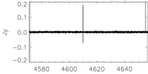
G188.79+1.03 (WB)
