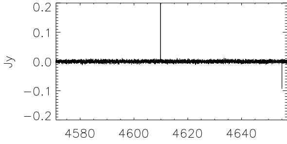
G207.02-1.83 (WB)
