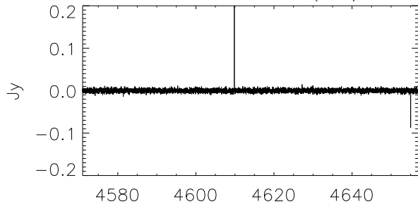
G207.11-1.83 (WB)
