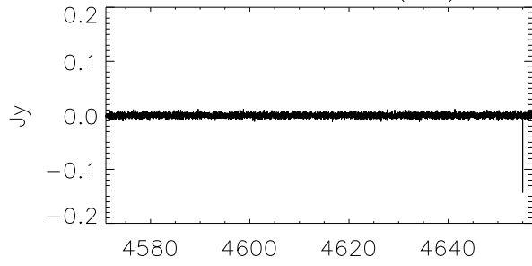
G202.47+2.48 (WB)
