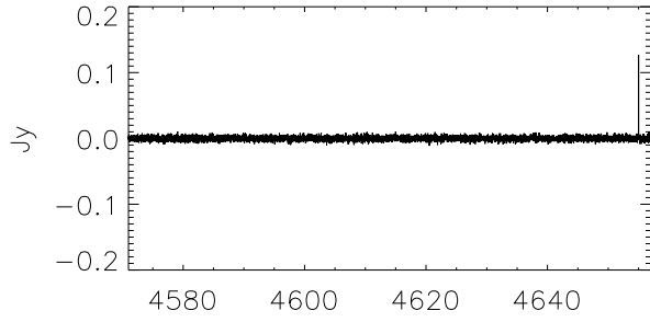
G203.20+2.02 (WB)
