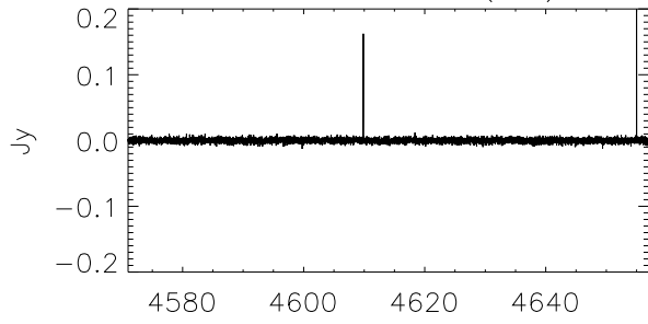
G189.01+0.83 (WB)
