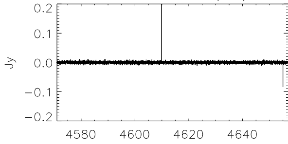
G196.22-1.17 (WB)
