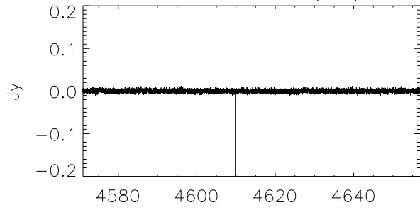
G189.68+0.19 (WB)
