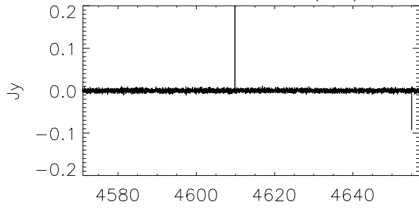
G189.06+1.07 (WB)
