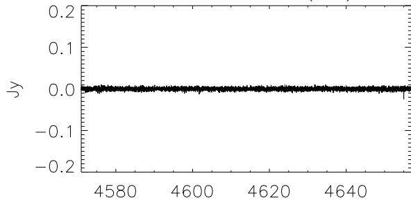
G202.91+2.11 (WB)
