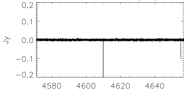
G189.03+0.78 (WB)
