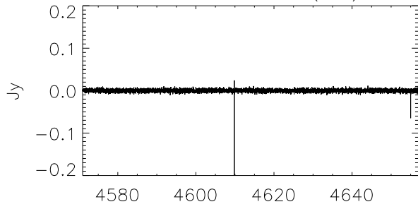
G189.03+0.81 (WB)
