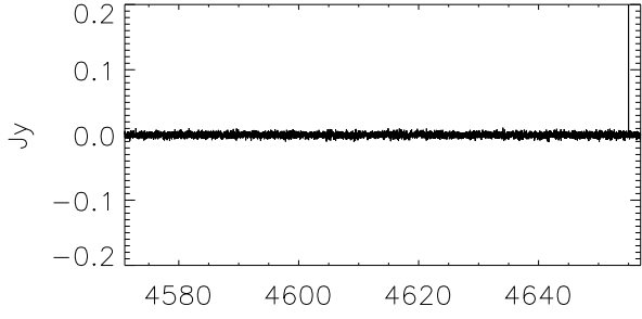
G203.22+2.09 (WB)
