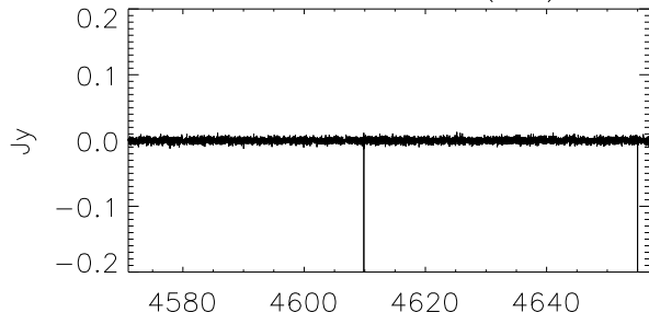
G183.40-0.56 (WB)
