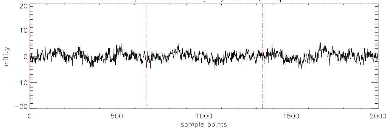
a2471 epsTau 20dec10 (AST) StokesQ freq:5176.
