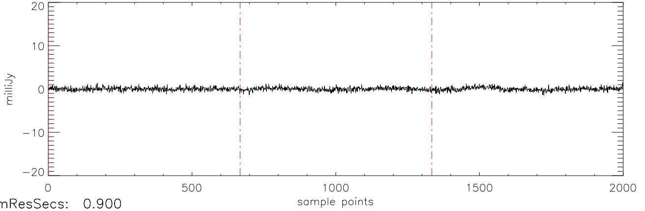
a2471 epsTau 20dec10 (AST) StokesV freq:5034.
