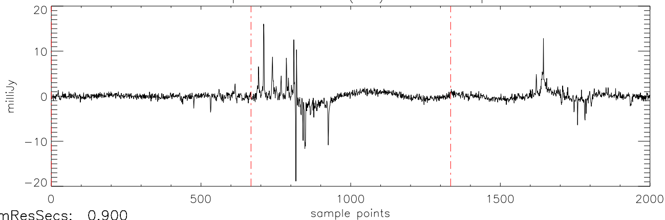
a2471 epsTau 20dec10 (AST) StokesU freq:4466.
