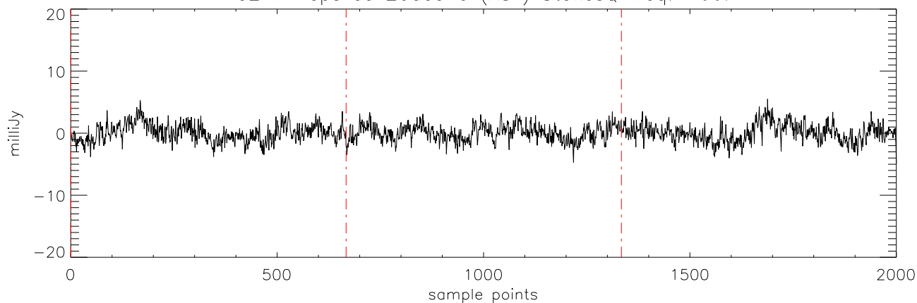
a2471 epsTau 20dec10 (AST) StokesQ freq:4608.
