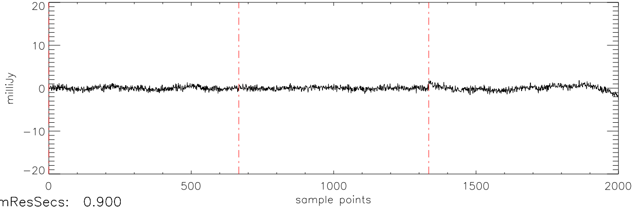
a2471 epsTau 20dec10 (AST) StokesU freq:5034.
