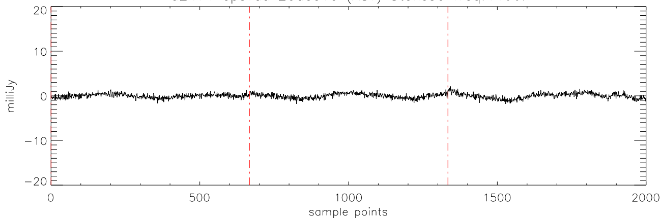
a2471 epsTau 20dec10 (AST) StokesU freq:4608.
