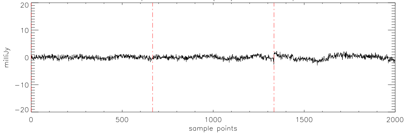
a2471 epsTau 20dec10 (AST) StokesU freq:5176.
