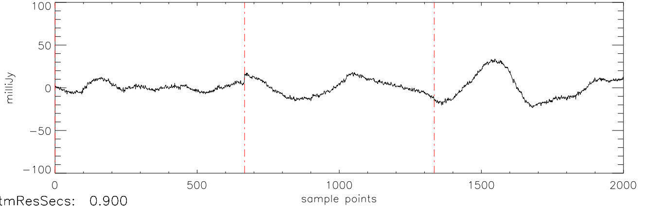
a2471 epsTau 20dec10 (AST) StokesI freq:5034.
