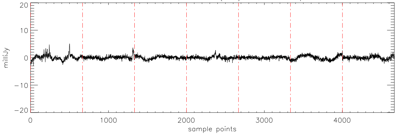
a2471 TVLM-513 31mar12 (AST) StokesU freq:4608.
