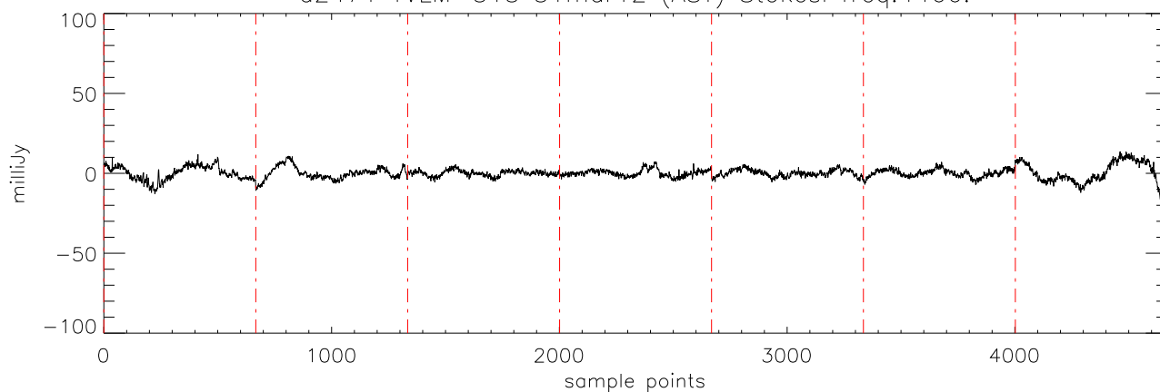
a2471 TVLM-513 31mar12 (AST) StokesI freq:4608.
