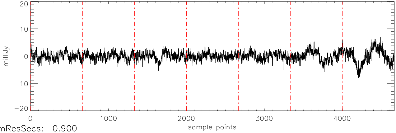
a2471 TVLM-513 31mar12 (AST) StokesQ freq:5034.
