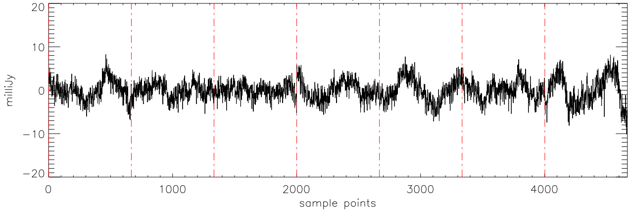
a2471 TVLM-513 31mar12 (AST) StokesQ freq:5176.
