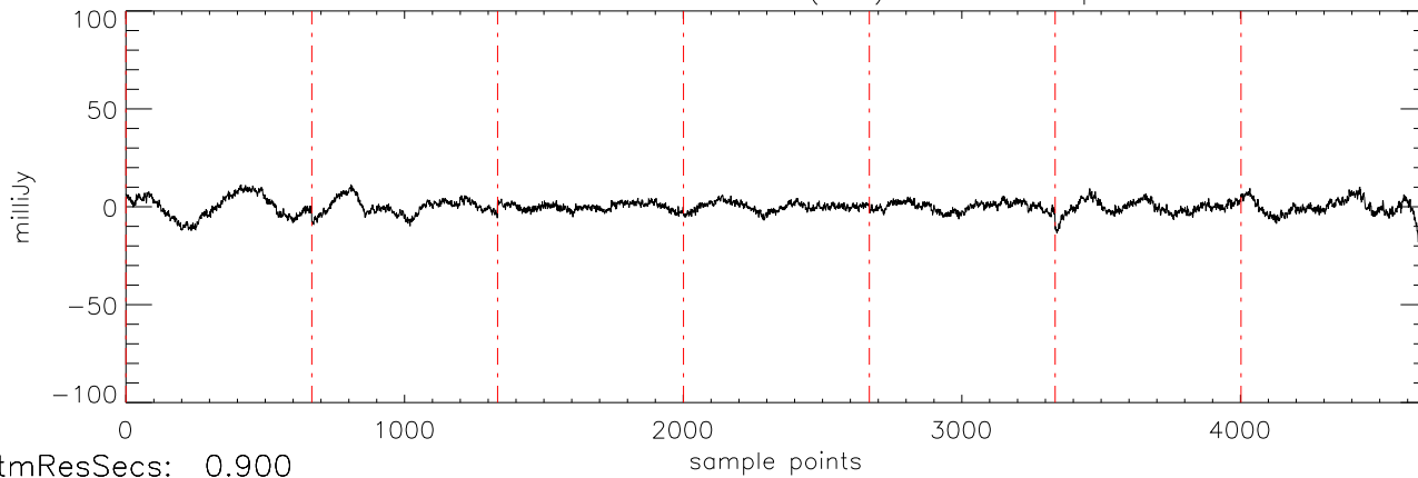
a2471 TVLM-513 31mar12 (AST) StokesI freq:5034.
