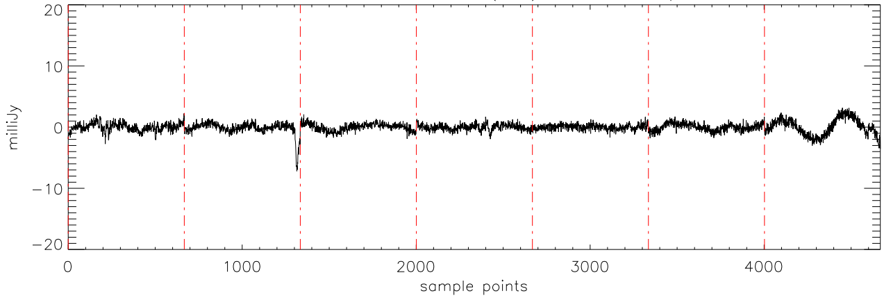
a2471 TVLM-513 31mar12 (AST) StokesU freq:4750.
