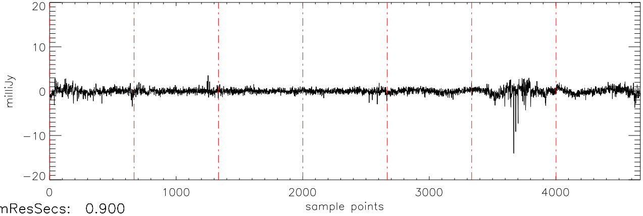
a2471 TVLM-513 31mar12 (AST) StokesV freq:4466.
