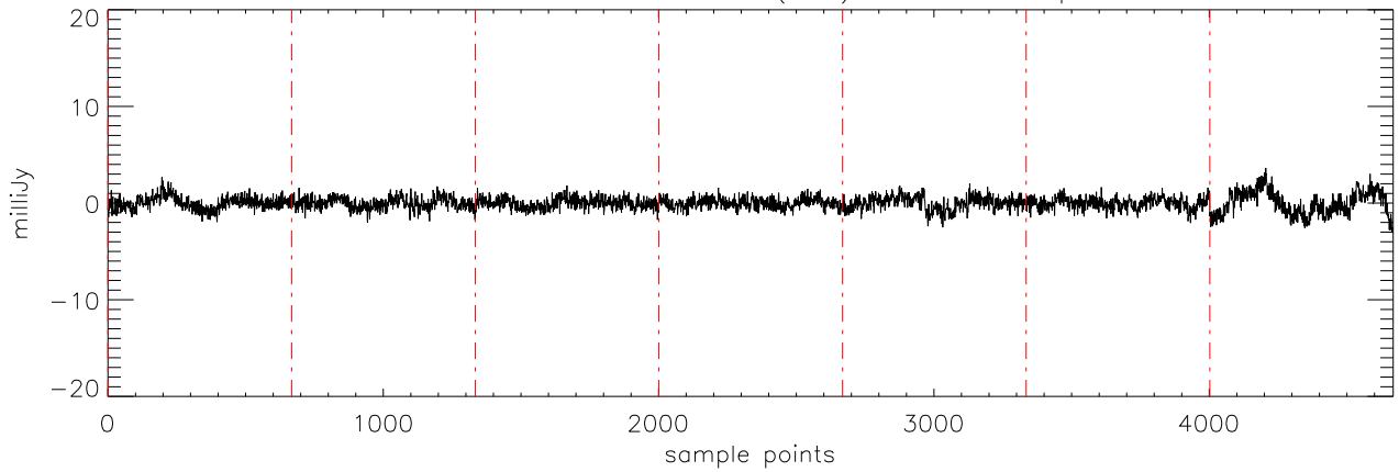
a2471 TVLM-513 31mar12 (AST) StokesU freq:5176.
