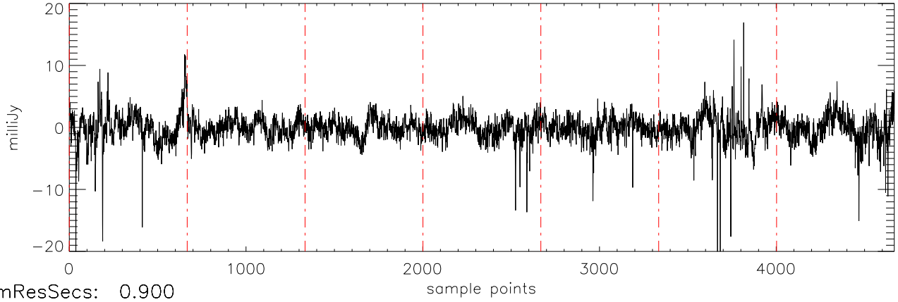
a2471 TVLM-513 31mar12 (AST) StokesQ freq:4466.
