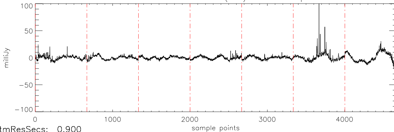
a2471 TVLM-513 31mar12 (AST) StokesI freq:4466.
