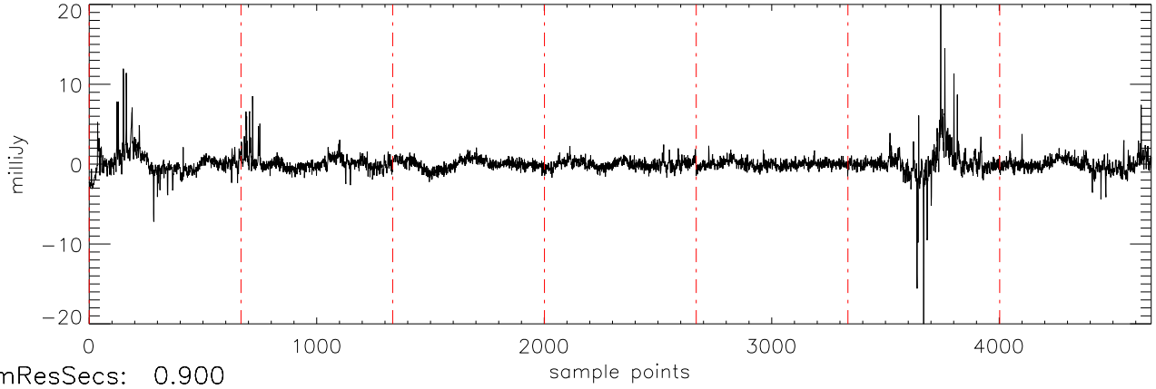
a2471 TVLM-513 31mar12 (AST) StokesU freq:4466.
