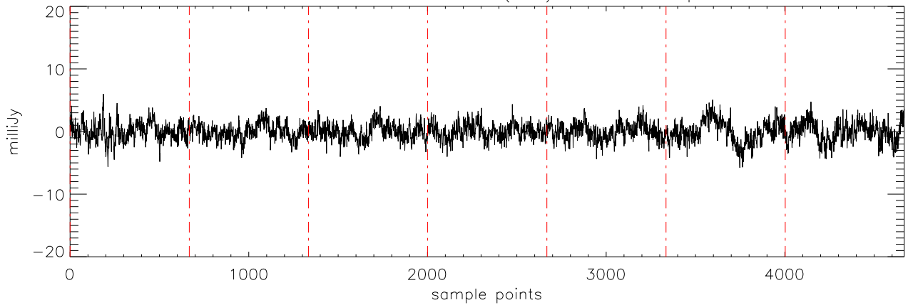
a2471 TVLM-513 31mar12 (AST) StokesQ freq:4750.
