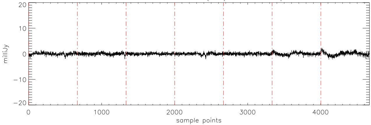
a2471 TVLM-513 31mar12 (AST) StokesV freq:4608.
