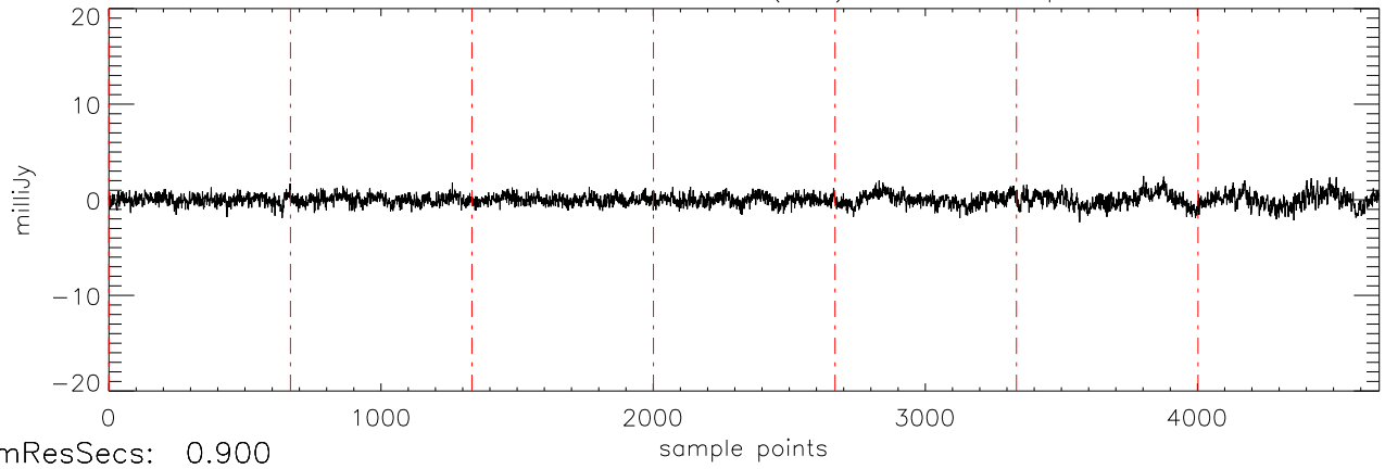
a2471 TVLM-513 31mar12 (AST) StokesV freq:5034.
