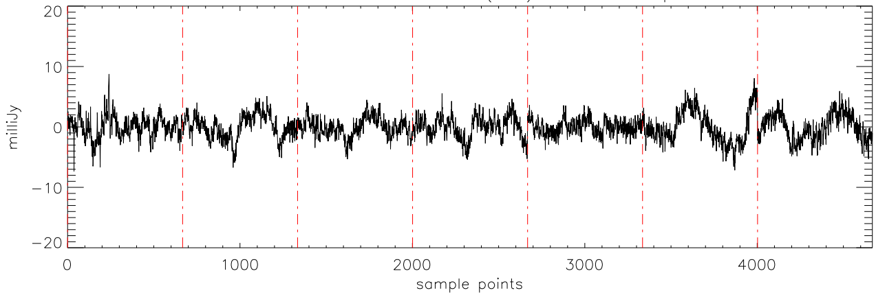
a2471 TVLM-513 31mar12 (AST) StokesQ freq:4608.
