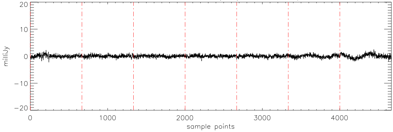
a2471 TVLM-513 31mar12 (AST) StokesV freq:4750.
