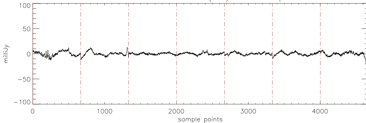
a2471 TVLM-513 31mar12 (AST) StokesI freq:4750.
