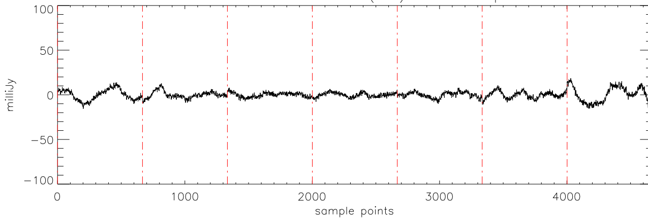
a2471 TVLM-513 31mar12 (AST) StokesI freq:5176.
