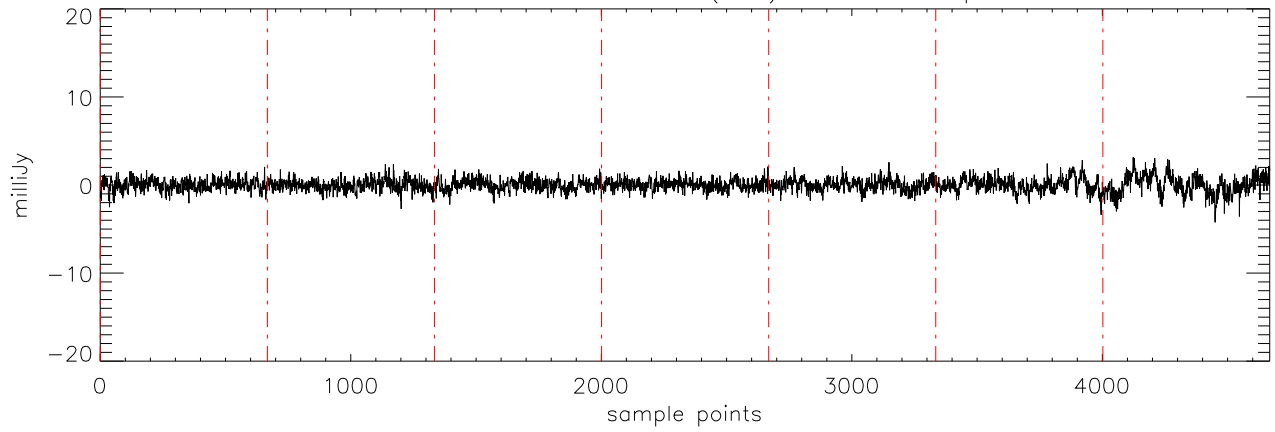
a2471 TVLM-513 31mar12 (AST) StokesV freq:5176.
