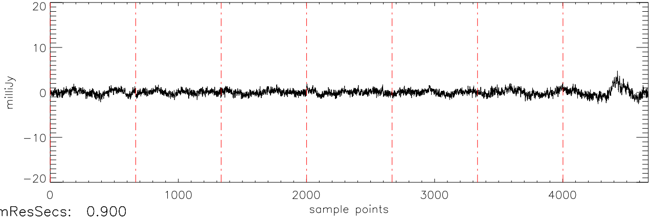
a2471 TVLM-513 31mar12 (AST) StokesU freq:5034.
