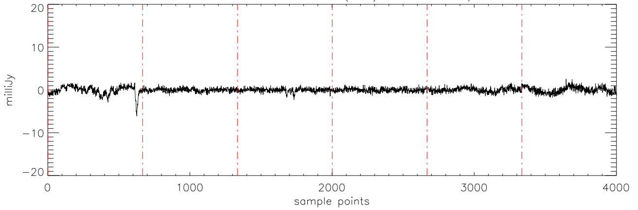
a2471 TVLM-513 30mar12 (AST) StokesV freq:4750.
