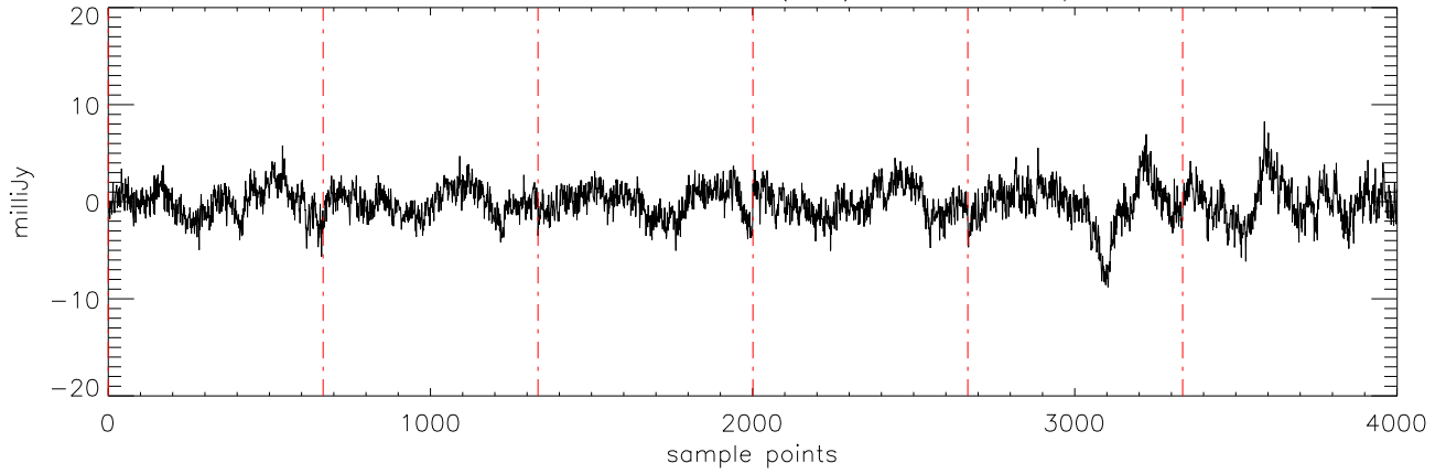
a2471 TVLM-513 30mar12 (AST) StokesQ freq:4750.
