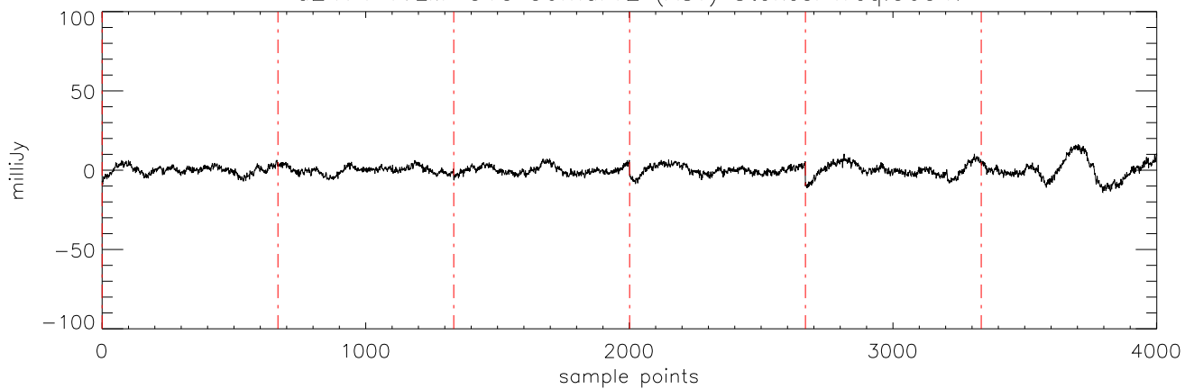
a2471 TVLM-513 30mar12 (AST) StokesI freq:5176.
