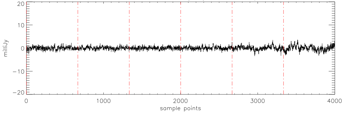
a2471 TVLM-513 30mar12 (AST) StokesV freq:5176.
