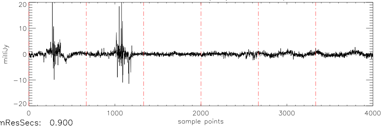
a2471 TVLM-513 30mar12 (AST) StokesV freq:4466.
