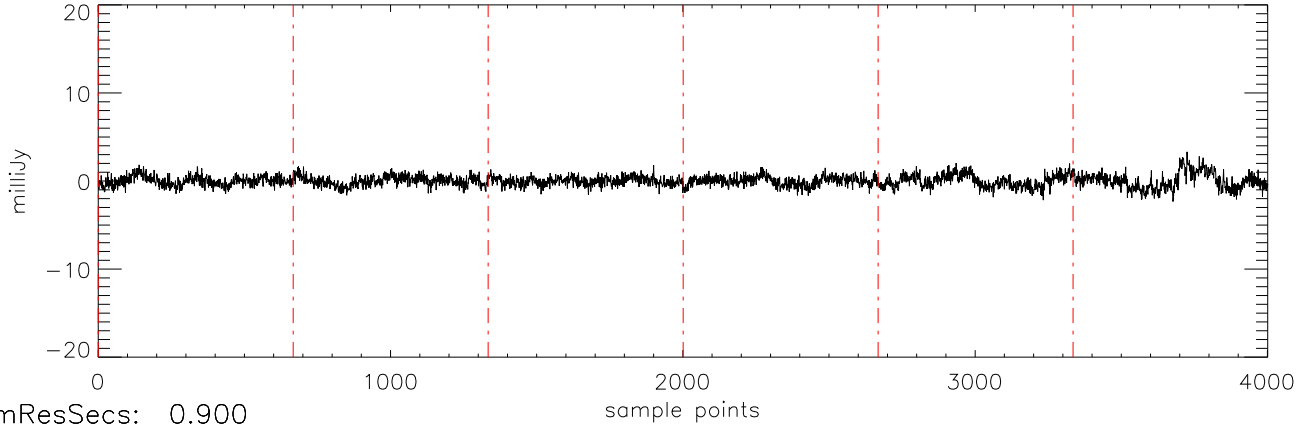
a2471 TVLM-513 30mar12 (AST) StokesU freq:5034.
