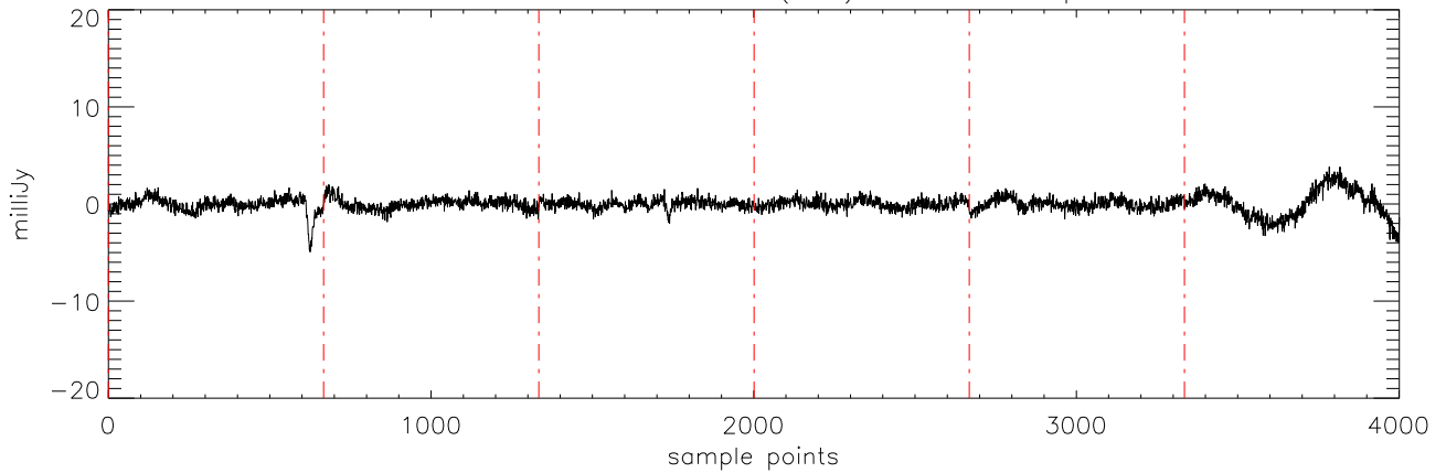
a2471 TVLM-513 30mar12 (AST) StokesU freq:4750.
