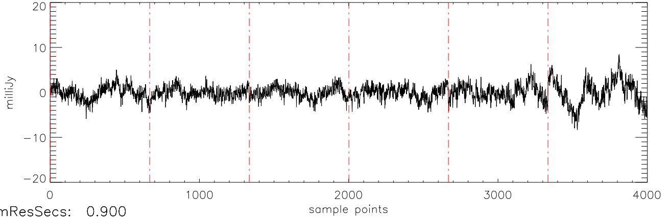
a2471 TVLM-513 30mar12 (AST) StokesQ freq:5034.
