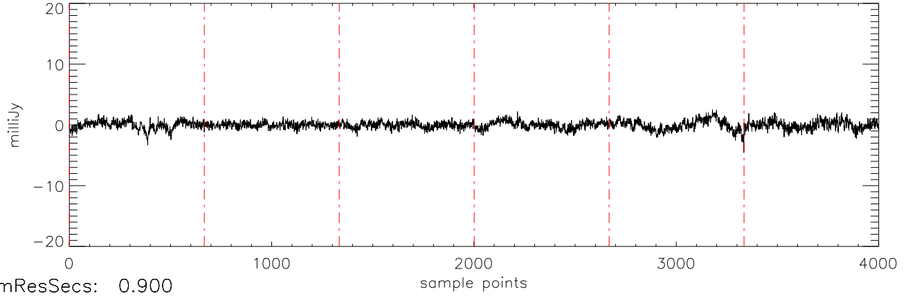
a2471 TVLM-513 30mar12 (AST) StokesV freq:5034.
