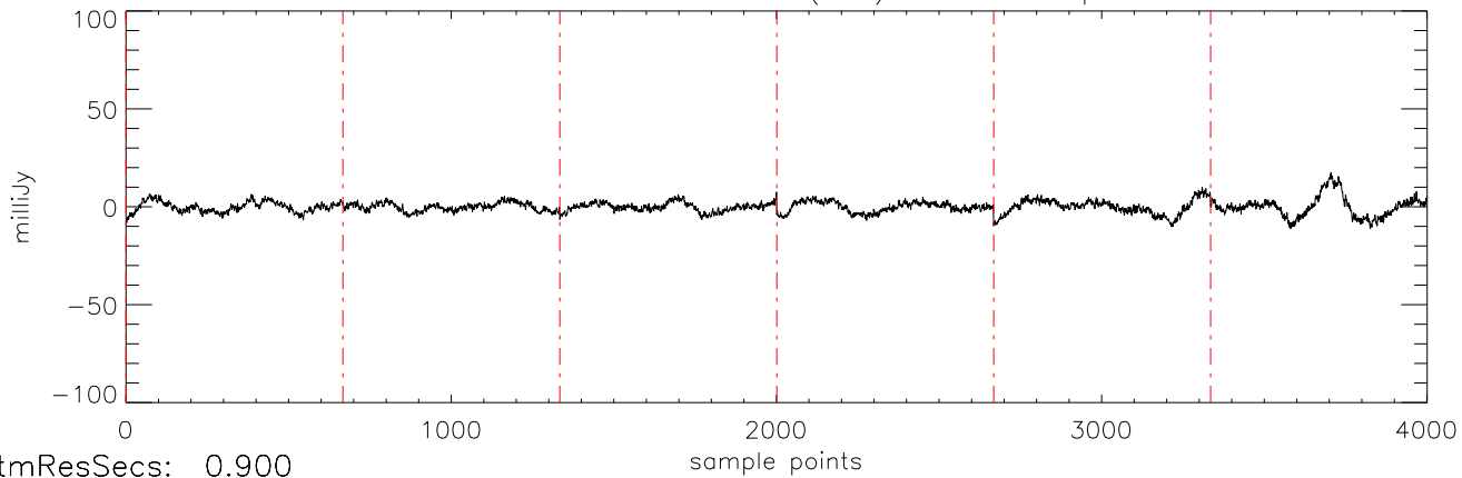
a2471 TVLM-513 30mar12 (AST) StokesI freq:5034.
