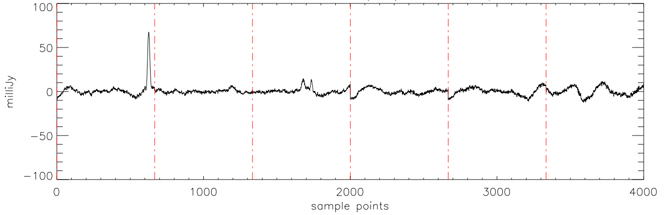
a2471 TVLM-513 30mar12 (AST) StokesI freq:4750.
