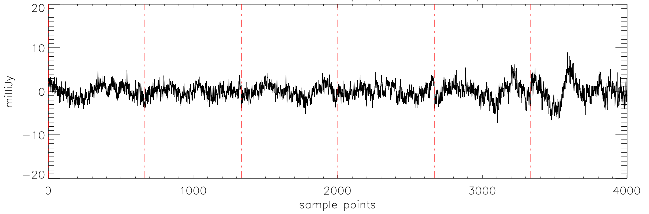
a2471 TVLM-513 30mar12 (AST) StokesQ freq:5176.
