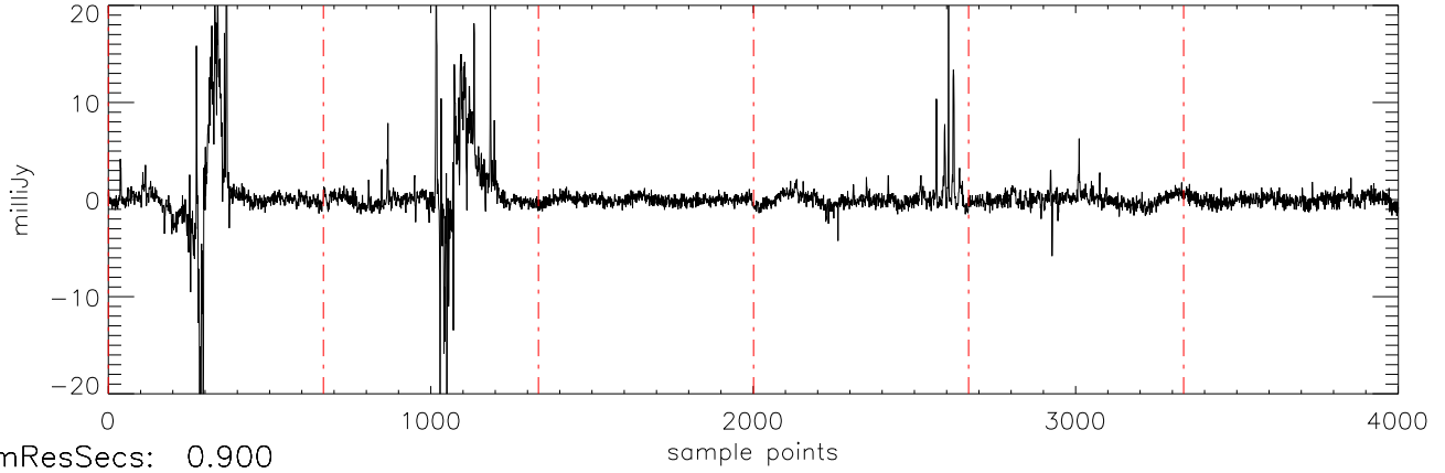
a2471 TVLM-513 30mar12 (AST) StokesU freq:4466.
