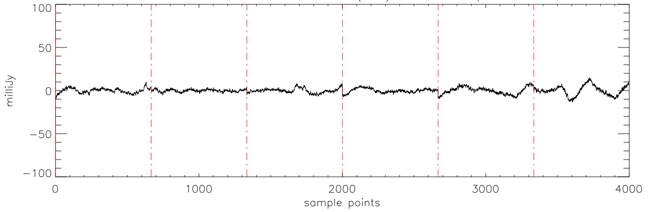
a2471 TVLM-513 30mar12 (AST) StokesI freq:4608.
