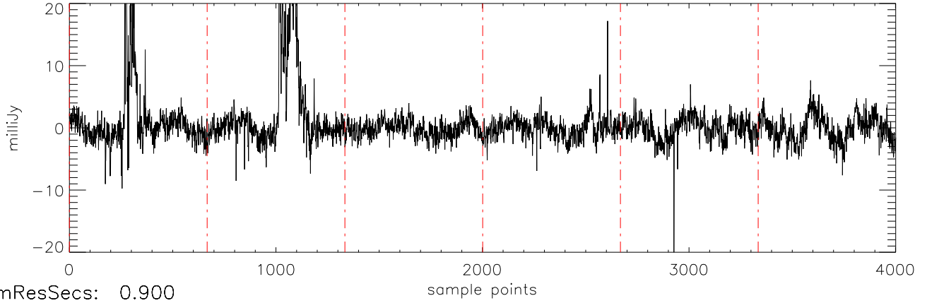
a2471 TVLM-513 30mar12 (AST) StokesQ freq:4466.
