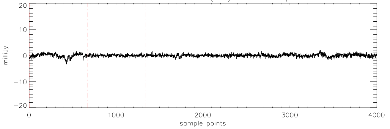
a2471 TVLM-513 30mar12 (AST) StokesV freq:4608.
