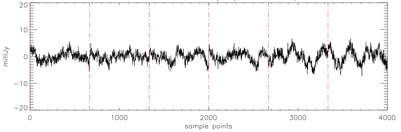
a2471 TVLM-513 30mar12 (AST) StokesQ freq:4608.
