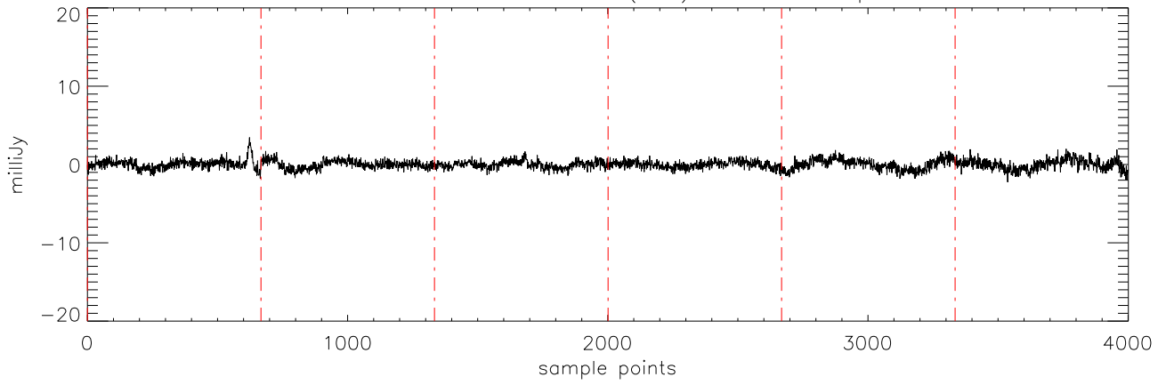
a2471 TVLM-513 30mar12 (AST) StokesU freq:4608.
