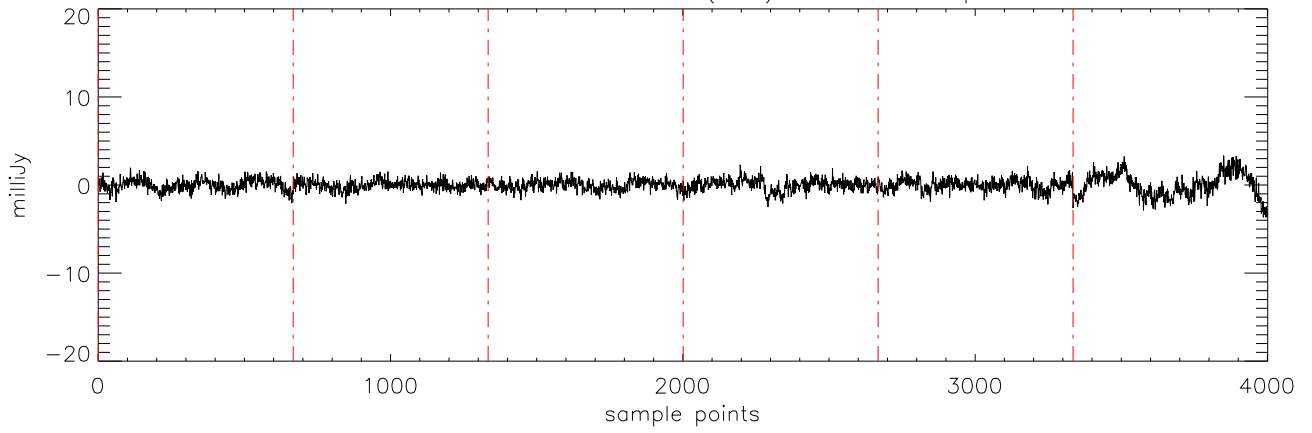
a2471 TVLM-513 30mar12 (AST) StokesU freq:5176.
