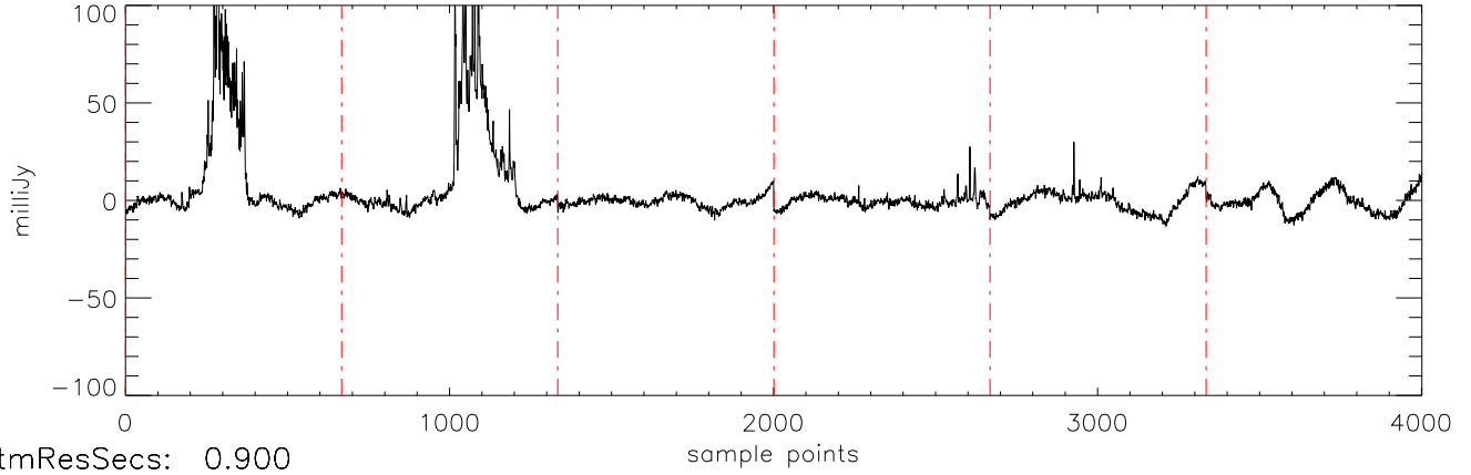
a2471 TVLM-513 30mar12 (AST) StokesI freq:4466.
