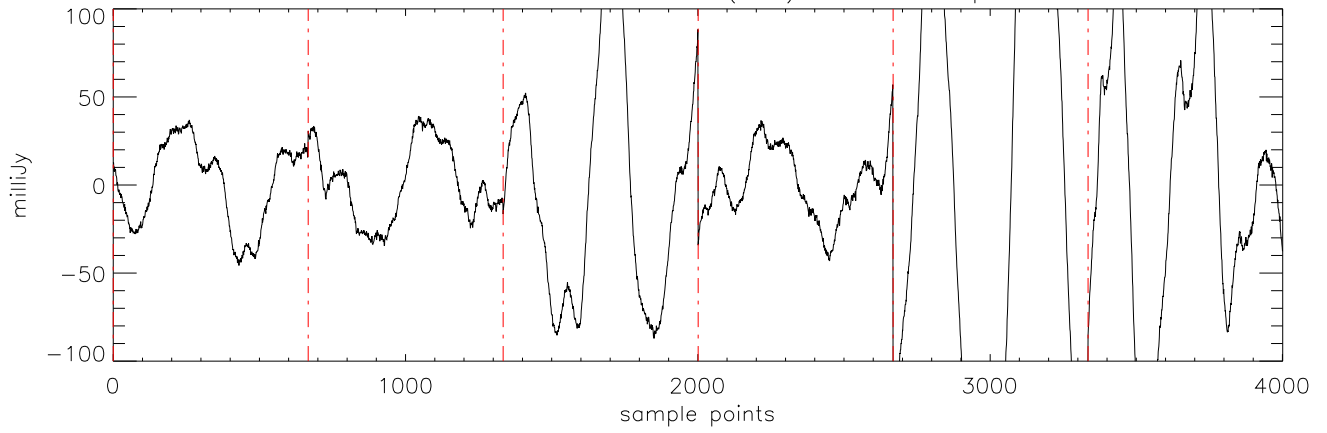
a2471 TVLM-513 29mar12 (AST) StokesI freq:5176.
