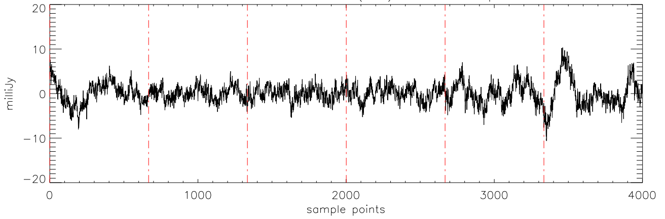
a2471 TVLM-513 29mar12 (AST) StokesQ freq:4608.
