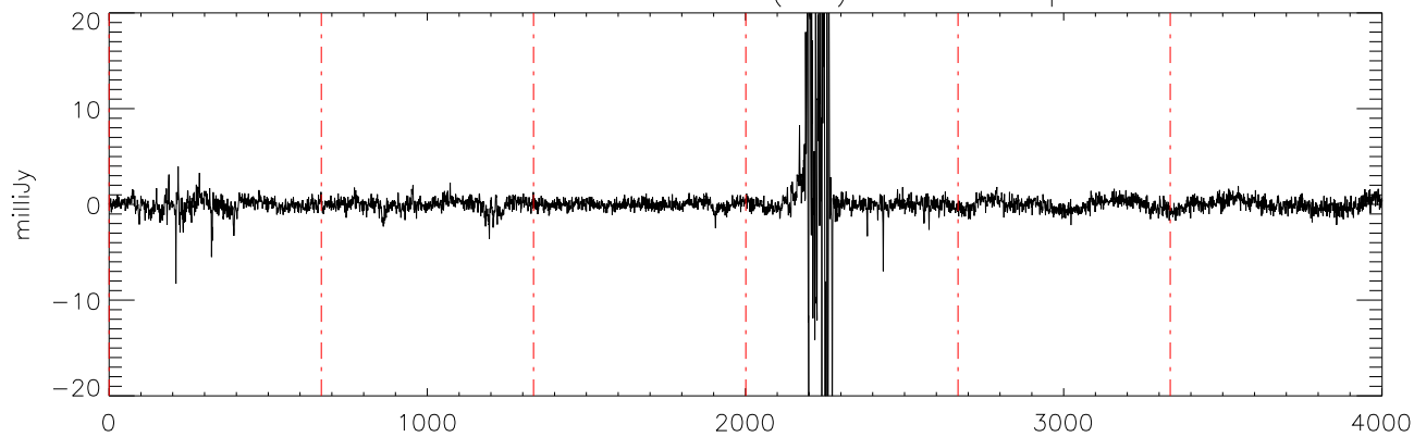
a2471 TVLM-513 29mar12 (AST) StokesV freq:4325.
