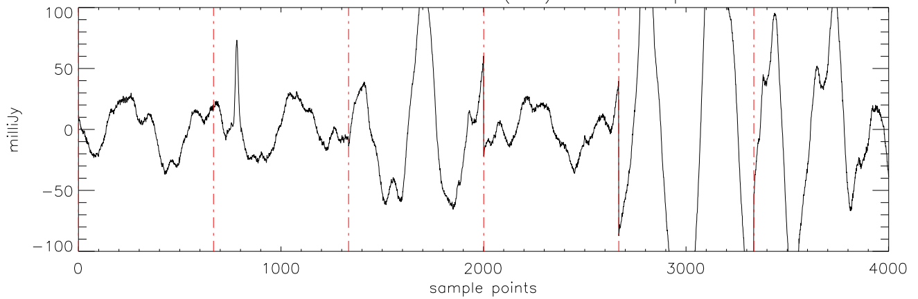
a2471 TVLM-513 29mar12 (AST) StokesI freq:4750.
