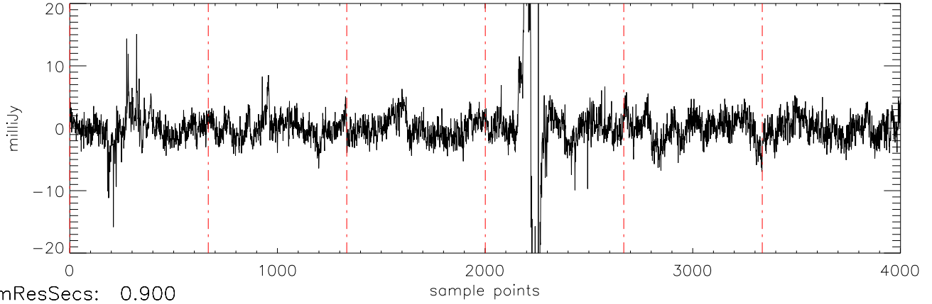
a2471 TVLM-513 29mar12 (AST) StokesQ freq:4466.
