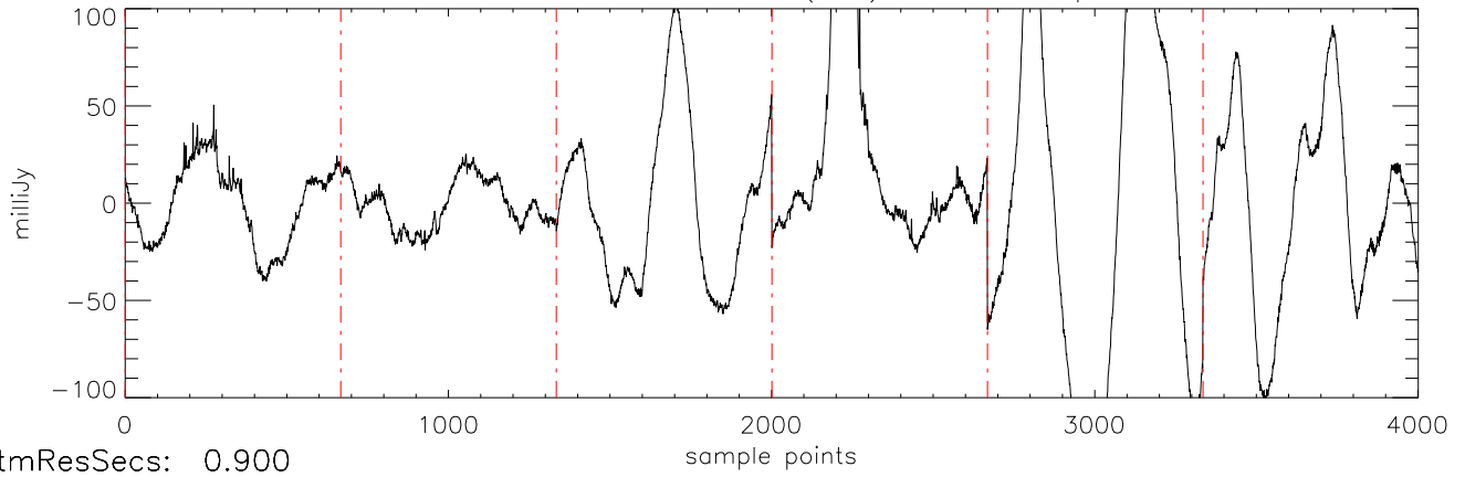
a2471 TVLM-513 29mar12 (AST) StokesI freq:4466.
