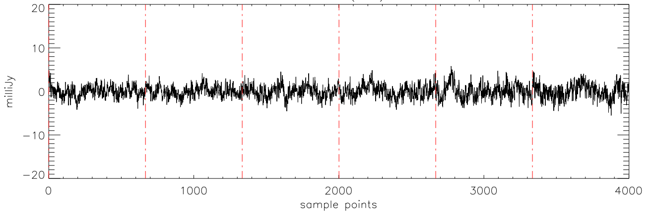
a2471 TVLM-513 29mar12 (AST) StokesQ freq:4750.
