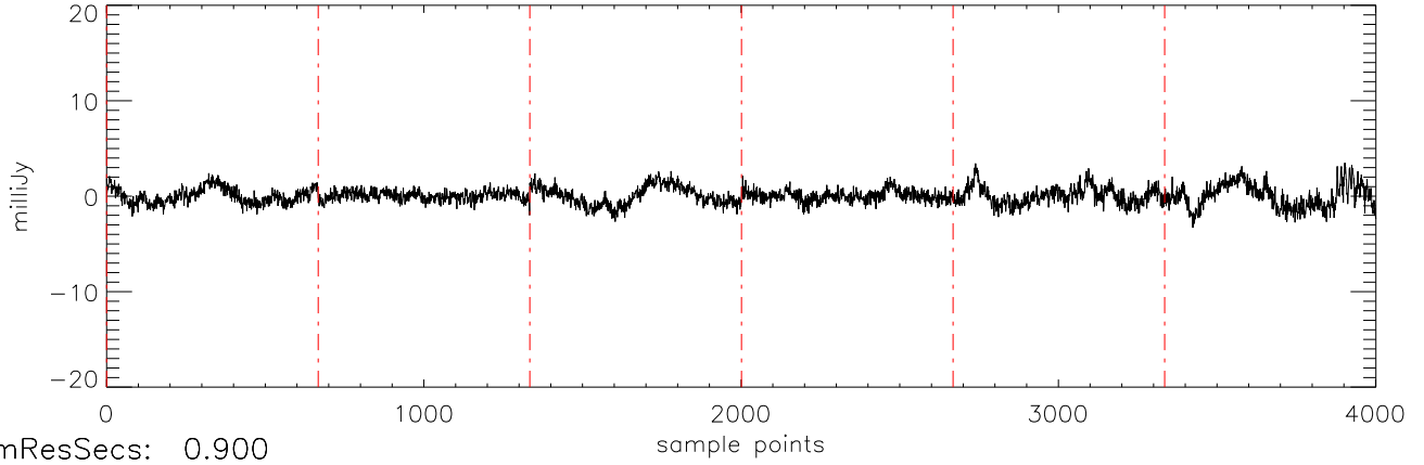
a2471 TVLM-513 29mar12 (AST) StokesU freq:5034.
