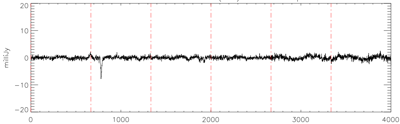
a2471 TVLM-513 29mar12 (AST) StokesV freq:4608.
