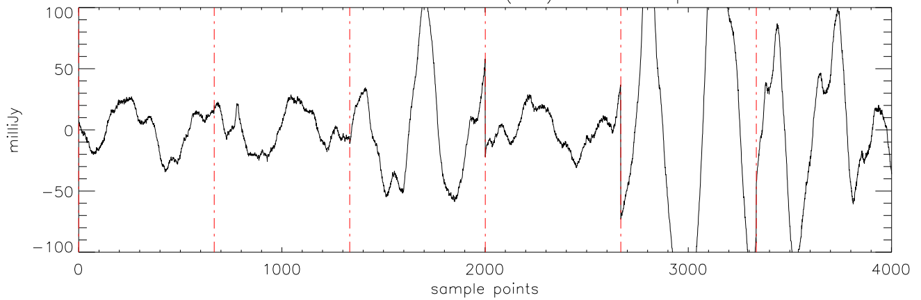
a2471 TVLM-513 29mar12 (AST) StokesI freq:4608.
