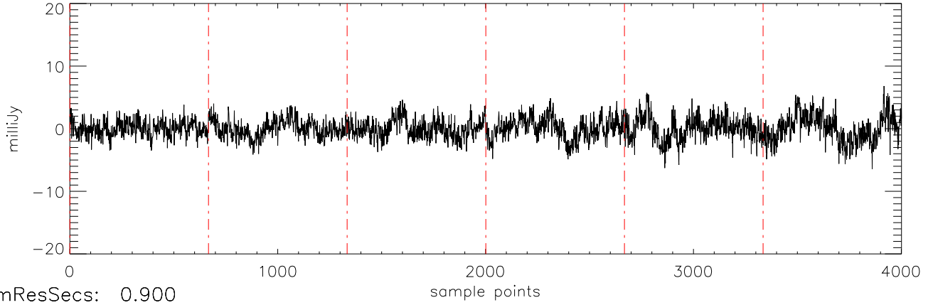
a2471 TVLM-513 29mar12 (AST) StokesQ freq:5034.
