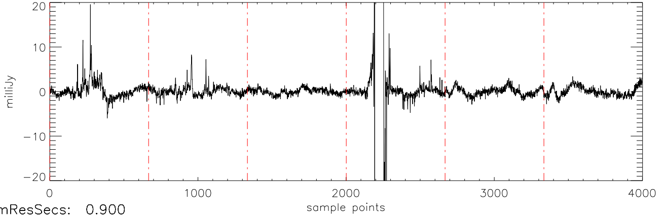
a2471 TVLM-513 29mar12 (AST) StokesU freq:4466.
