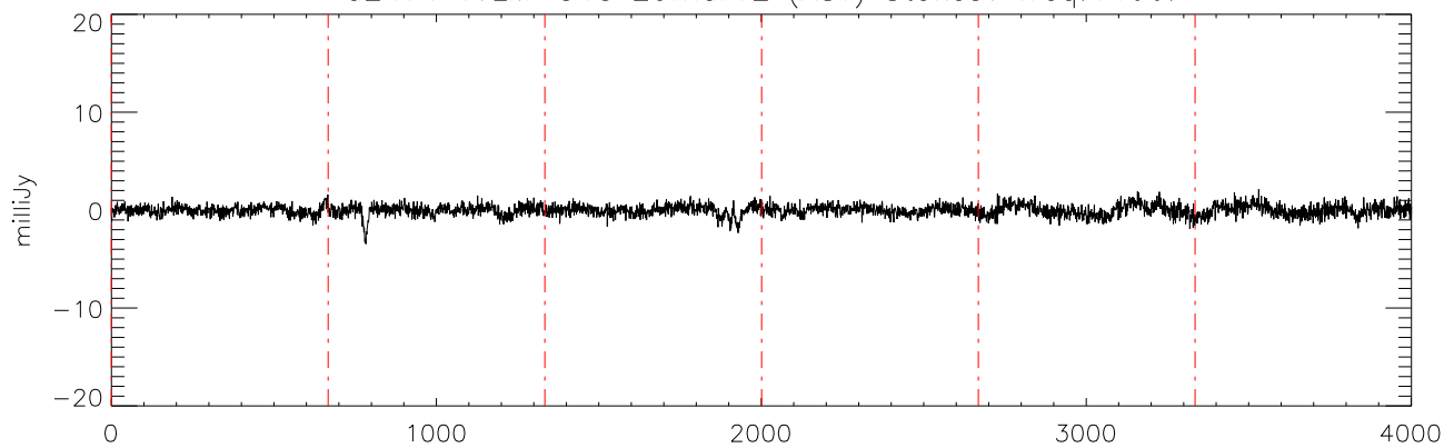
a2471 TVLM-513 29mar12 (AST) StokesV freq:4466.
