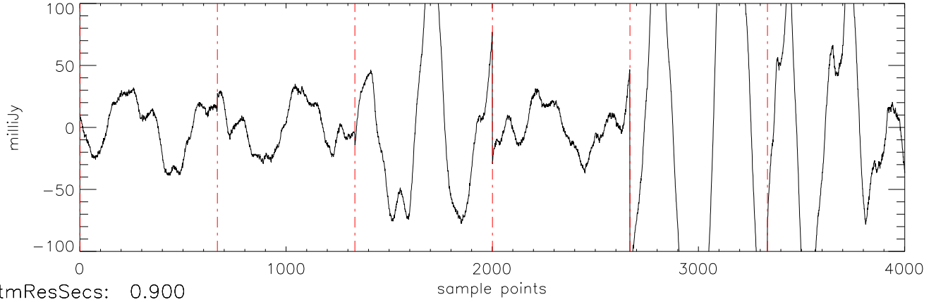
a2471 TVLM-513 29mar12 (AST) StokesI freq:5034.
