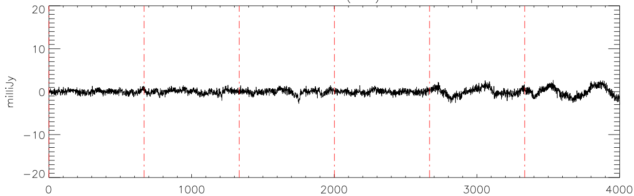
a2471 TVLM-513 29mar12 (AST) StokesV freq:4750.
