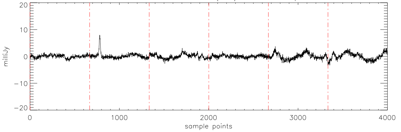
a2471 TVLM-513 29mar12 (AST) StokesU freq:4608.
