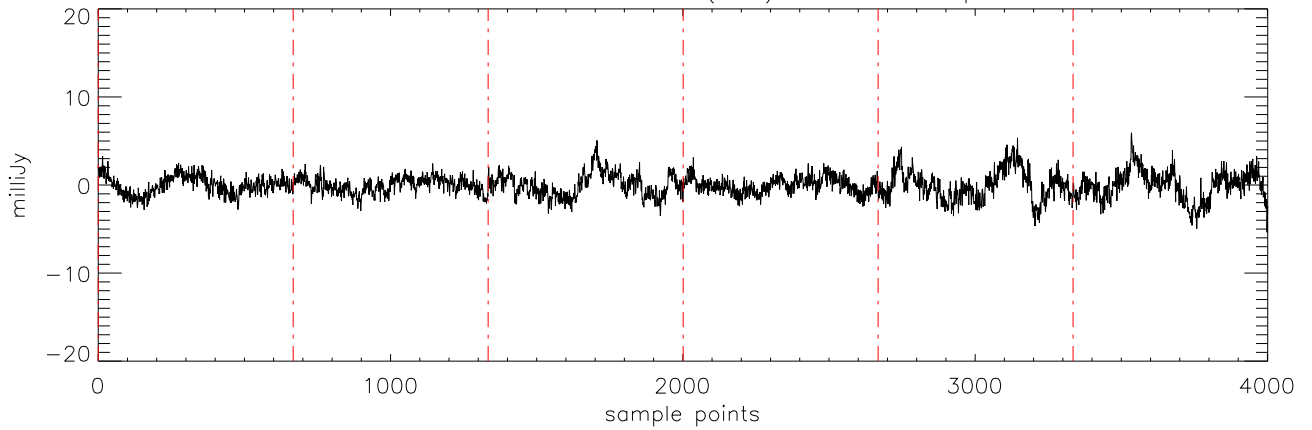
a2471 TVLM-513 29mar12 (AST) StokesU freq:5176.
