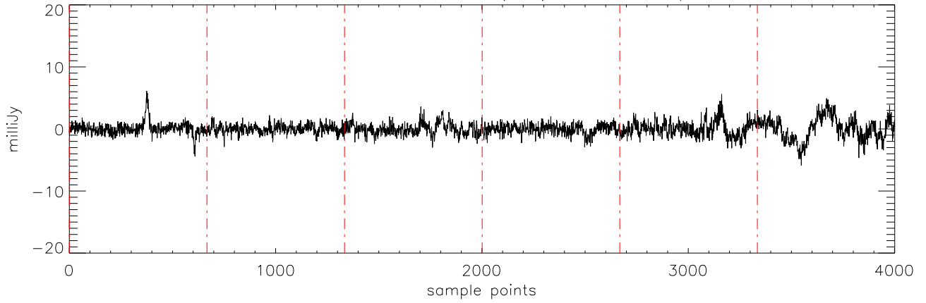
a2471 TVLM-513 29mar12 (AST) StokesV freq:5176.
