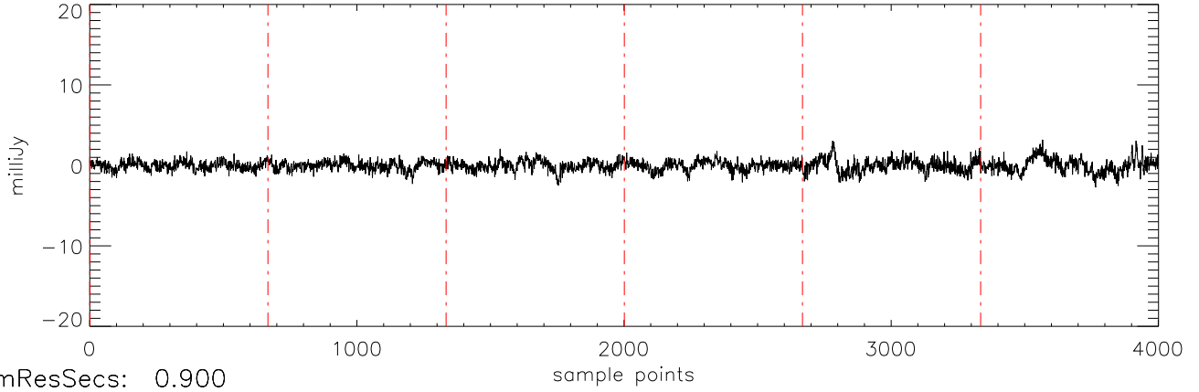
a2471 TVLM-513 29mar12 (AST) StokesV freq:5034.
