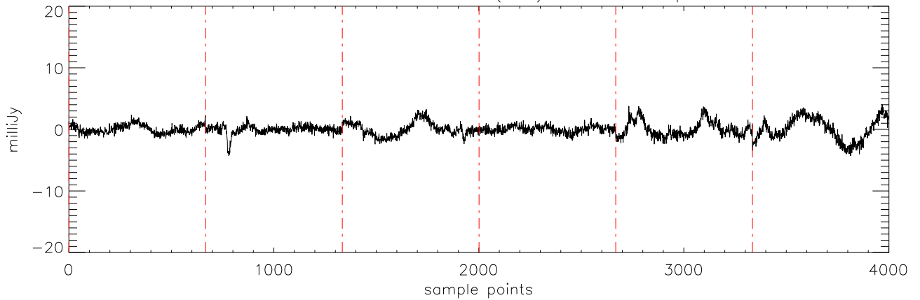
a2471 TVLM-513 29mar12 (AST) StokesU freq:4750.
