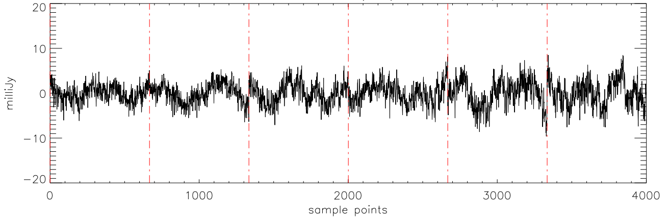
a2471 TVLM-513 29mar12 (AST) StokesQ freq:5176.
