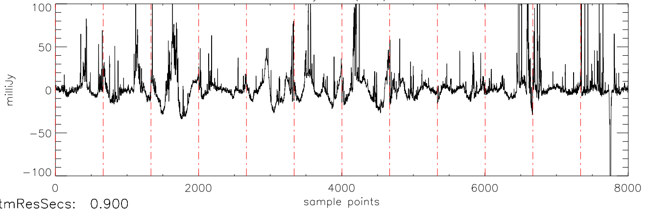
a2471 J21011544 18jul11 (AST) StokesI freq:5034.
