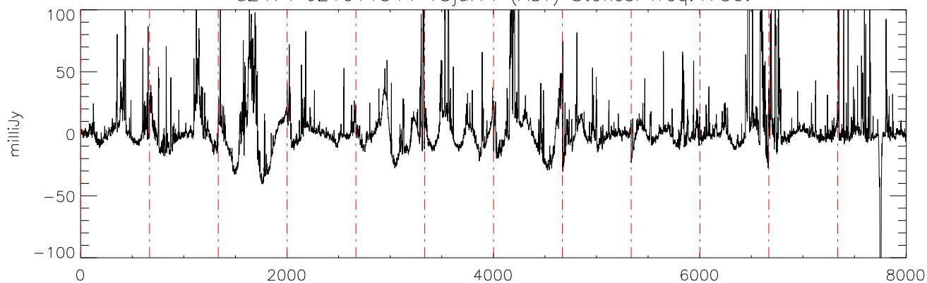
a2471 J21011544 18jul11 (AST) StokesI freq:4750.
