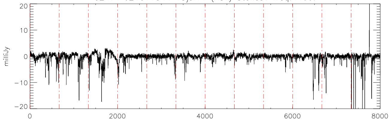
a2471 J21011544 18jul11 (AST) StokesV freq:4466.
