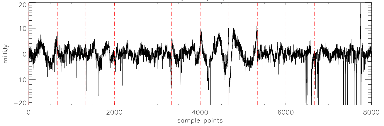
a2471 J21011544 18jul11 (AST) StokesQ freq:4608.
