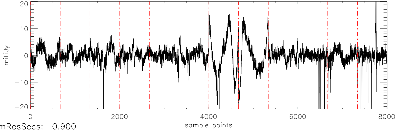
a2471 J21011544 18jul11 (AST) StokesQ freq:5034.
