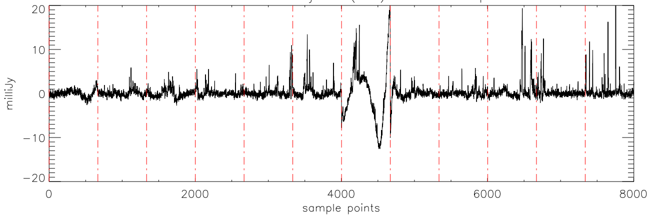
a2471 J21011544 18jul11 (AST) StokesU freq:4608.
