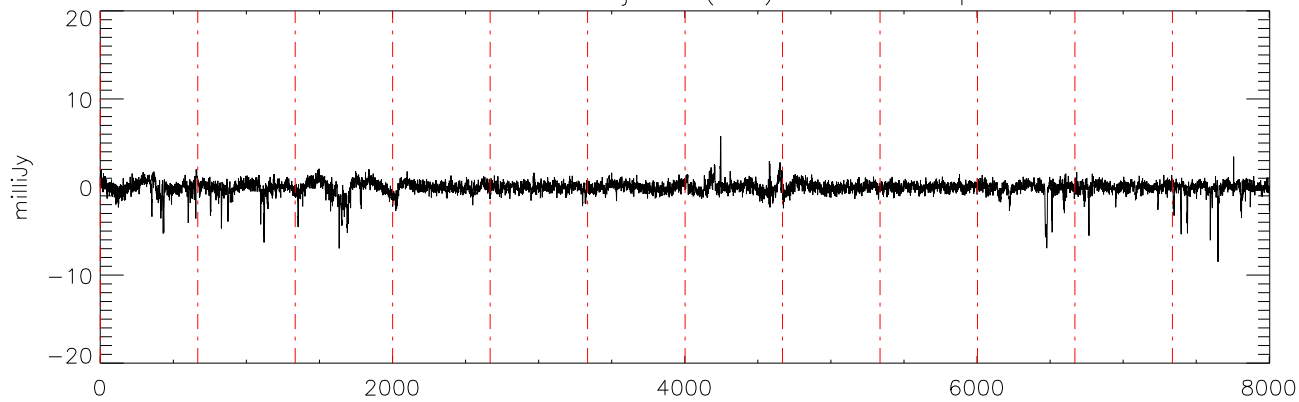
a2471 J21011544 18jul11 (AST) StokesV freq:4608.
