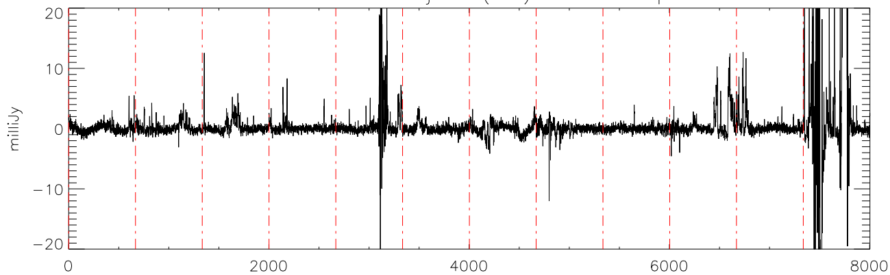
a2471 J21011544 18jul11 (AST) StokesV freq:4325.
