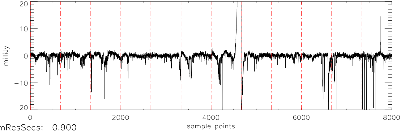
a2471 J21011544 18jul11 (AST) StokesU freq:5034.
