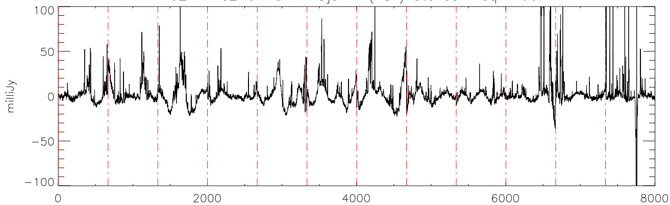
a2471 J21011544 18jul11 (AST) StokesI freq:4466.
