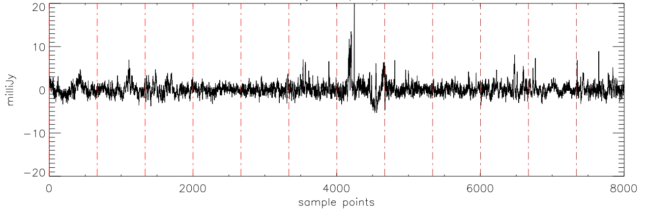
a2471 J21011544 18jul11 (AST) StokesV freq:5176.
