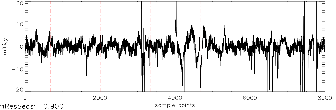
a2471 J21011544 18jul11 (AST) StokesQ freq:4466.
