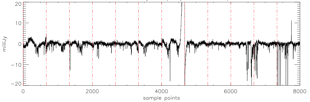
a2471 J21011544 18jul11 (AST) StokesU freq:4750.
