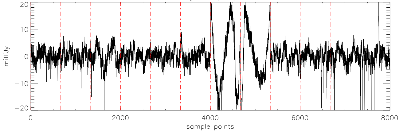
a2471 J21011544 18jul11 (AST) StokesQ freq:5176.
