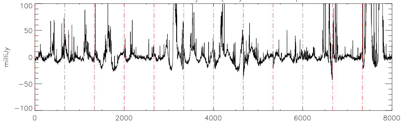
a2471 J21011544 18jul11 (AST) StokesI freq:4325.
