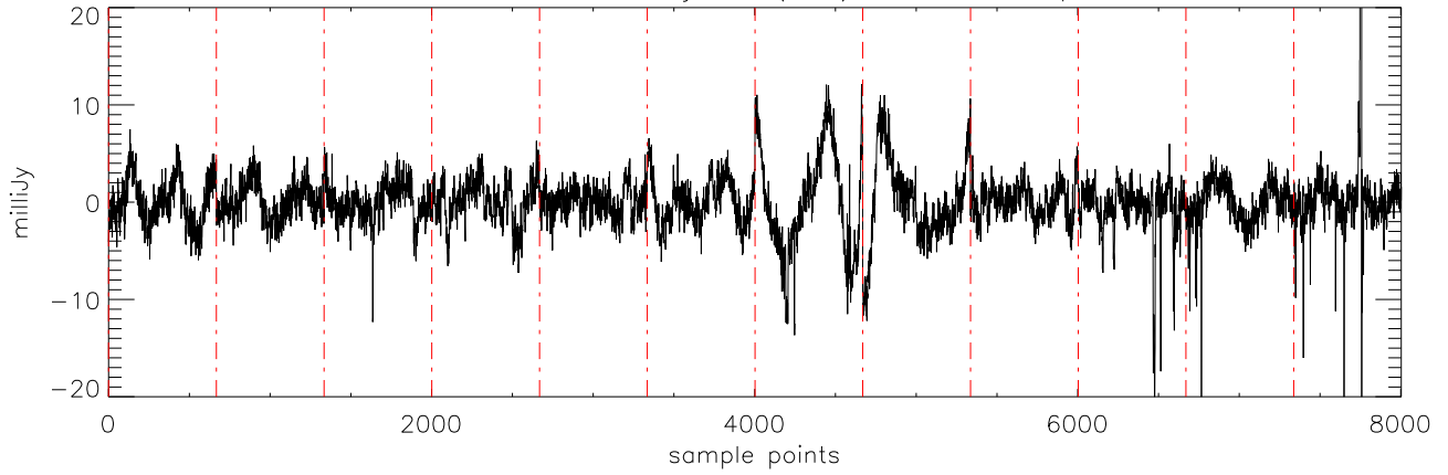
a2471 J21011544 18jul11 (AST) StokesQ freq:4750.
