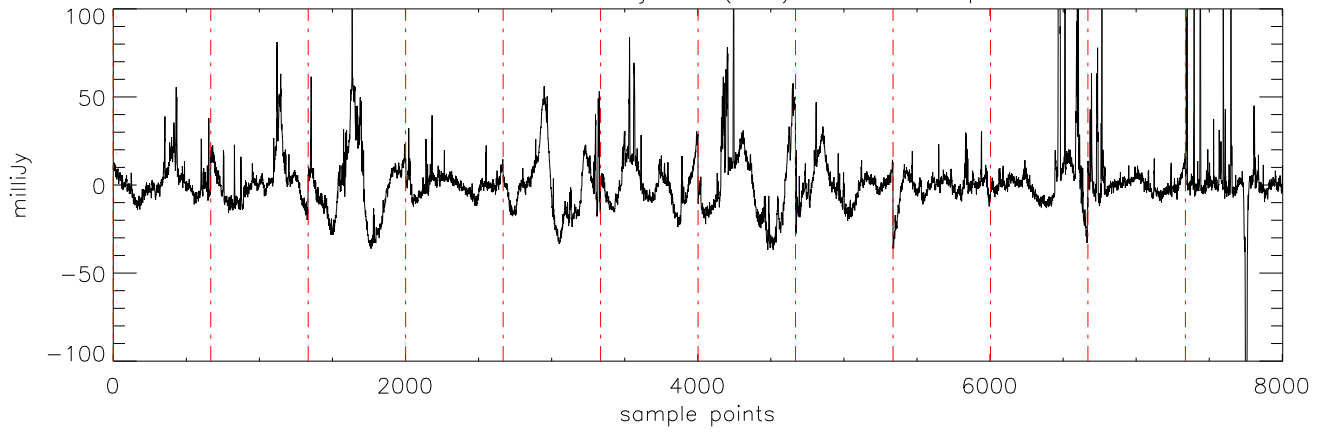
a2471 J21011544 18jul11 (AST) StokesI freq:5176.
