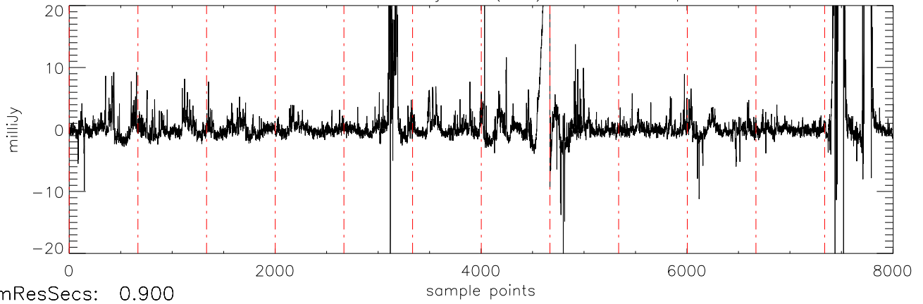
a2471 J21011544 18jul11 (AST) StokesU freq:4466.
