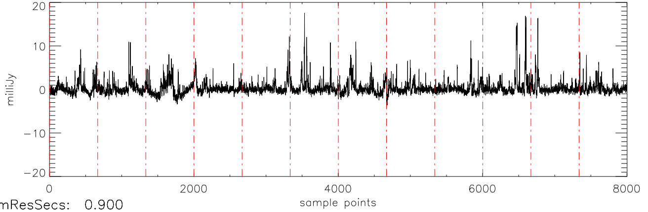
a2471 J21011544 18jul11 (AST) StokesV freq:5034.
