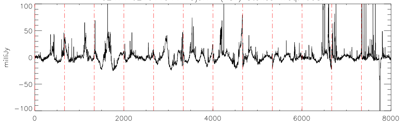
a2471 J21011544 18jul11 (AST) StokesI freq:4608.
