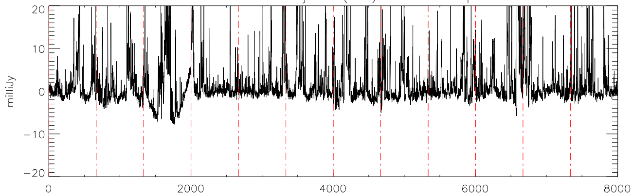
a2471 J21011544 18jul11 (AST) StokesV freq:4750.
