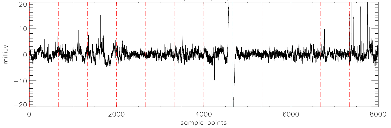
a2471 J21011544 18jul11 (AST) StokesU freq:5176.
