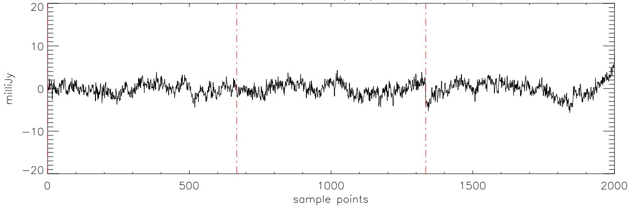
a2471 J1711457 11mar12 (AST) StokesQ freq:4750.
