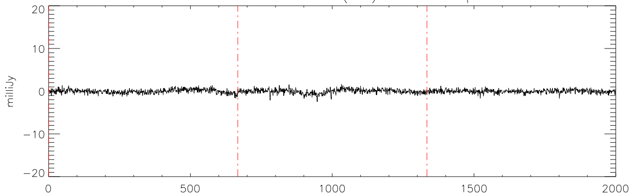
a2471 J1711457 11mar12 (AST) StokesV freq:4325.
