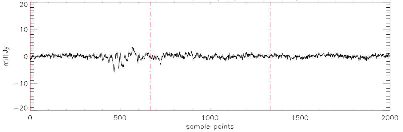
a2471 J1711457 11mar12 (AST) StokesU freq:4750.
