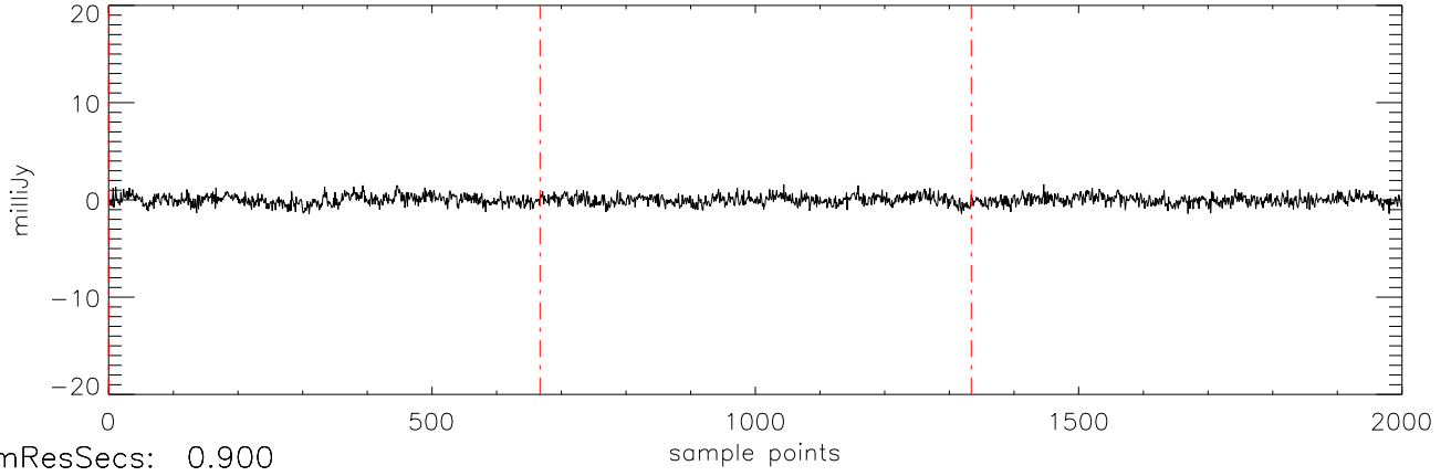
a2471 J1711457 11mar12 (AST) StokesV freq:5034.
