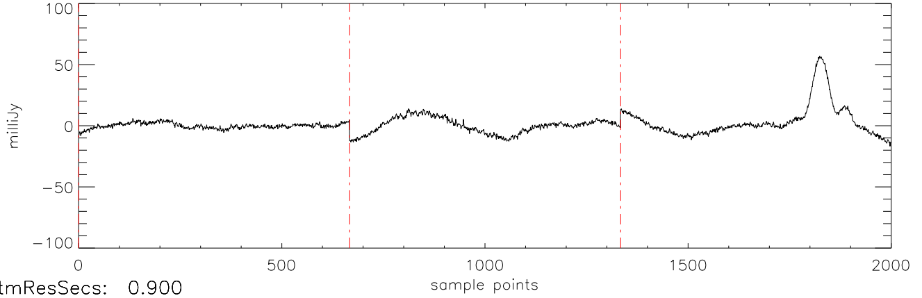
a2471 J1711457 11mar12 (AST) StokesI freq:4466.
