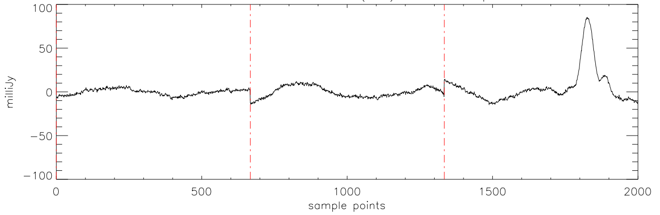
a2471 J1711457 11mar12 (AST) StokesI freq:5176.
