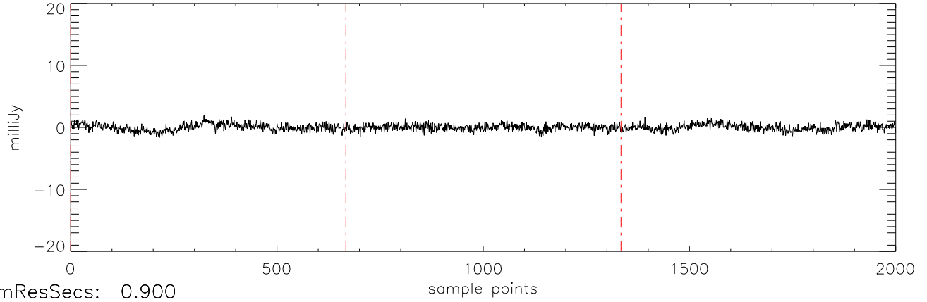
a2471 J1711457 11mar12 (AST) StokesU freq:5034.
