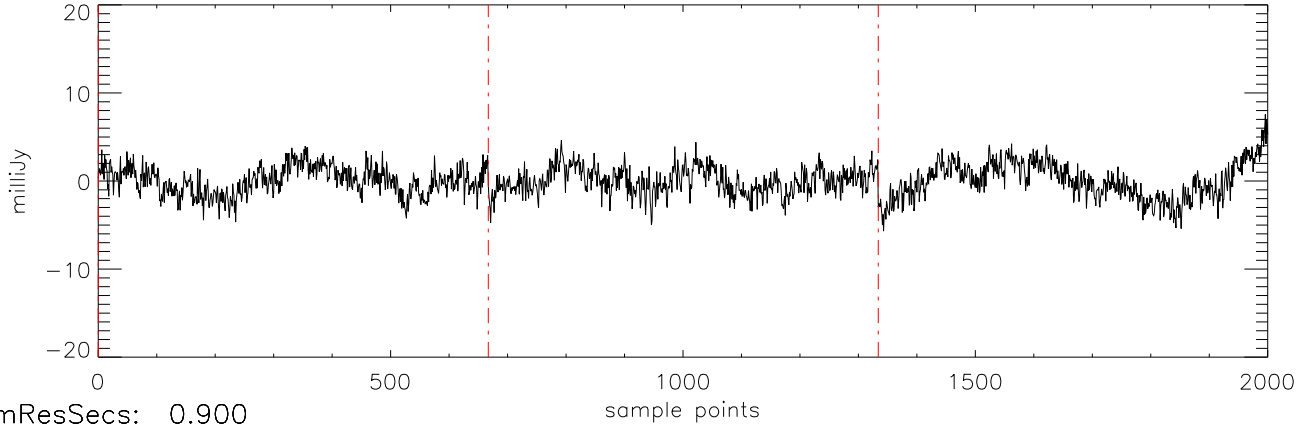
a2471 J1711457 11mar12 (AST) StokesQ freq:4466.
