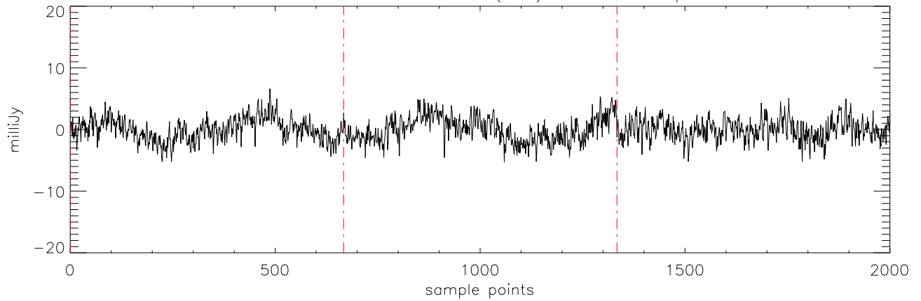
a2471 J17111457 11mar12 (AST) StokesQ freq:5176.
