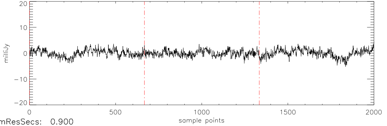
a2471 J17111457 11mar12 (AST) StokesQ freq:5034.
