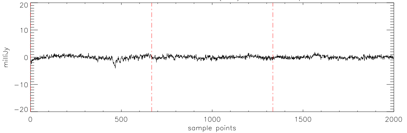
a2471 J1711457 11mar12 (AST) StokesU freq:4608.
