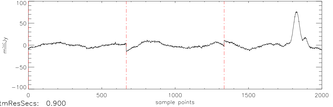
a2471 J1711457 11mar12 (AST) StokesI freq:5034.
