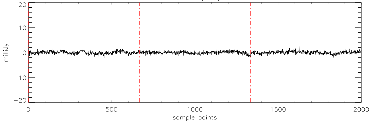
a2471 J1711457 11mar12 (AST) StokesU freq:5176.
