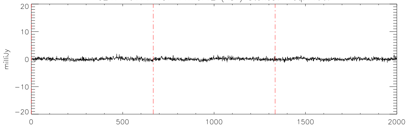
a2471 J1711457 11mar12 (AST) StokesV freq:4466.
