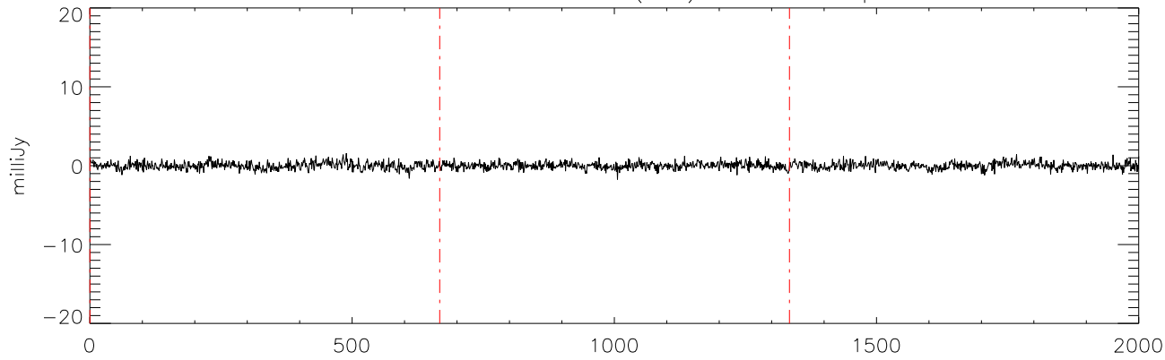
a2471 J1711457 11mar12 (AST) StokesV freq:4750.
