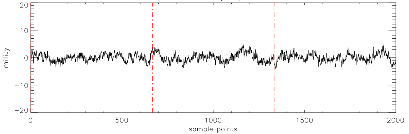
a2471 J1711457 11mar12 (AST) StokesQ freq:4608.
