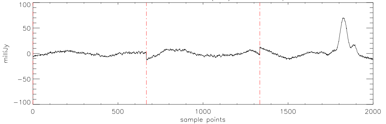
a2471 J1711457 11mar12 (AST) StokesI freq:4750.
