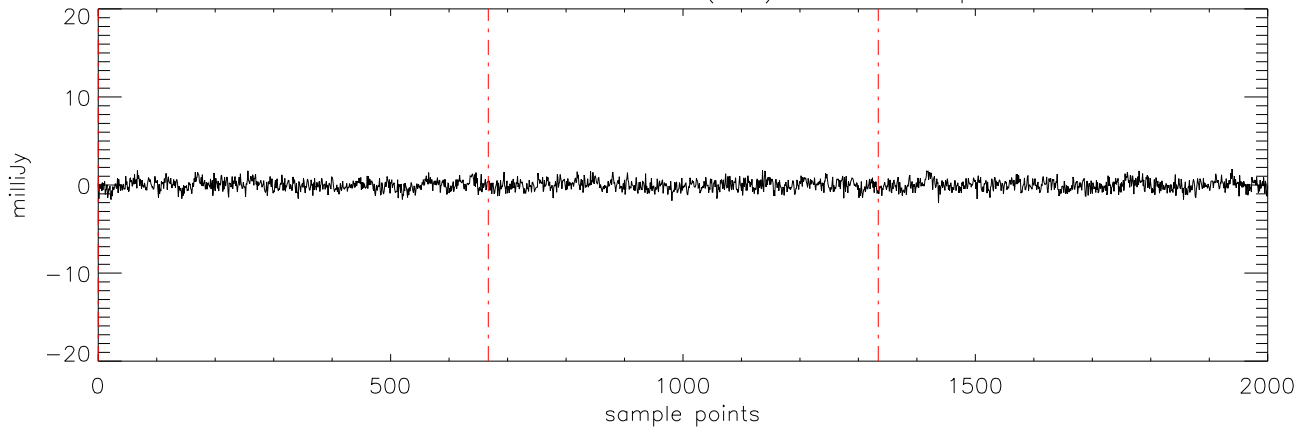
a2471 J1711457 11mar12 (AST) StokesV freq:5176.
