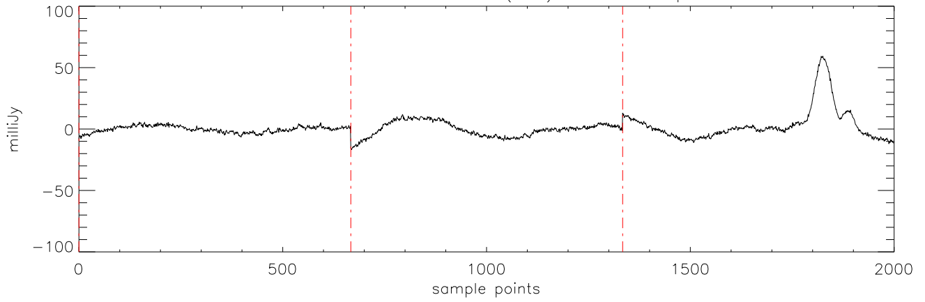
a2471 J1711457 11mar12 (AST) StokesI freq:4608.
