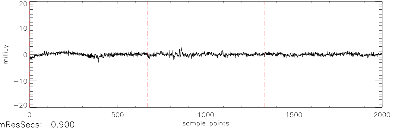
a2471 J1711457 11mar12 (AST) StokesU freq:4466.
