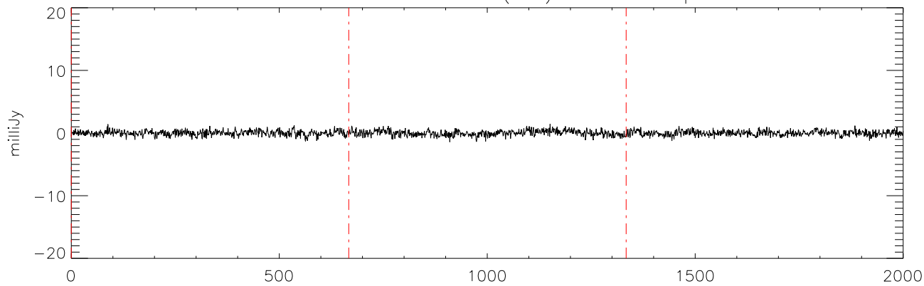
a2471 J1711457 11mar12 (AST) StokesV freq:4608.
