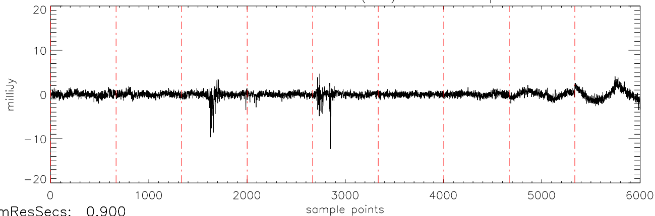
a2471 J16322911 29mar12 (AST) StokesV freq:4466.
