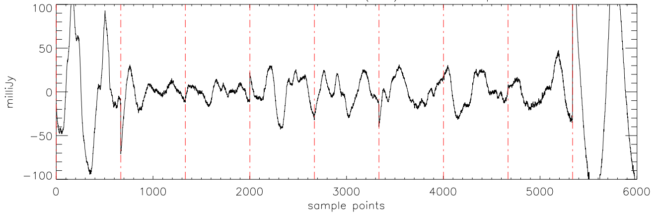
a2471 J16322911 29mar12 (AST) StokesI freq:5176.
