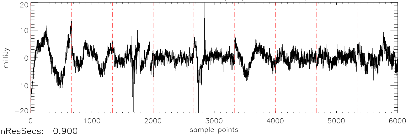
a2471 J16322911 29mar12 (AST) StokesQ freq:4466.
