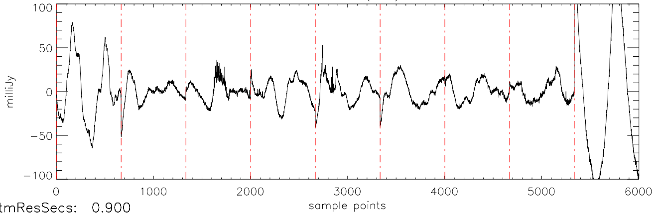
a2471 J16322911 29mar12 (AST) StokesI freq:4466.
