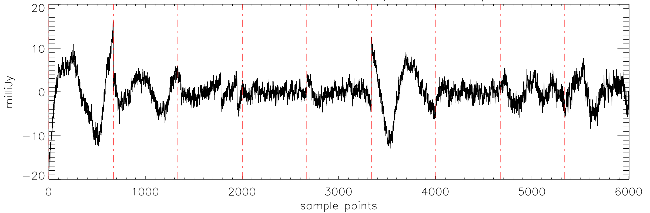
a2471 J16322911 29mar12 (AST) StokesQ freq:4750.
