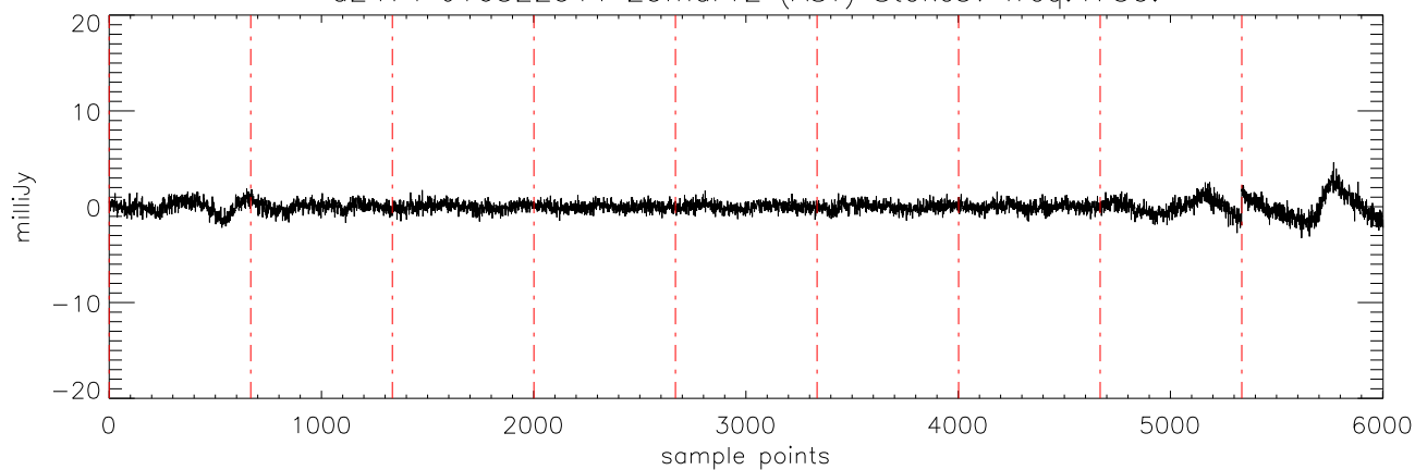
a2471 J16322911 29mar12 (AST) StokesV freq:4750.
