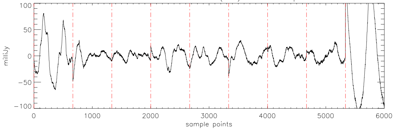
a2471 J16322911 29mar12 (AST) StokesI freq:4608.
