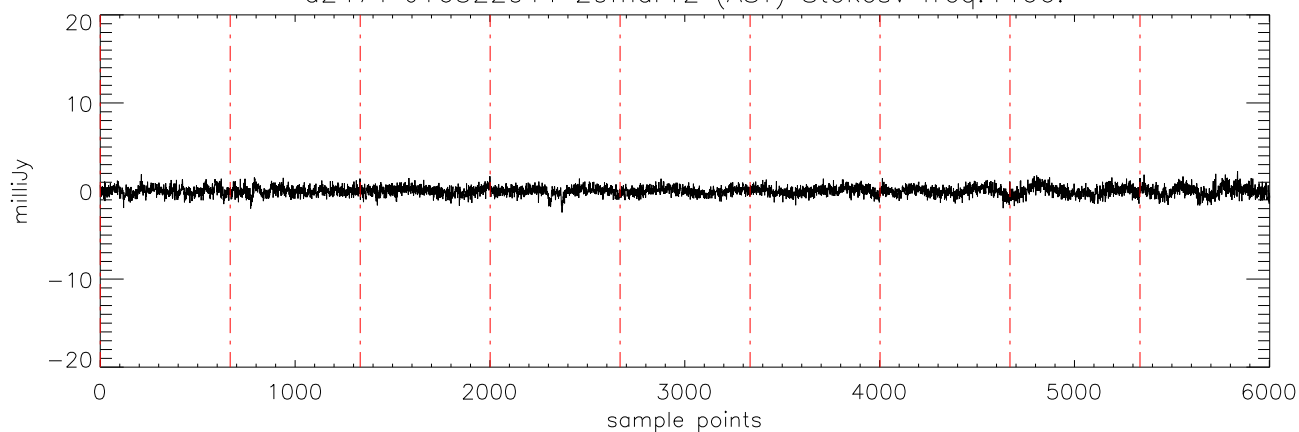
a2471 J16322911 29mar12 (AST) StokesV freq:4608.
