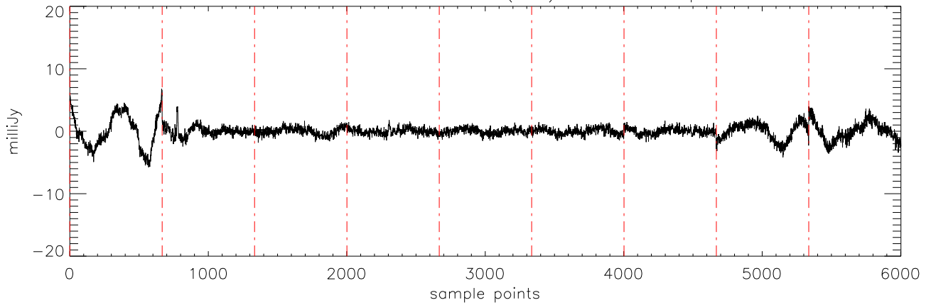
a2471 J16322911 29mar12 (AST) StokesU freq:4608.
