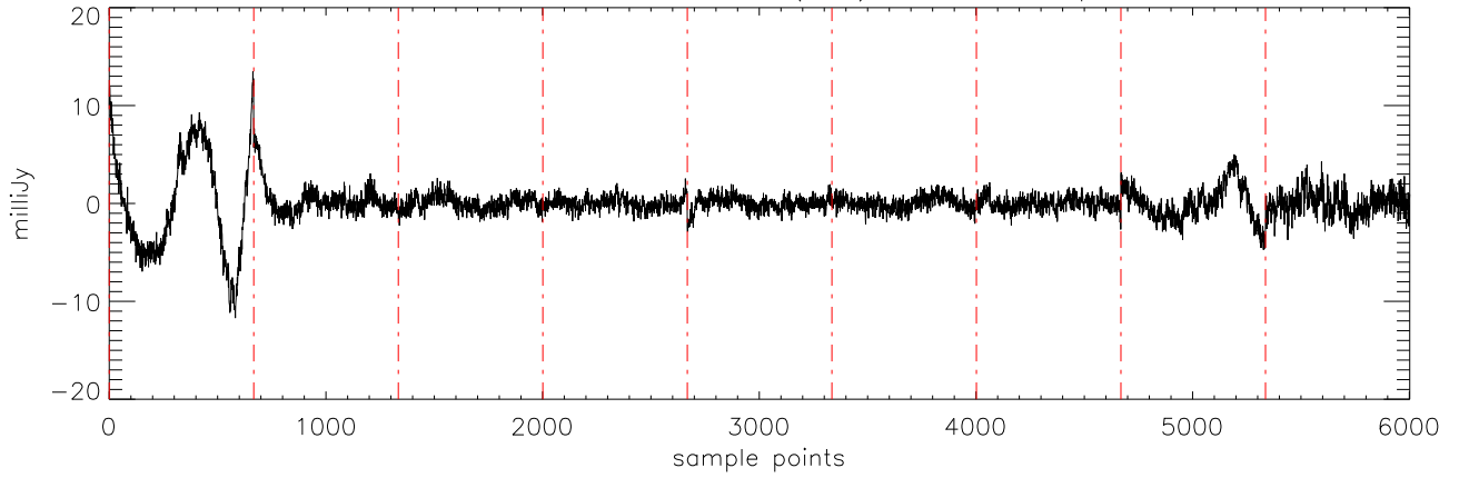
a2471 J16322911 29mar12 (AST) StokesU freq:5176.
