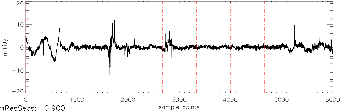
a2471 J16322911 29mar12 (AST) StokesU freq:4466.
