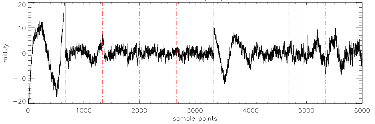
a2471 J16322911 29mar12 (AST) StokesQ freq:5176.
