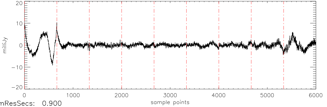
a2471 J16322911 29mar12 (AST) StokesU freq:5034.
