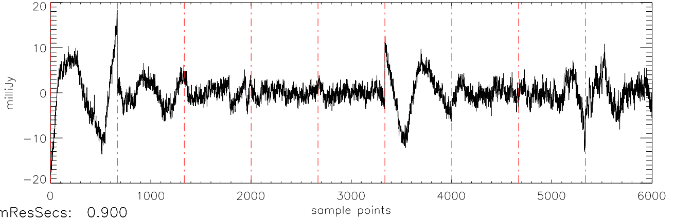
a2471 J16322911 29mar12 (AST) StokesQ freq:5034.
