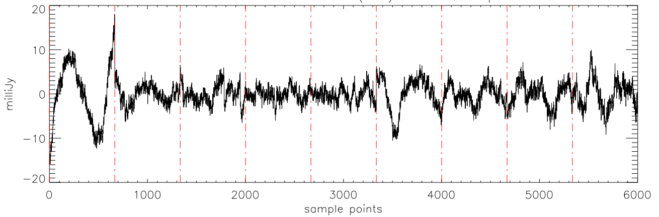
a2471 J16322911 29mar12 (AST) StokesQ freq:4608.
