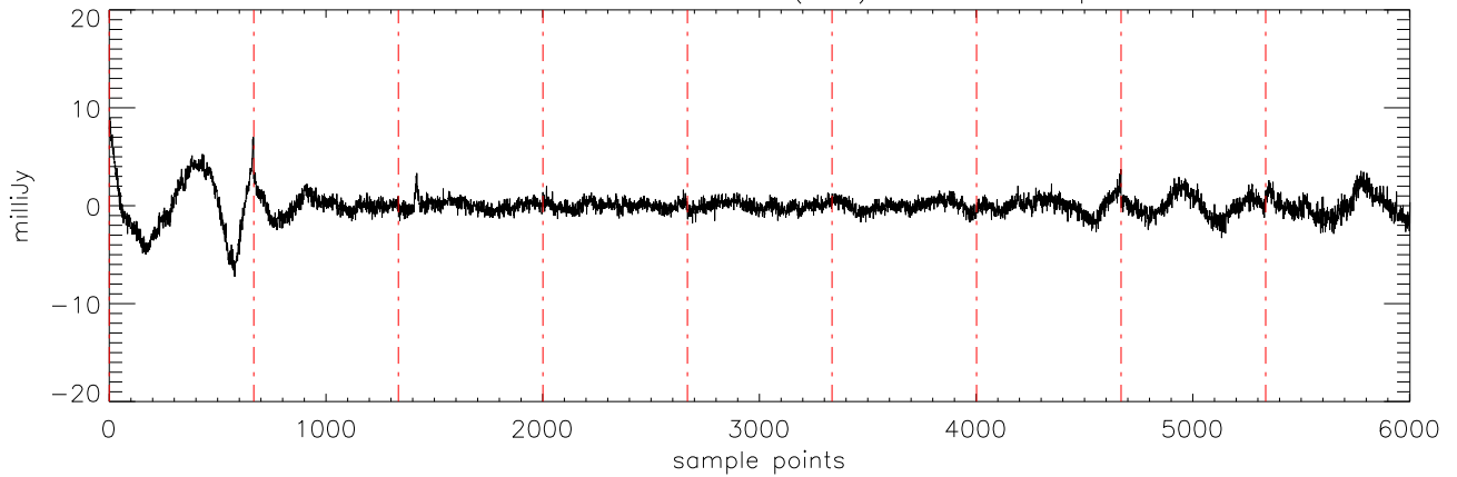
a2471 J16322911 29mar12 (AST) StokesU freq:4750.
