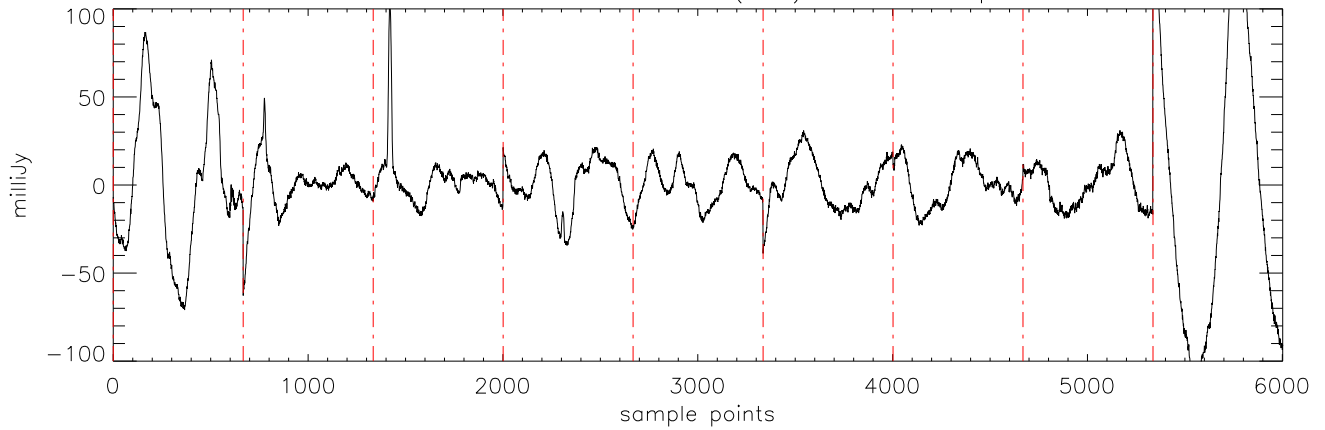
a2471 J16322911 29mar12 (AST) StokesI freq:4750.
