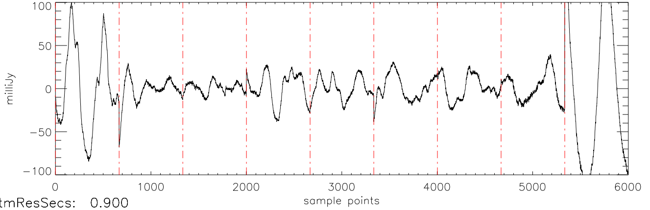
a2471 J16322911 29mar12 (AST) StokesI freq:5034.
