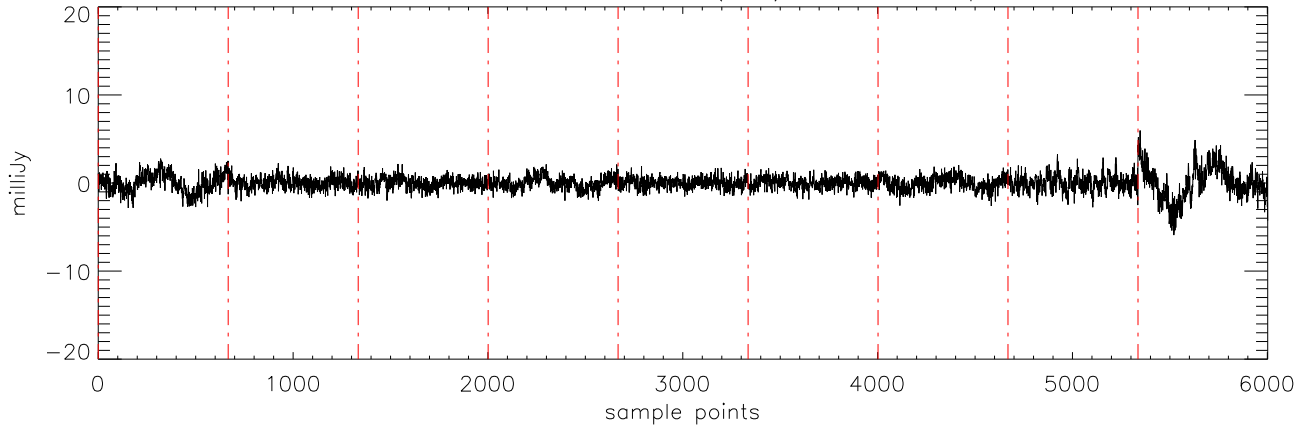
a2471 J16322911 29mar12 (AST) StokesV freq:5176.
