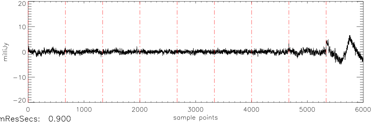
a2471 J16322911 29mar12 (AST) StokesV freq:5034.
