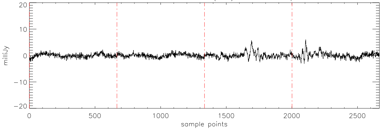
a2471 J16241436 09mar12 (AST) StokesU freq:4608.
