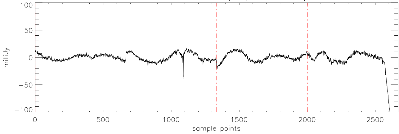
a2471 J16241436 09mar12 (AST) StokesI freq:5176.
