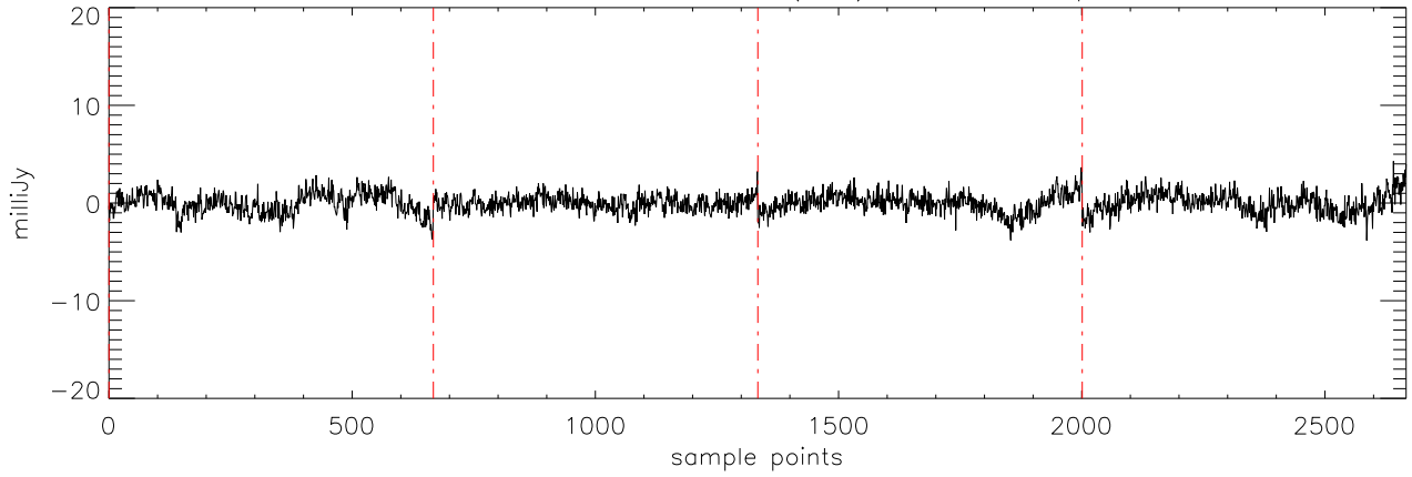
a2471 J16241436 09mar12 (AST) StokesU freq:5176.
