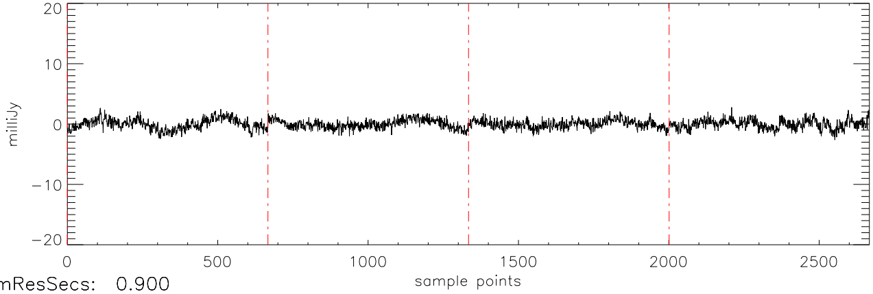
a2471 J16241436 09mar12 (AST) StokesU freq:5034.
