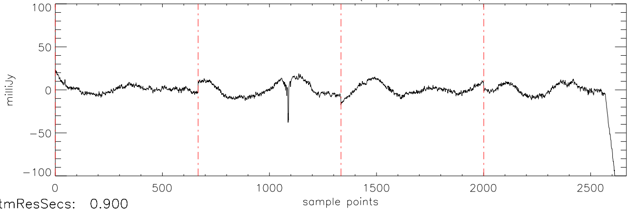
a2471 J16241436 09mar12 (AST) StokesI freq:5034.
