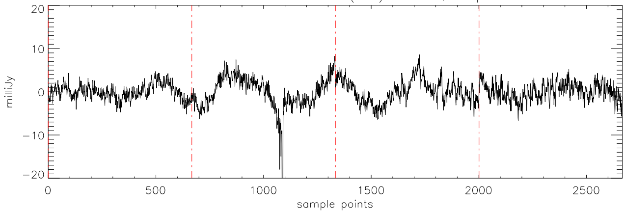
a2471 J16241436 09mar12 (AST) StokesQ freq:4608.
