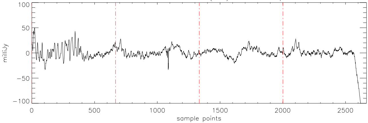
a2471 J16241436 09mar12 (AST) StokesI freq:4750.
