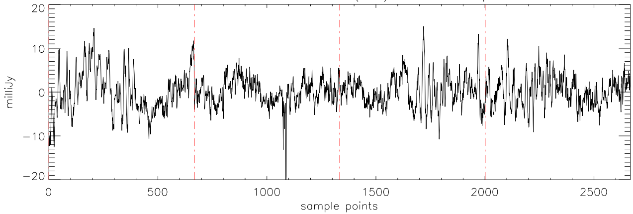
a2471 J16241436 09mar12 (AST) StokesQ freq:4750.
