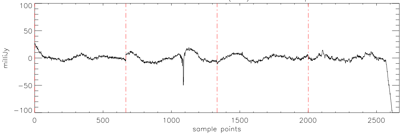
a2471 J16241436 09mar12 (AST) StokesI freq:4608.
