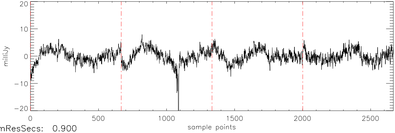
a2471 J16241436 09mar12 (AST) StokesQ freq:5034.
