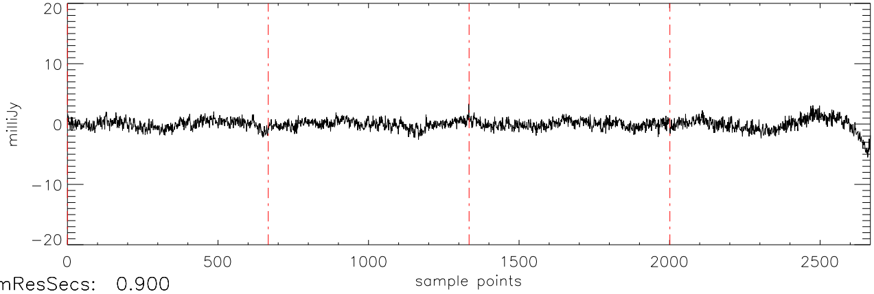
a2471 J16241436 09mar12 (AST) StokesV freq:5034.
