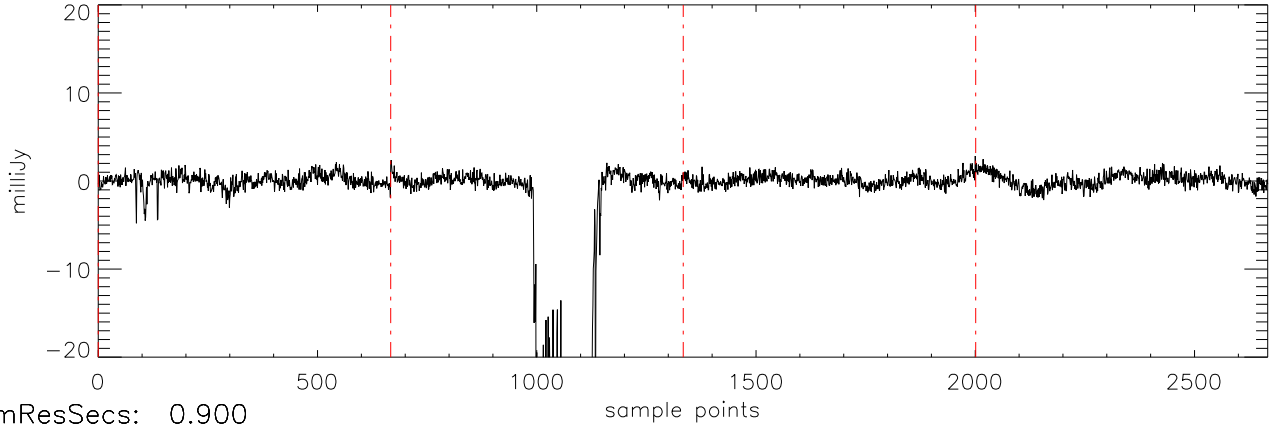
a2471 J16241436 09mar12 (AST) StokesU freq:4466.
