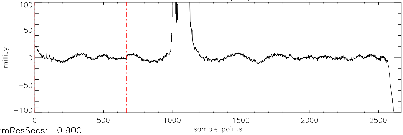
a2471 J16241436 09mar12 (AST) StokesI freq:4466.
