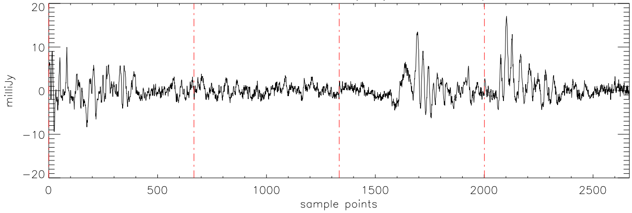
a2471 J16241436 09mar12 (AST) StokesU freq:4750.
