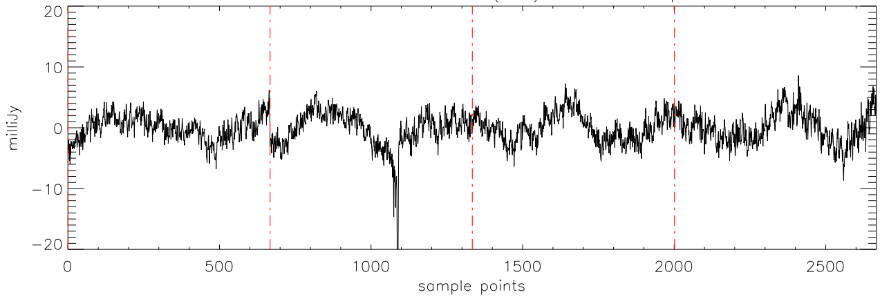
a2471 J16241436 09mar12 (AST) StokesQ freq:5176.
