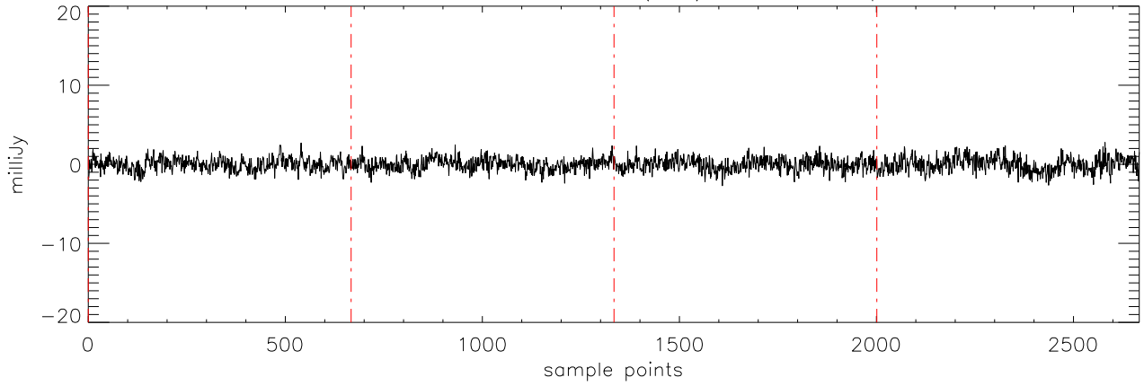
a2471 J16241436 09mar12 (AST) StokesV freq:5176.
