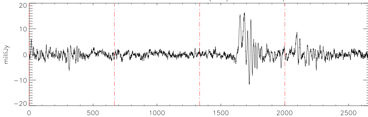
a2471 J16241436 09mar12 (AST) StokesV freq:4608.
