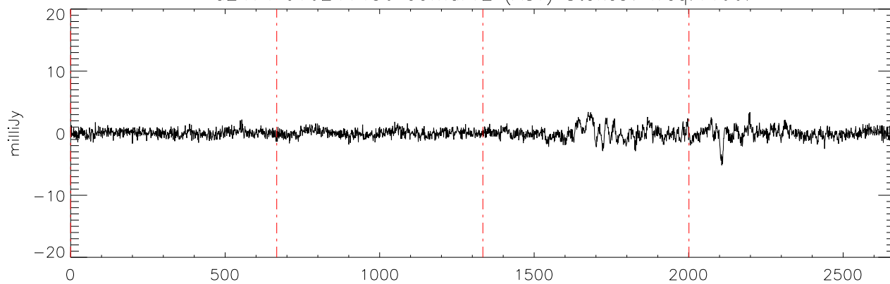
a2471 J16241436 09mar12 (AST) StokesV freq:4466.
