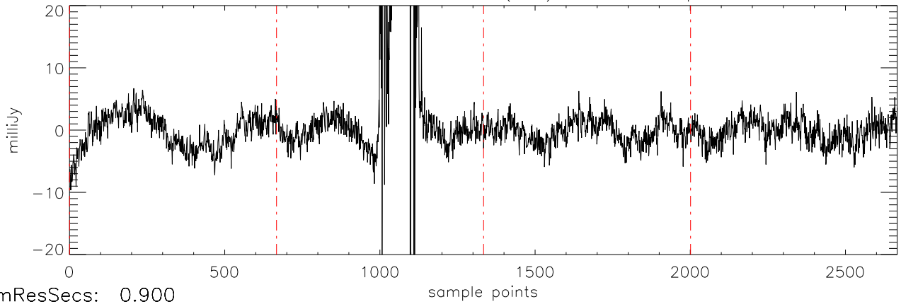
a2471 J16241436 09mar12 (AST) StokesQ freq:4466.
