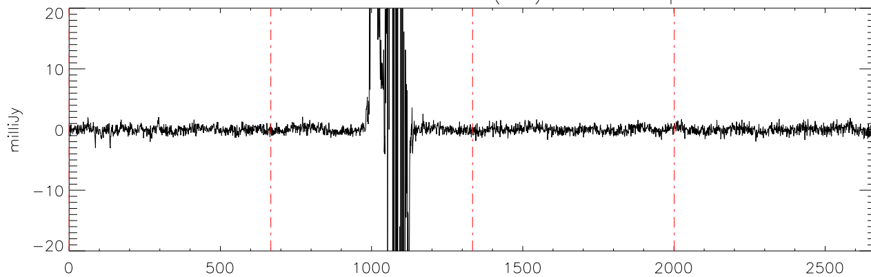
a2471 J16241436 09mar12 (AST) StokesV freq:4325.
