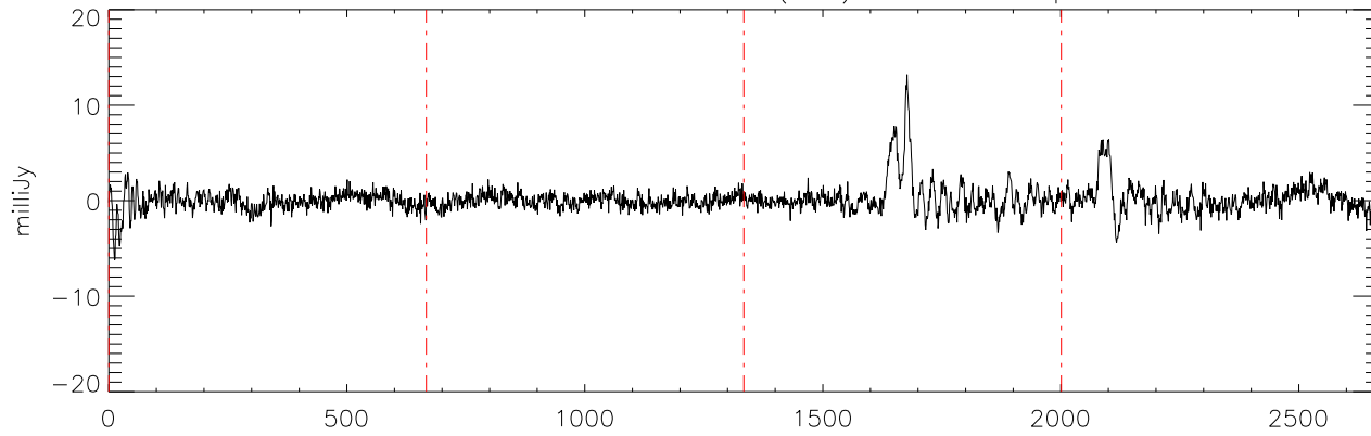
a2471 J16241436 09mar12 (AST) StokesV freq:4750.
