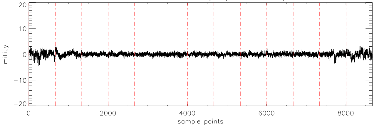
a2471 J14243909 07feb12 (AST) StokesV freq:5176.
