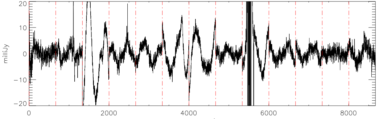
a2471 J14243909 07feb12 (AST) StokesQ freq:4325.
