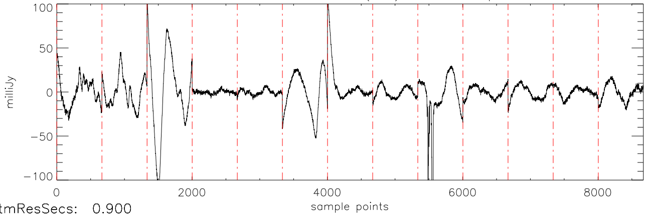
α2471 J14243909 07feb12 (AST) StokesI freq:5034.
