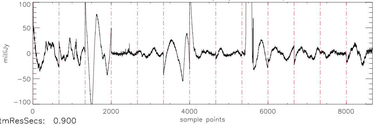
\alpha 2471 J14243909 07feb12 (AST) StokesI freq:4466.
