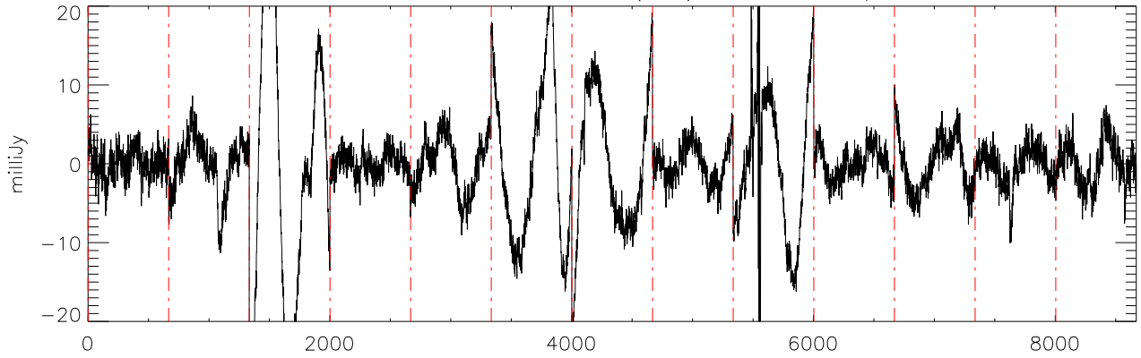
a2471 J14243909 07feb12 (AST) StokesQ freq:4750.
