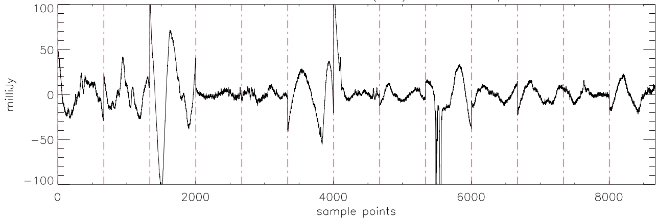
\alpha 2471 J14243909 07feb12 (AST) StokesI freq:4750.
