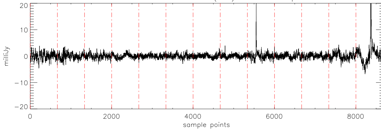
a2471 J14243909 07feb12 (AST) StokesU freq:5176.
