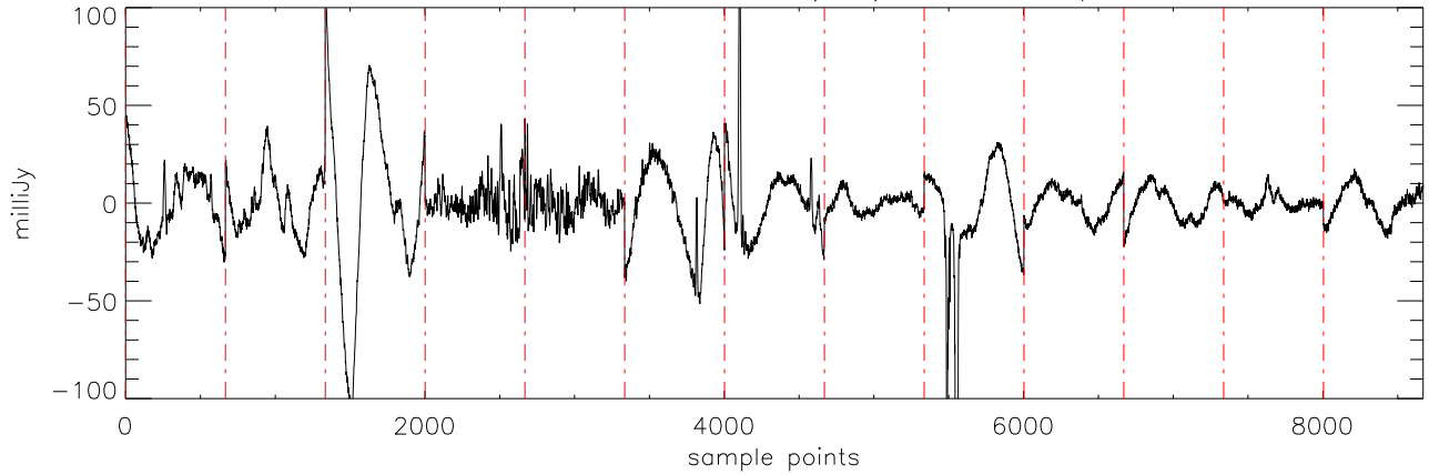
\alpha 2471 J14243909 07feb12 (AST) StokesI freq:4750.
