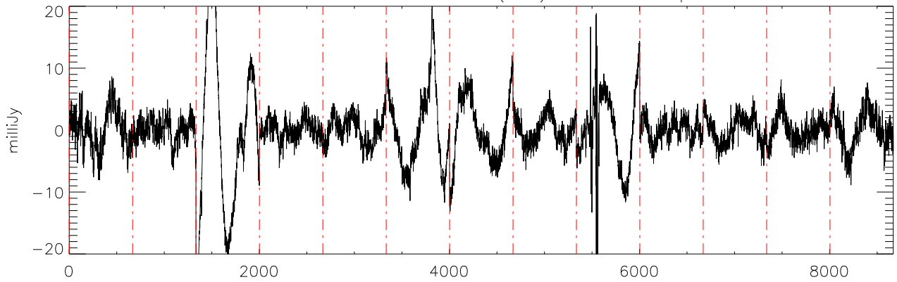
a2471 J14243909 07feb12 (AST) StokesQ freq:4466.
