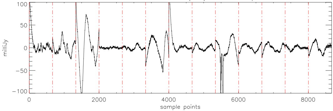
\alpha 2471 J14243909 07feb12 (AST) StokesI freq:4608.
