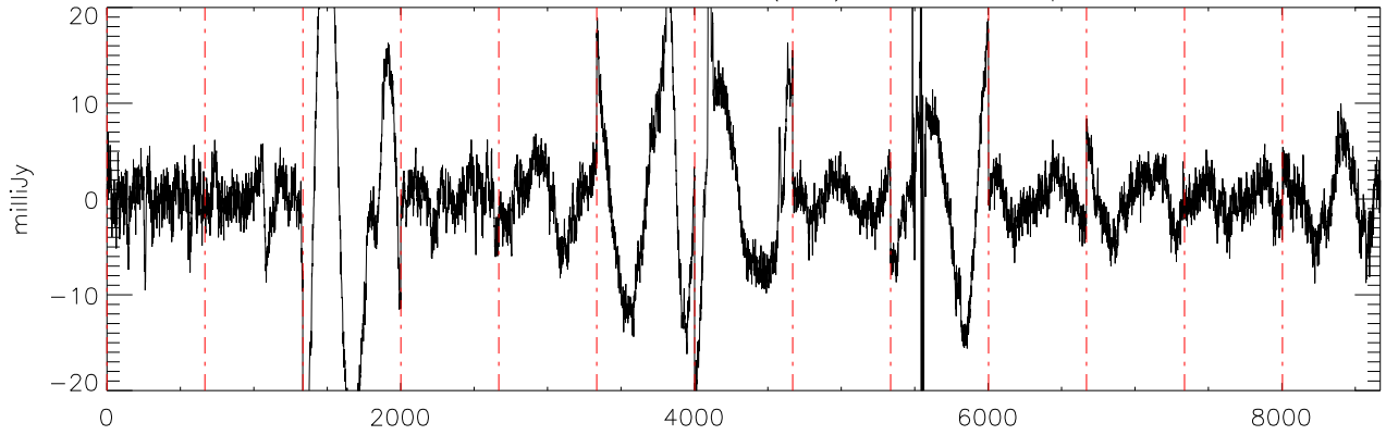
a2471 J14243909 07feb12 (AST) StokesQ freq:4608.
