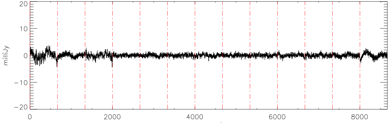
a2471 J14243909 07feb12 (AST) StokesV freq:4892.
