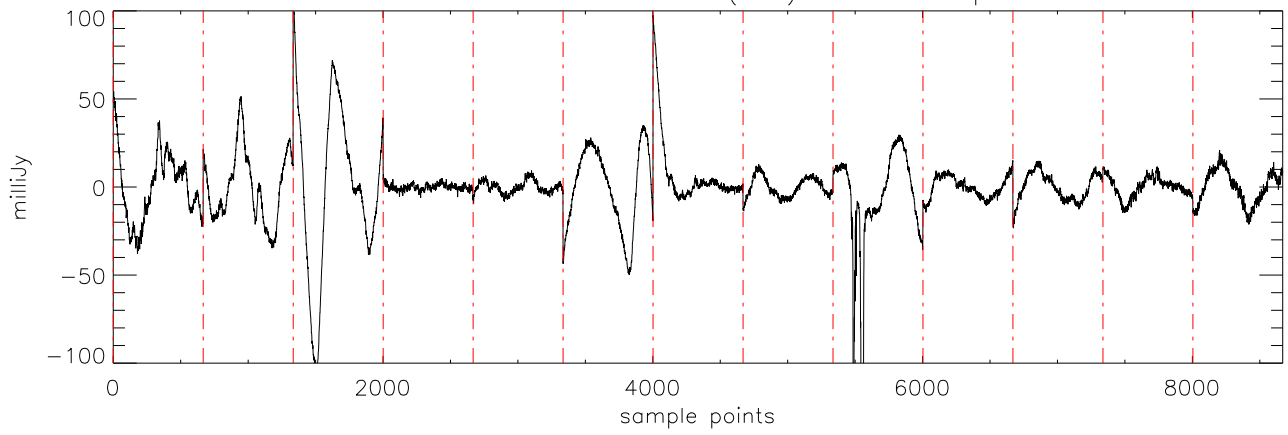
α2471 J14243909 07feb12 (AST) StokesI freq:5176.
