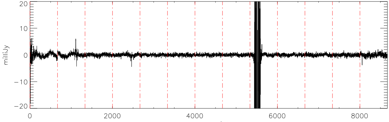
a2471 J14243909 07feb12 (AST) StokesV freq:4325.
