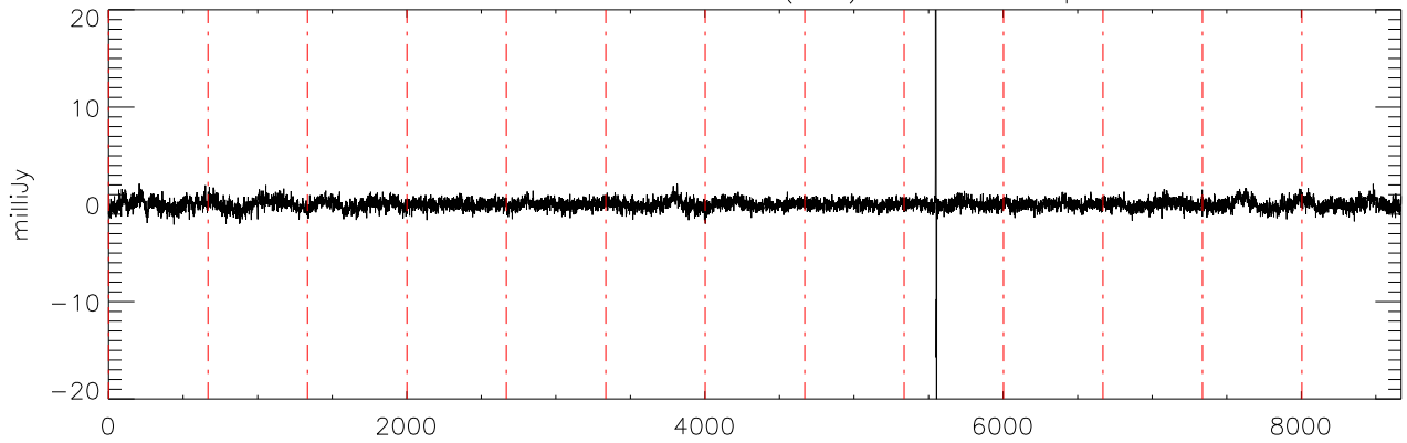
a2471 J14243909 07feb12 (AST) StokesV freq:4466.
