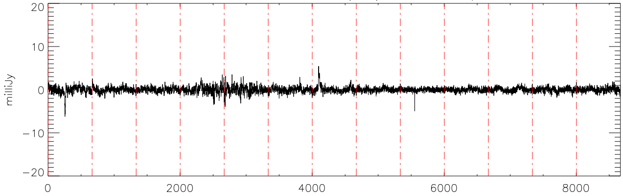
a2471 J14243909 07feb12 (AST) StokesV freq:4608.
