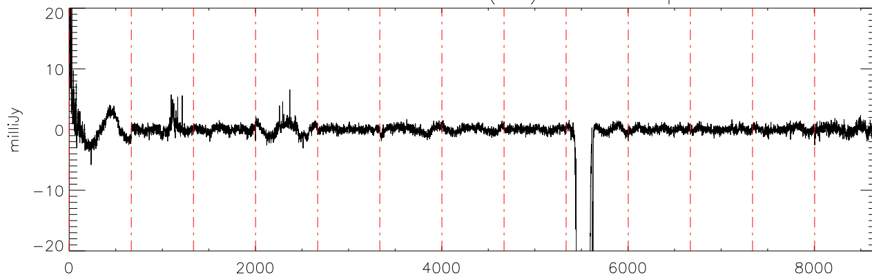
a2471 J14243909 07feb12 (AST) StokesU freq:4325.
