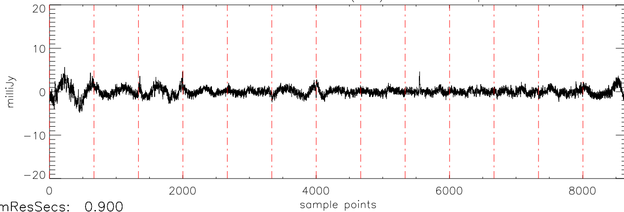
a2471 J14243909 07feb12 (AST) StokesU freq:5034.
