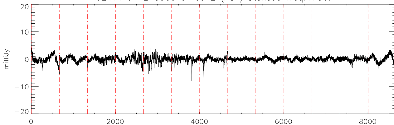
a2471 J14243909 07feb12 (AST) StokesU freq:4750.
