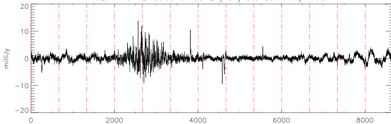
a2471 J14243909 07feb12 (AST) StokesU freq:4608.
