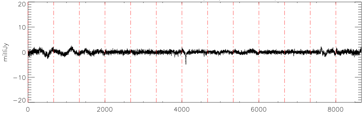
a2471 J14243909 07feb12 (AST) StokesV freq:4750.
