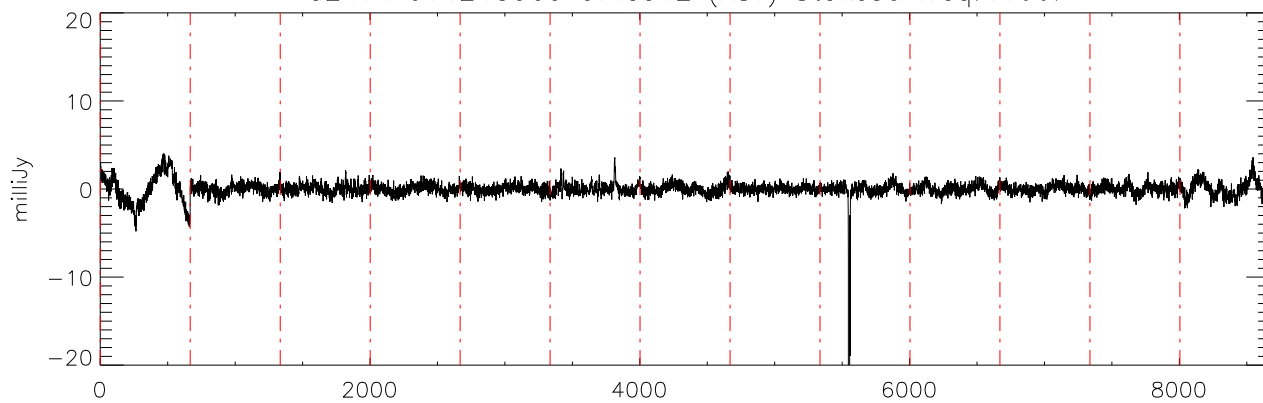
a2471 J14243909 07feb12 (AST) StokesU freq:4466.
