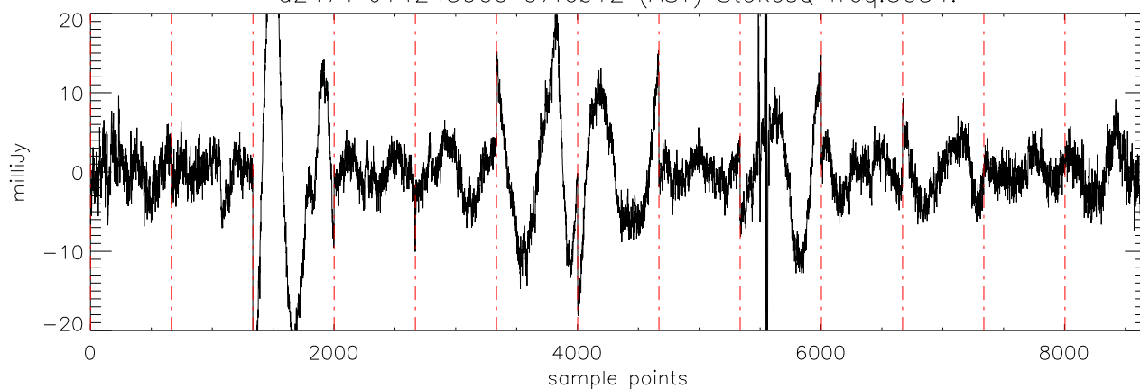
a2471 J14243909 07feb12 (AST) StokesQ freq:5176.
