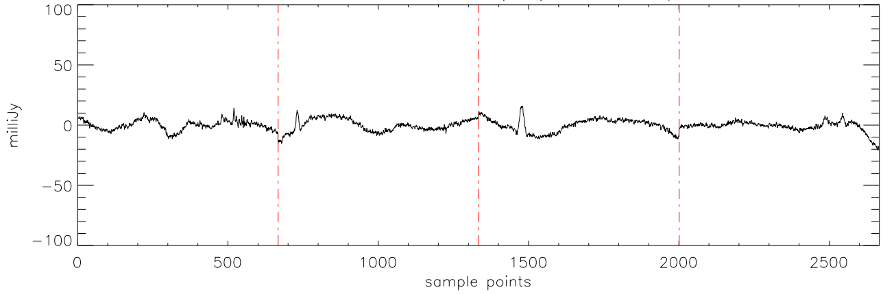
α2471 J10475385 08feb11 (AST) StokesI freq:4750.
