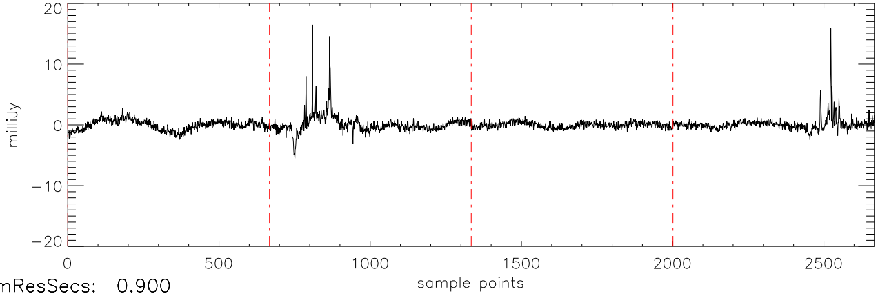
a2471 J10475385 08feb11 (AST) StokesU freq:4466.
