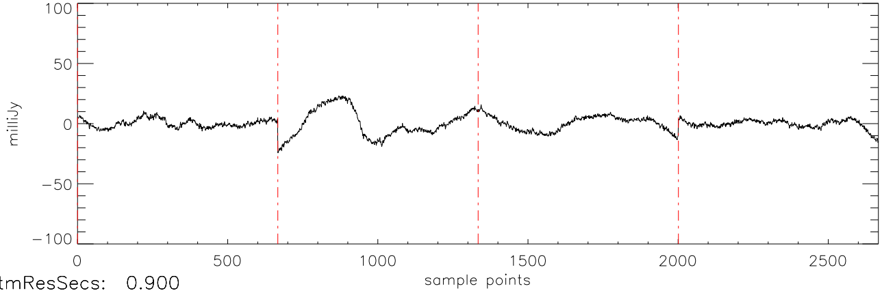
α2471 J10475385 08feb11 (AST) StokesI freq:5034.
