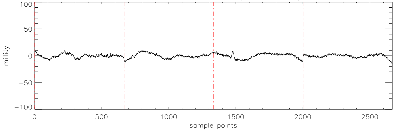
α2471 J10475385 08feb11 (AST) StokesI freq:4750.
