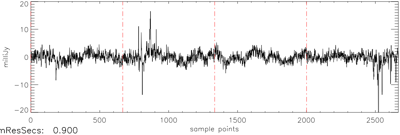
a2471 J10475385 08feb11 (AST) StokesQ freq:4466.
