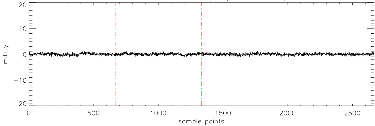
a2471 J10475385 08feb11 (AST) StokesV freq:4608.
