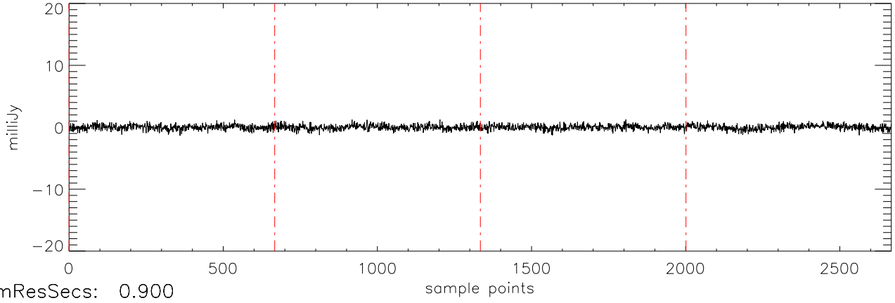
a2471 J10475385 08feb11 (AST) StokesV freq:5034.
