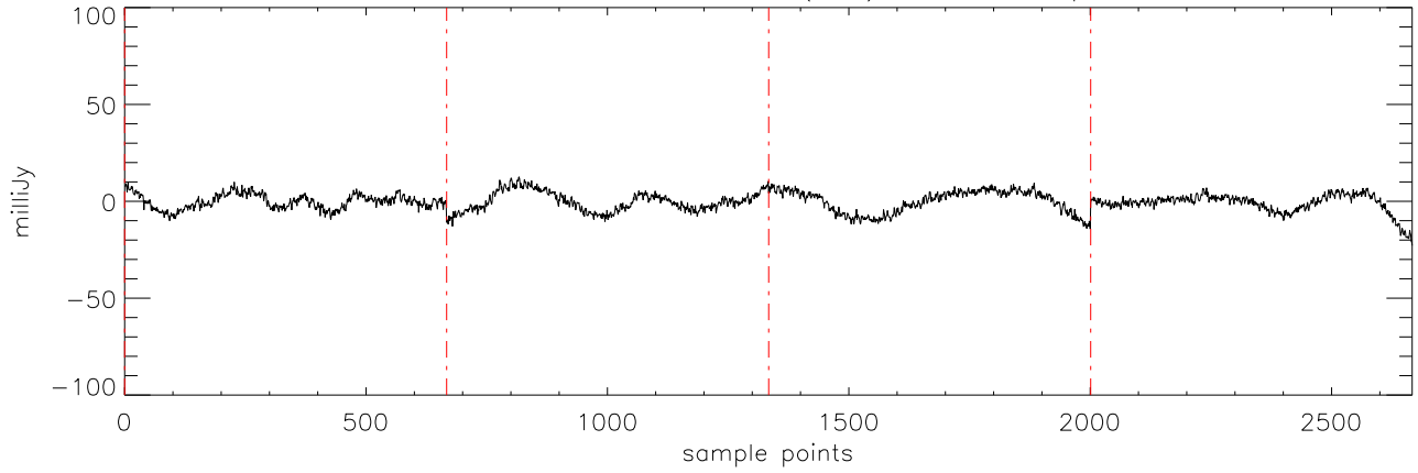
α2471 J10475385 08feb11 (AST) StokesI freq:5176.
