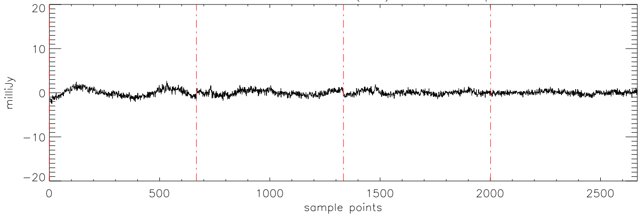
a2471 J10475385 08feb11 (AST) StokesU freq:4750.
