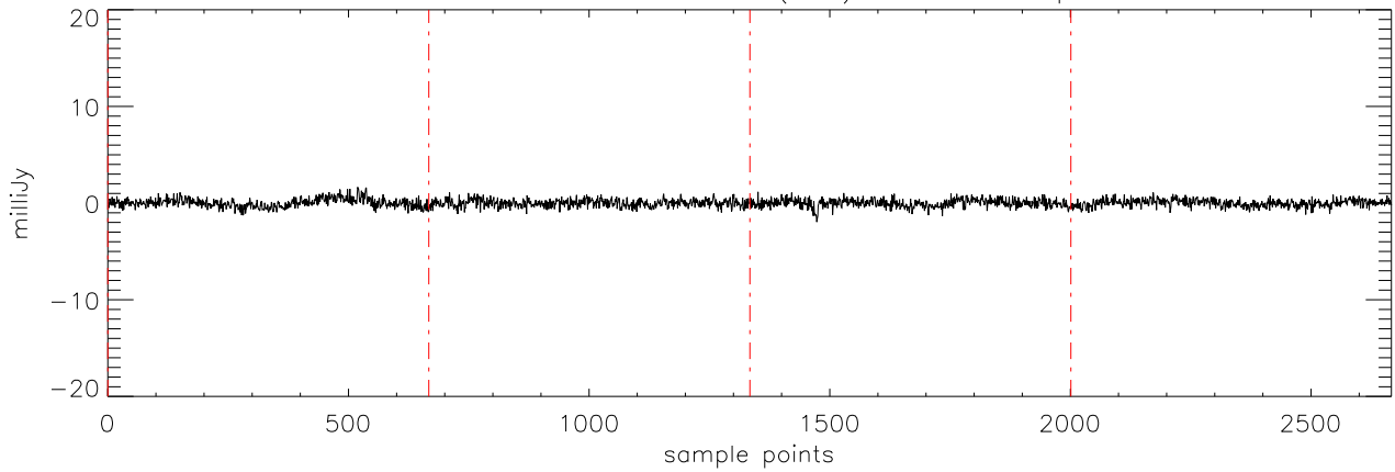
a2471 J10475385 08feb11 (AST) StokesV freq:4750.
