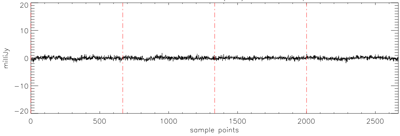
a2471 J10475385 08feb11 (AST) StokesV freq:5176.
