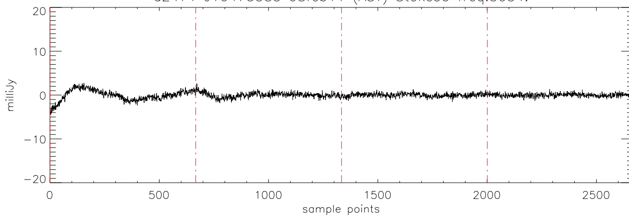
a2471 J10475385 08feb11 (AST) StokesU freq:5176.
