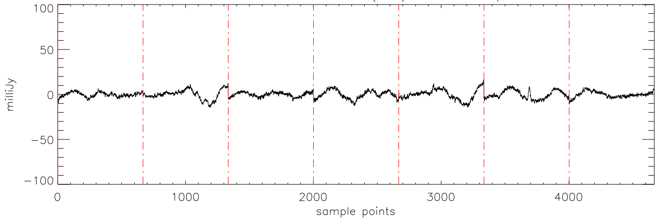
a2471 J10475385 07feb11 (AST) StokesI freq:4750.
