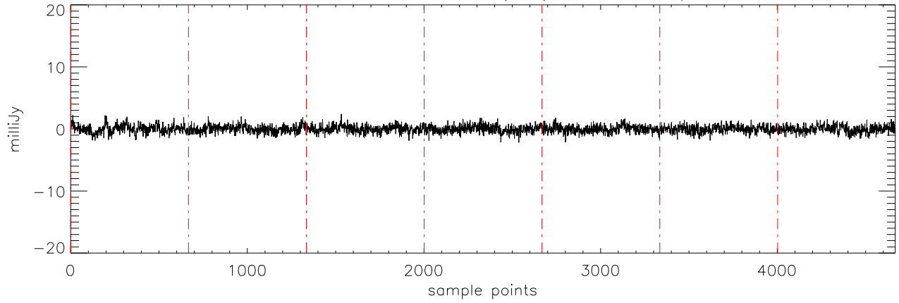
a2471 J10475385 07feb11 (AST) StokesV freq:5176.
