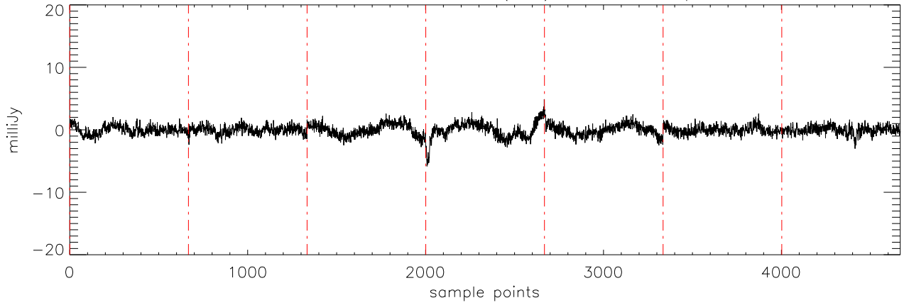
a2471 J10475385 07feb11 (AST) StokesU freq:5176.
