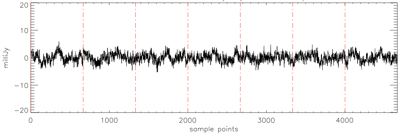
a2471 J10475385 07feb11 (AST) StokesQ freq:4608.
