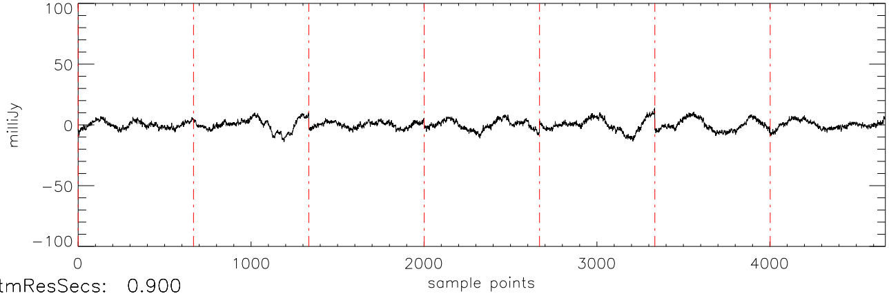
a2471 J10475385 07feb11 (AST) StokesI freq:5034.
