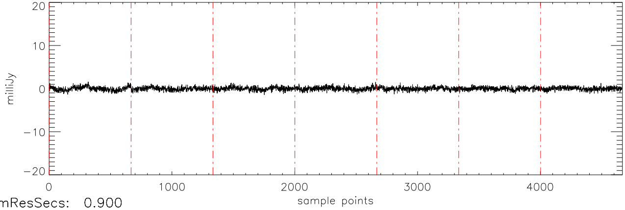
a2471 J10475385 07feb11 (AST) StokesV freq:5034.
