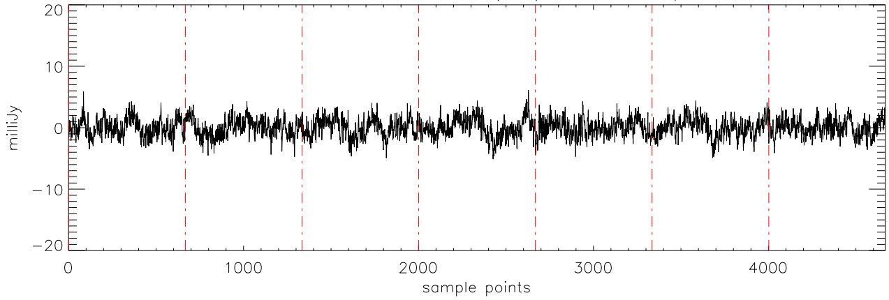
a2471 J10475385 07feb11 (AST) StokesQ freq:4750.
