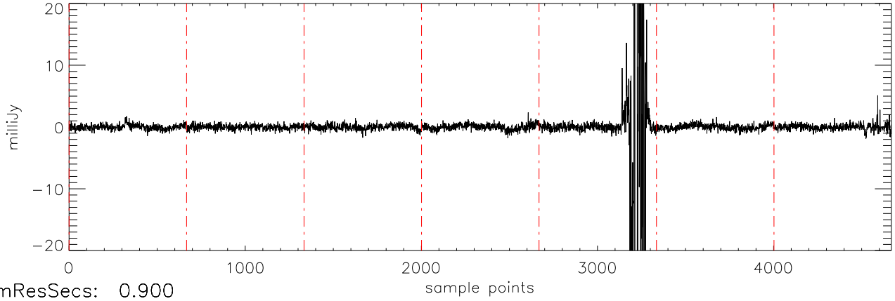
a2471 J10475385 07feb11 (AST) StokesV freq:4466.
