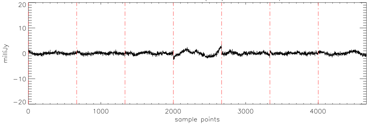
a2471 J10475385 07feb11 (AST) StokesU freq:4608.
