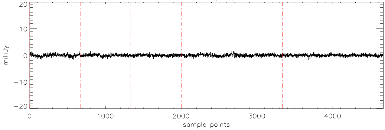
a2471 J10475385 07feb11 (AST) StokesV freq:4750.
