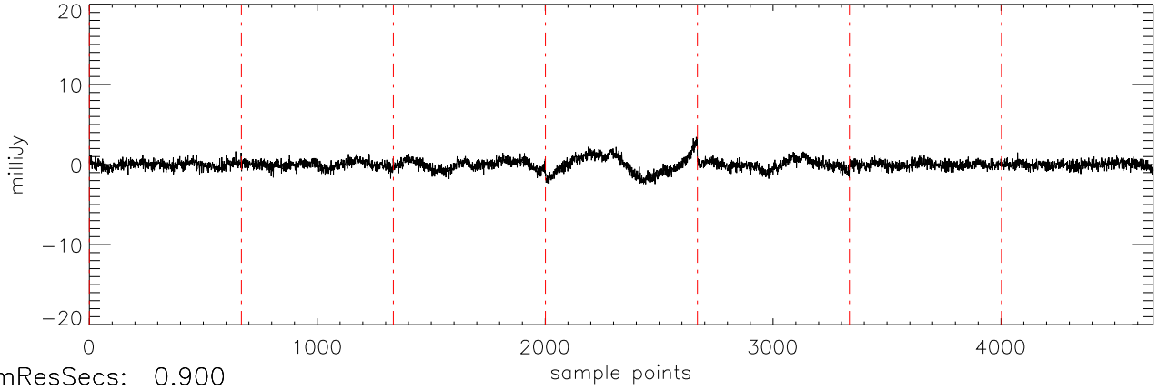
a2471 J10475385 07feb11 (AST) StokesU freq:5034.
