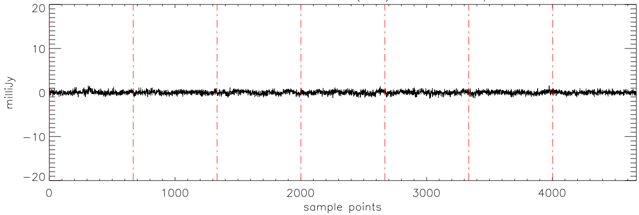
a2471 J10475385 07feb11 (AST) StokesV freq:4608.
