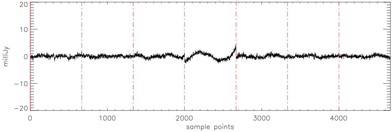
a2471 J10475385 07feb11 (AST) StokesU freq:4750.
