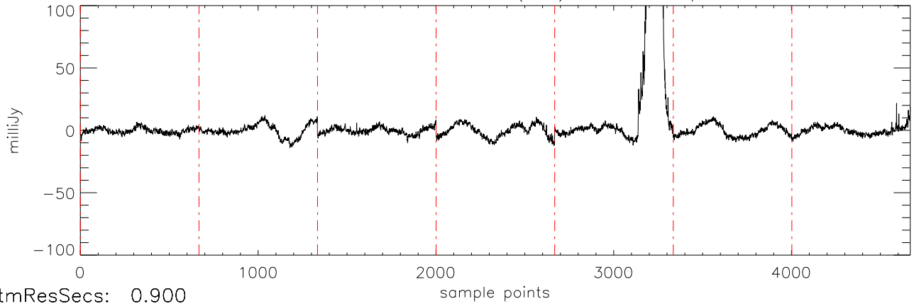
a2471 J10475385 07feb11 (AST) StokesI freq:4466.
