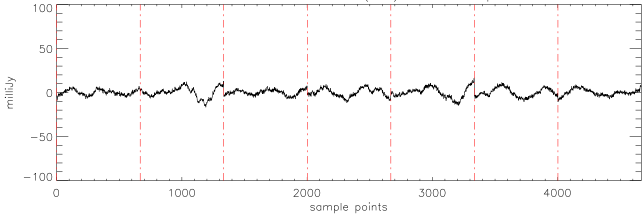
a2471 J10475385 07feb11 (AST) StokesI freq:5176.
