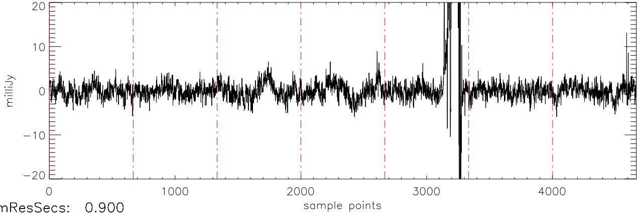
a2471 J10475385 07feb11 (AST) StokesQ freq:4466.
