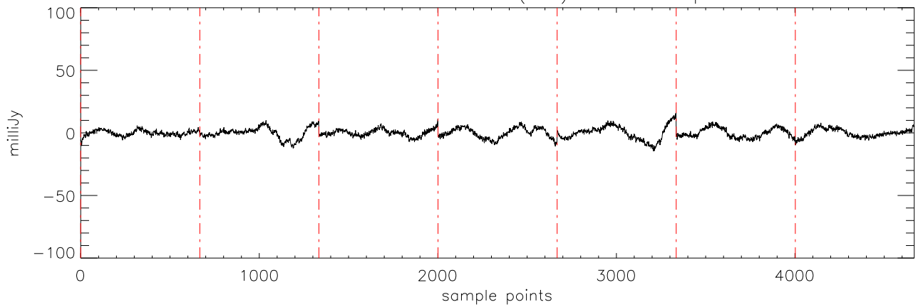
a2471 J10475385 07feb11 (AST) StokesI freq:4608.
