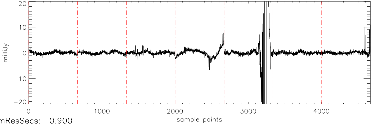
a2471 J10475385 07feb11 (AST) StokesU freq:4466.
