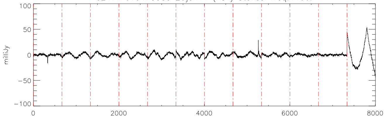
a2471 J10475385 20jan11 (AST) StokesI freq:4466.
