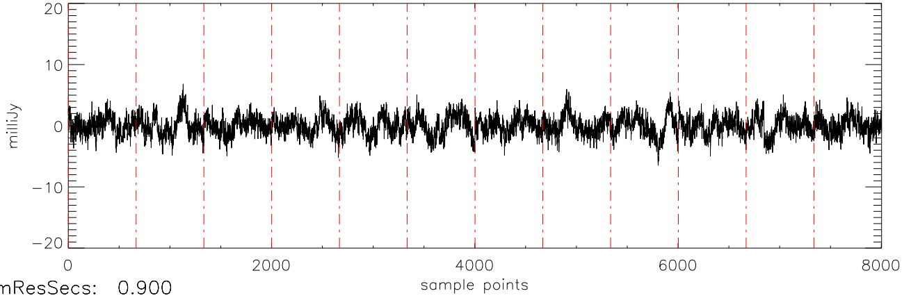
a2471 J10475385 20jan11 (AST) StokesQ freq:5034.
