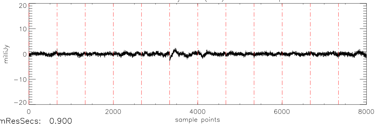
a2471 J10475385 20jan11 (AST) StokesU freq:5034.
