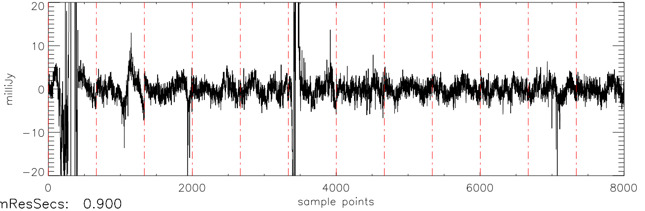
a2471 J10475385 20jan11 (AST) StokesQ freq:4466.
