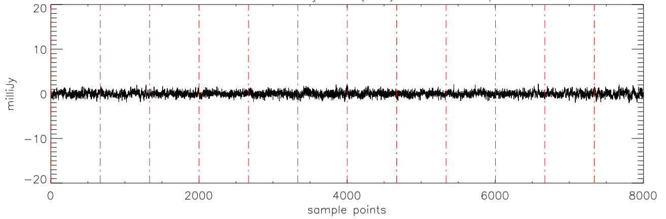
a2471 J10475385 20jan11 (AST) StokesV freq:5176.
