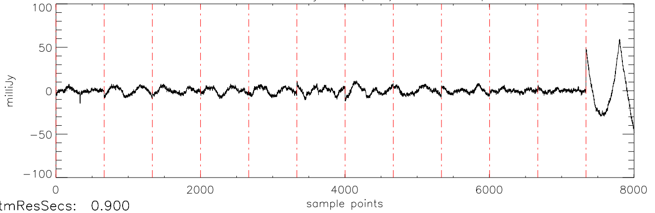
a2471 J10475385 20jan11 (AST) StokesI freq:5034.
