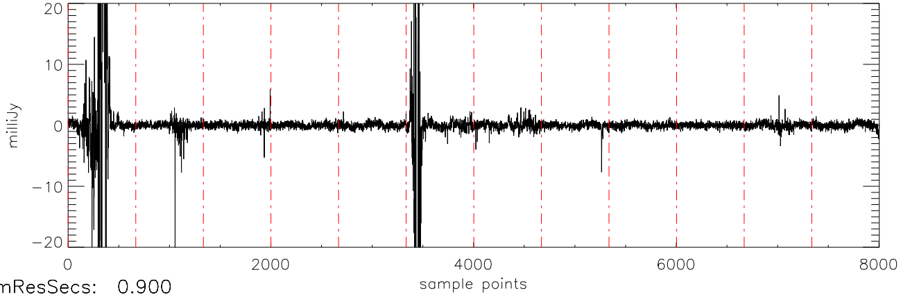
a2471 J10475385 20jan11 (AST) StokesV freq:4466.
