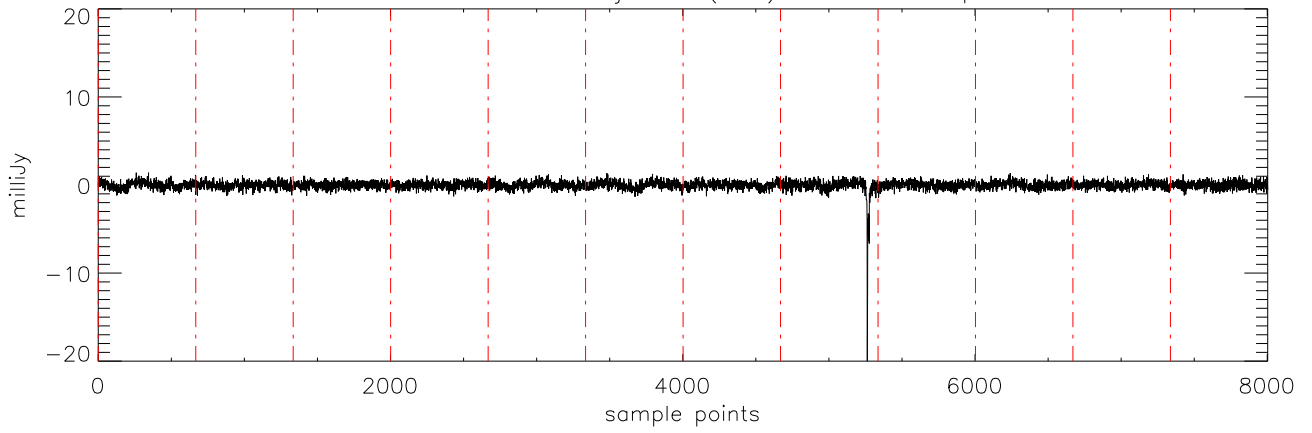
a2471 J10475385 20jan11 (AST) StokesV freq:4608.
