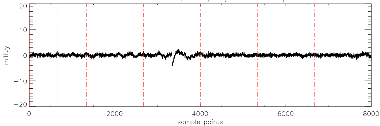
a2471 J10475385 20jan11 (AST) StokesU freq:5176.
