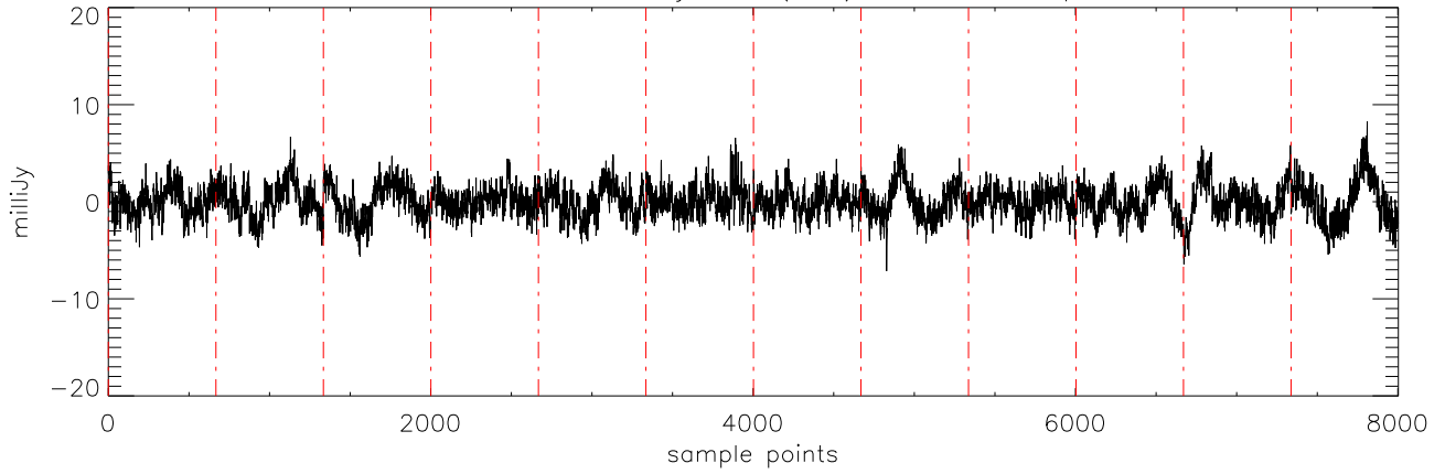
a2471 J10475385 20jan11 (AST) StokesQ freq:4750.
