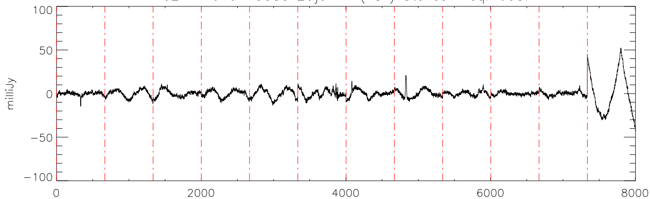
a2471 J10475385 20jan11 (AST) StokesI freq:4608.
