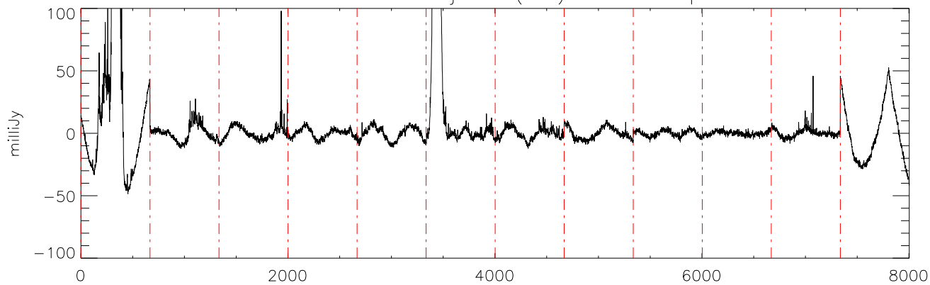
a2471 J10475385 20jan11 (AST) StokesI freq:4325.
