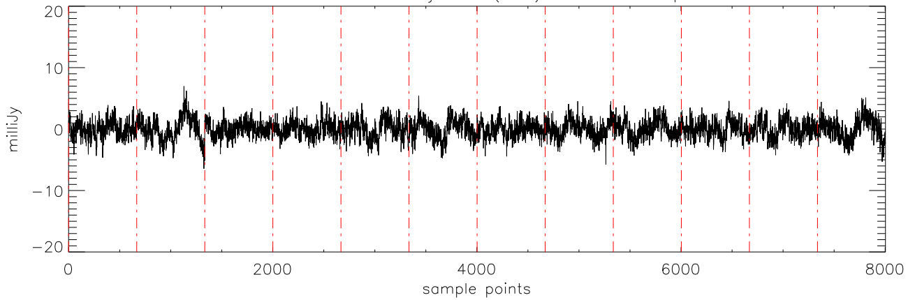
a2471 J10475385 20jan11 (AST) StokesQ freq:4608.
