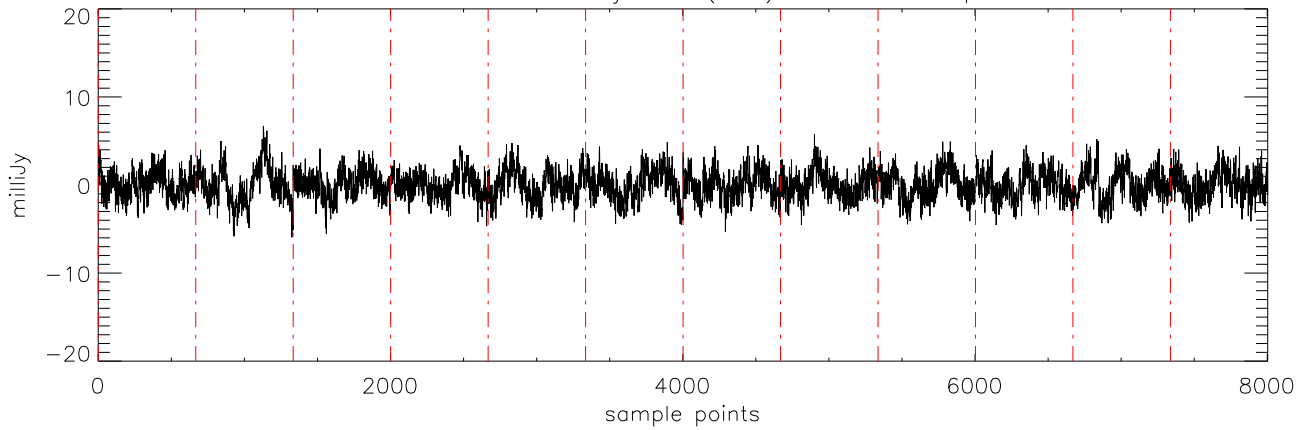
a2471 J10475385 20jan11 (AST) StokesQ freq:5176.
