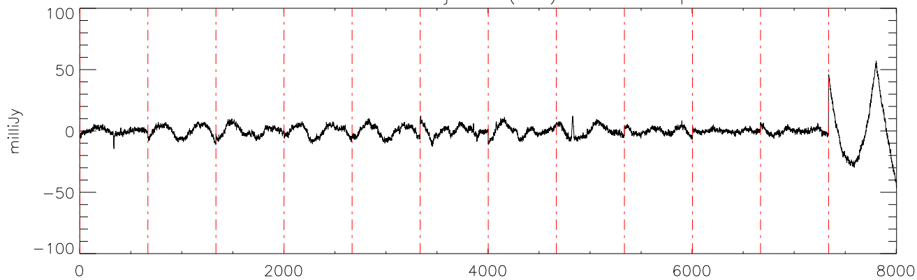
a2471 J10475385 20jan11 (AST) StokesI freq:4750.
