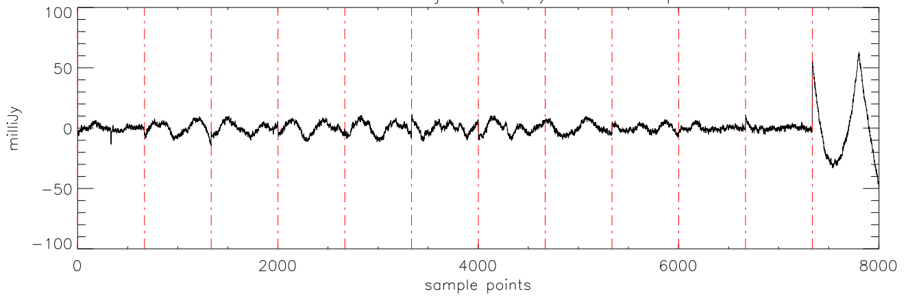
a2471 J10475385 20jan11 (AST) StokesI freq:5176.
