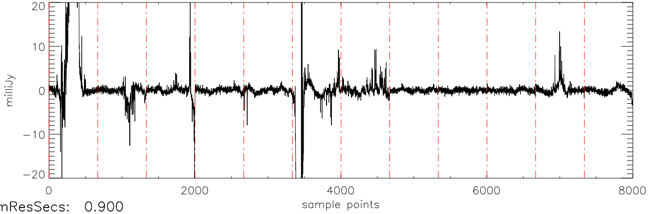
a2471 J10475385 20jan11 (AST) StokesU freq:4466.
