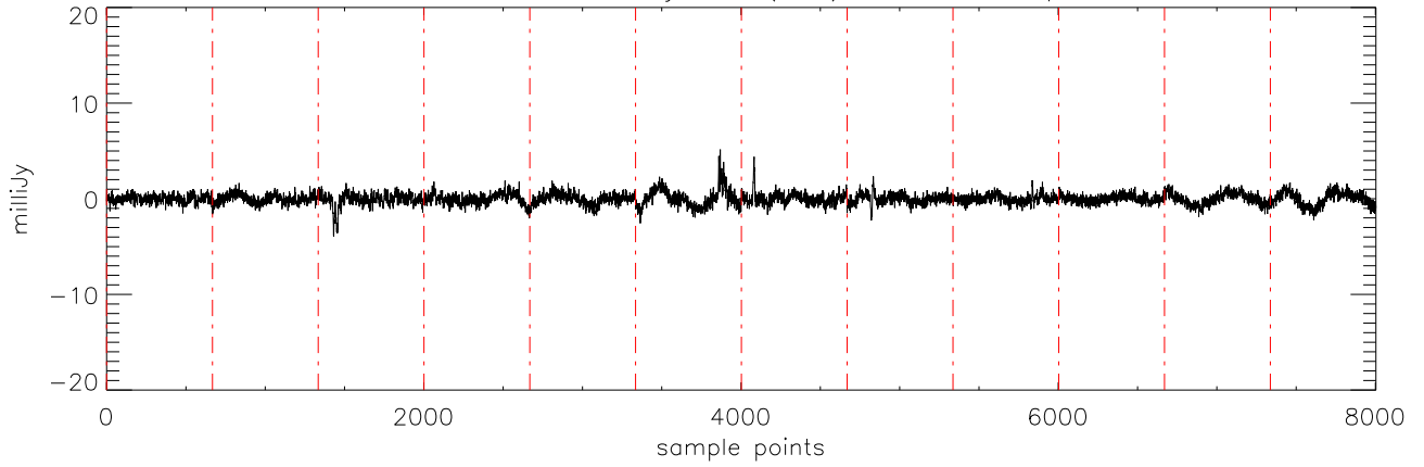
a2471 J10475385 20jan11 (AST) StokesU freq:4750.
