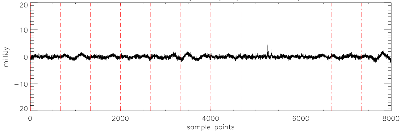
a2471 J10475385 20jan11 (AST) StokesU freq:4608.
