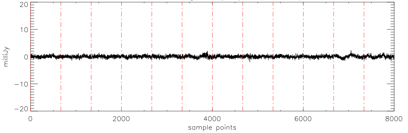
a2471 J10475385 20jan11 (AST) StokesV freq:4750.
