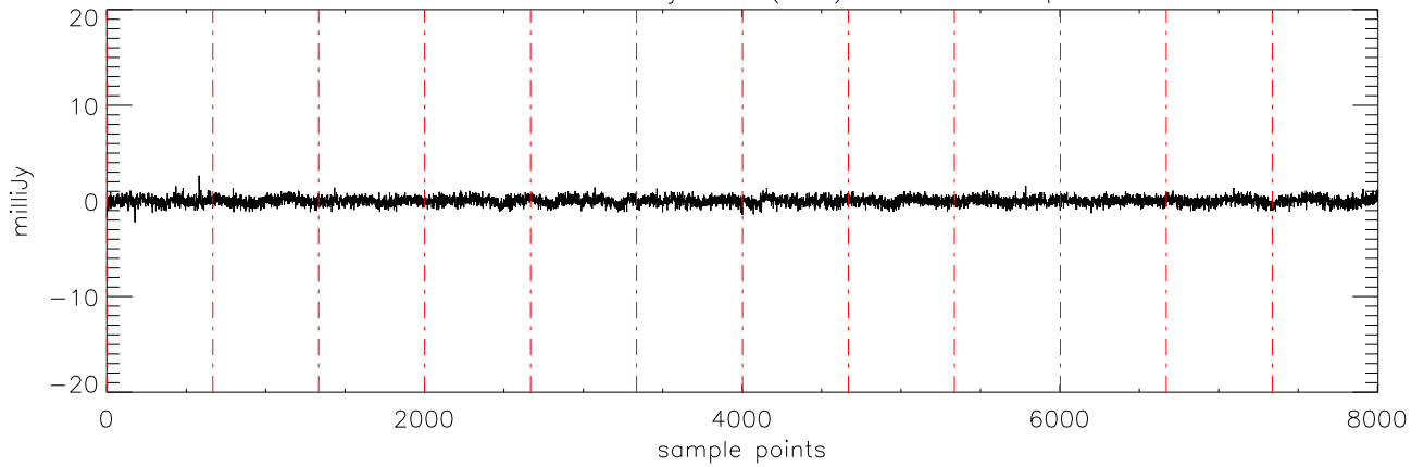
a2471 J10475385 02jan11 (AST) StokesV freq:4608.
