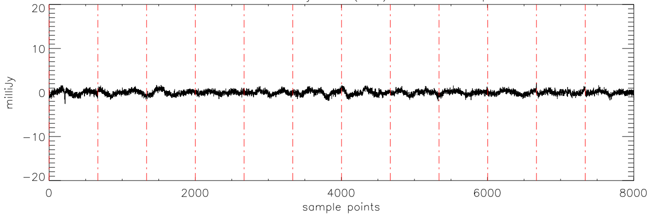
a2471 J10475385 02jan11 (AST) StokesU freq:4608.
