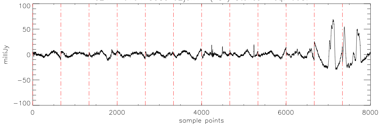
a2471 J10475385 02jan11 (AST) StokesI freq:4750.
