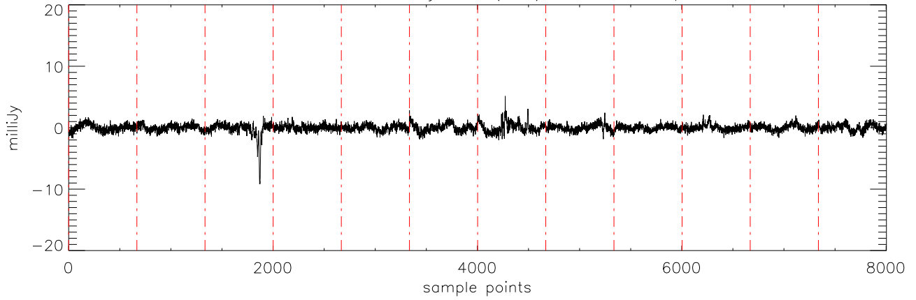
a2471 J10475385 02jan11 (AST) StokesU freq:4750.
