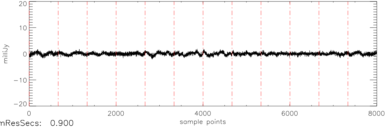
a2471 J10475385 02jan11 (AST) StokesU freq:5034.
