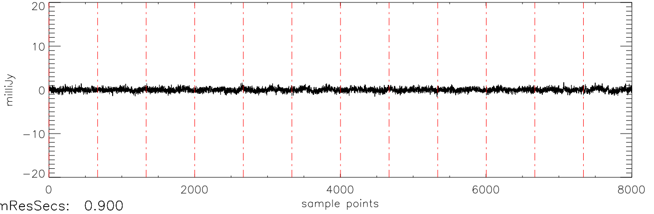
a2471 J10475385 02jan11 (AST) StokesV freq:5034.
