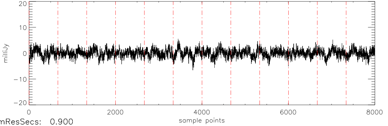
a2471 J10475385 02jan11 (AST) StokesQ freq:5034.
