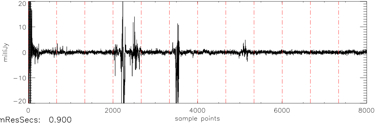
a2471 J10475385 02jan11 (AST) StokesV freq:4466.
