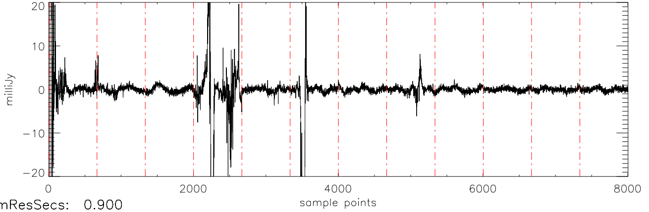
a2471 J10475385 02jan11 (AST) StokesU freq:4466.
