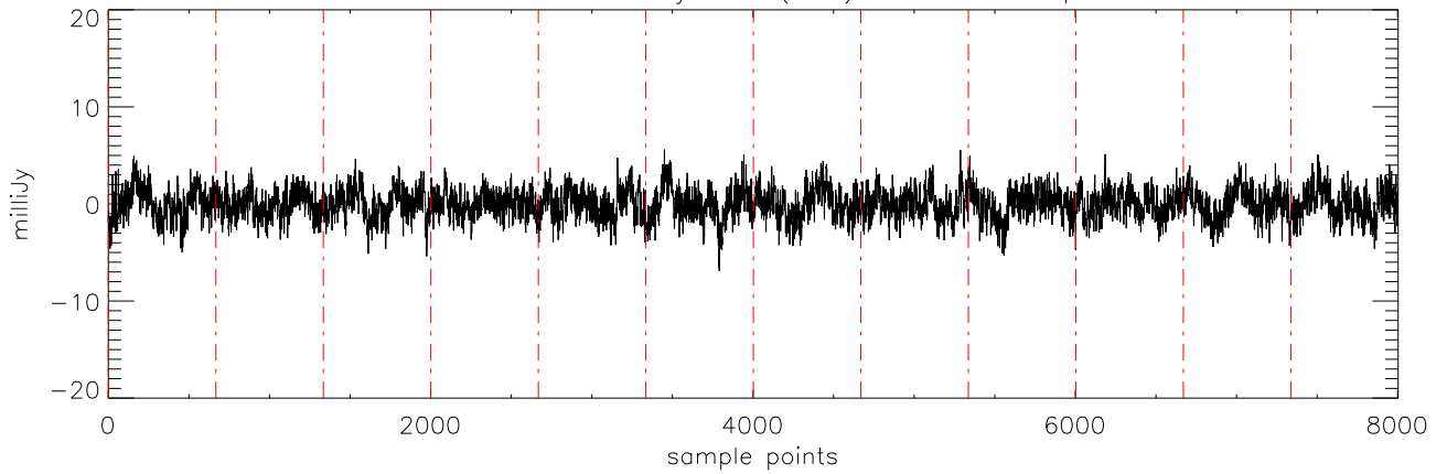
a2471 J10475385 02jan11 (AST) StokesQ freq:5176.
