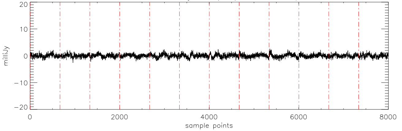
a2471 J10475385 02jan11 (AST) StokesU freq:5176.
