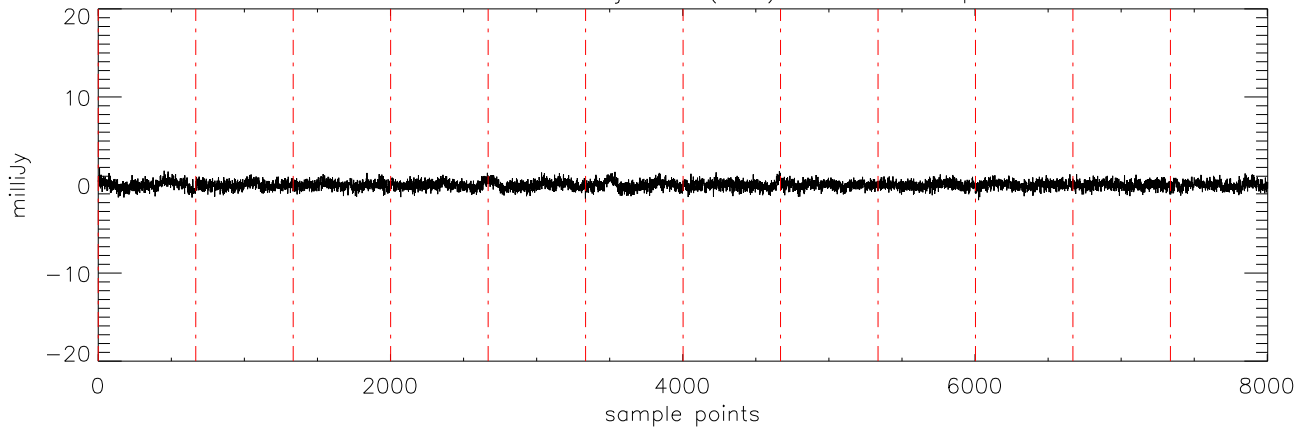
a2471 J10475385 02jan11 (AST) StokesV freq:5176.
