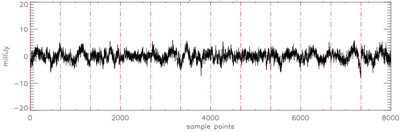
a2471 J10475385 02jan11 (AST) StokesQ freq:4750.
