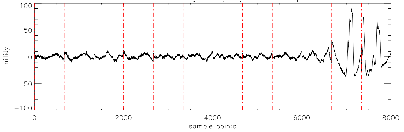
a2471 J10475385 02jan11 (AST) StokesI freq:5176.
