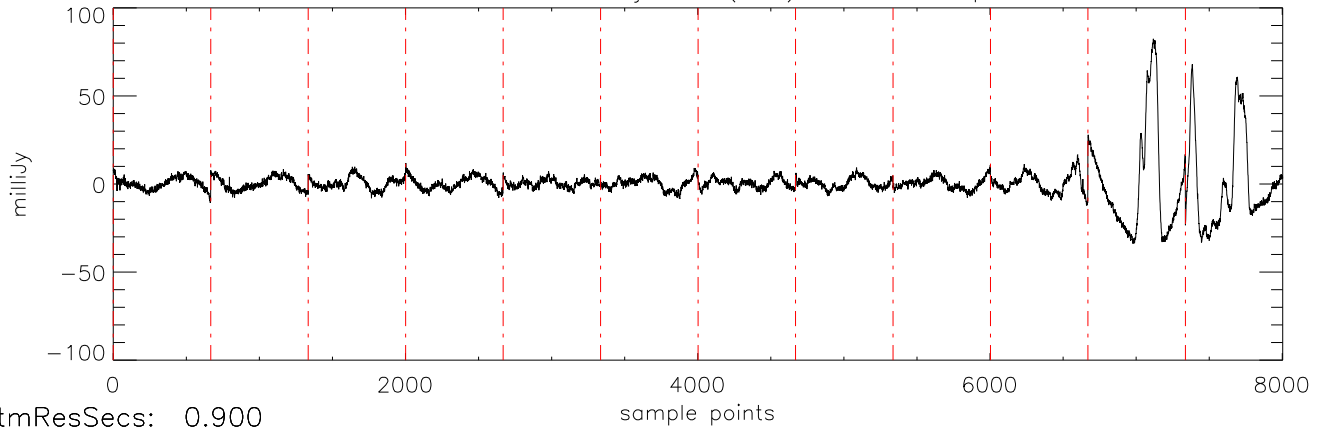
a2471 J10475385 02jan11 (AST) StokesI freq:5034.
