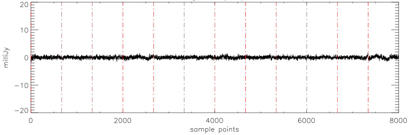
a2471 J10475385 02jan11 (AST) StokesV freq:4750.
