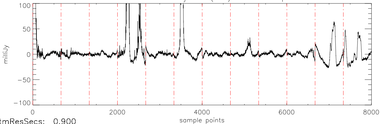
a2471 J10475385 02jan11 (AST) StokesI freq:4466.
