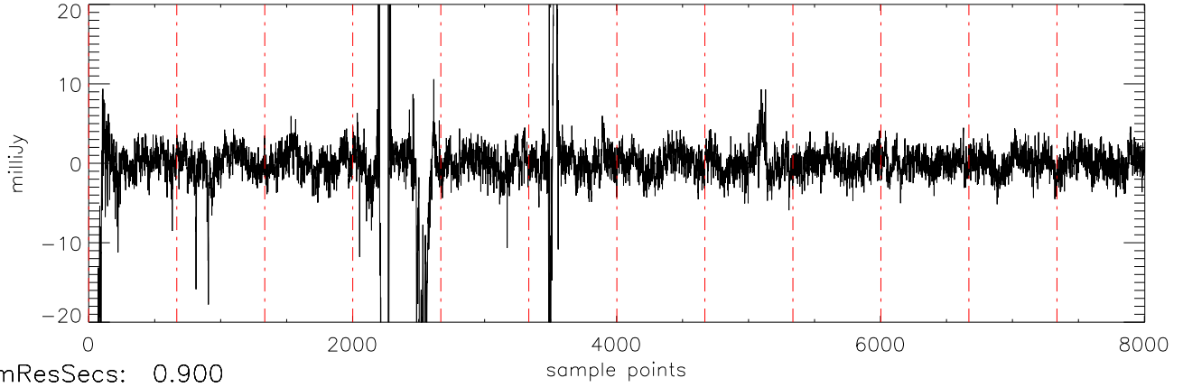
a2471 J10475385 02jan11 (AST) StokesQ freq:4466.
