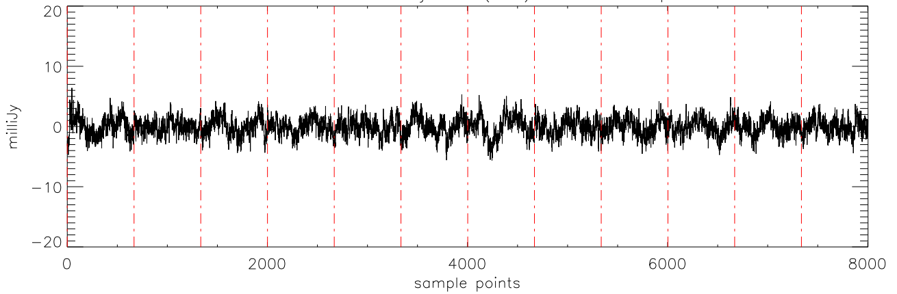
a2471 J10475385 02jan11 (AST) StokesQ freq:4608.
