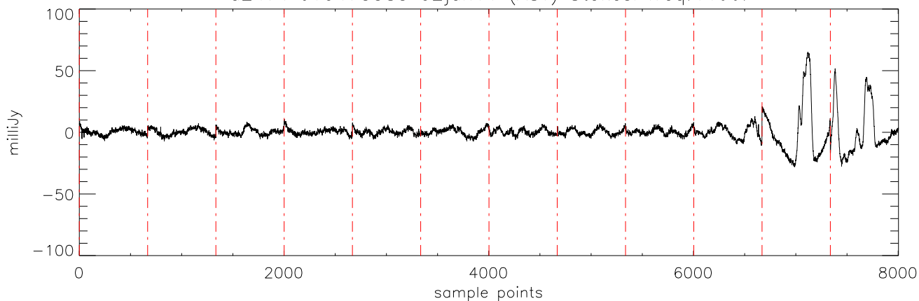
a2471 J10475385 02jan11 (AST) StokesI freq:4608.
