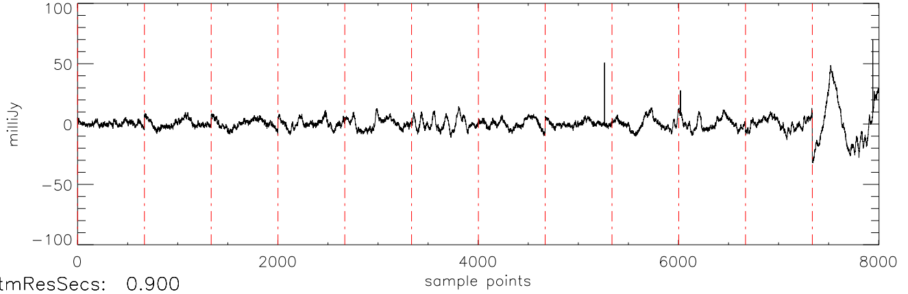
a2471 J10475385 07dec10 (AST) StokesI freq:5034.
