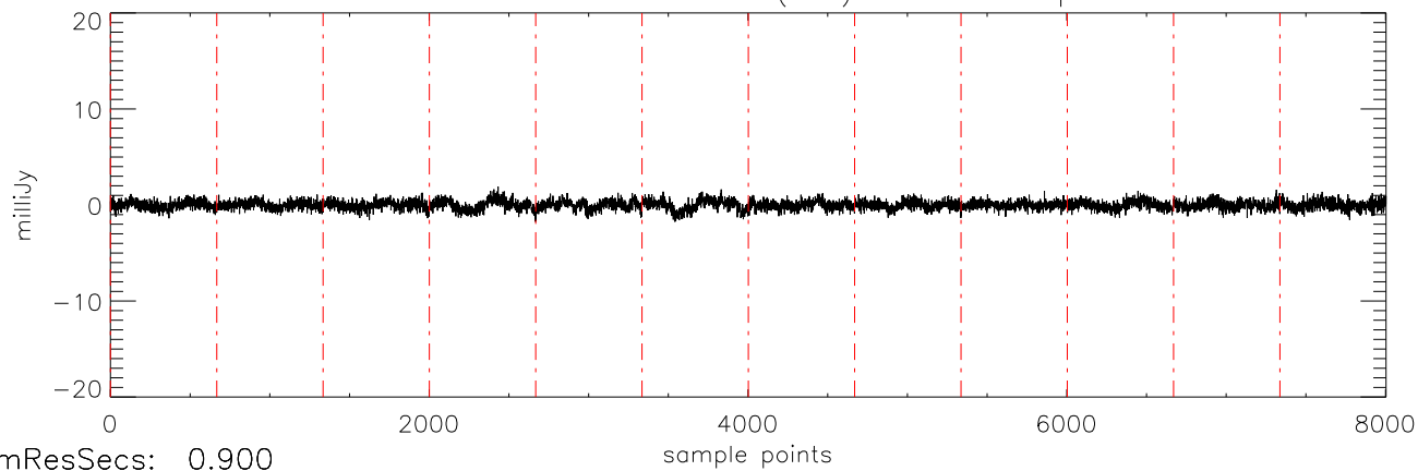
a2471 J10475385 07dec10 (AST) StokesU freq:5034.
