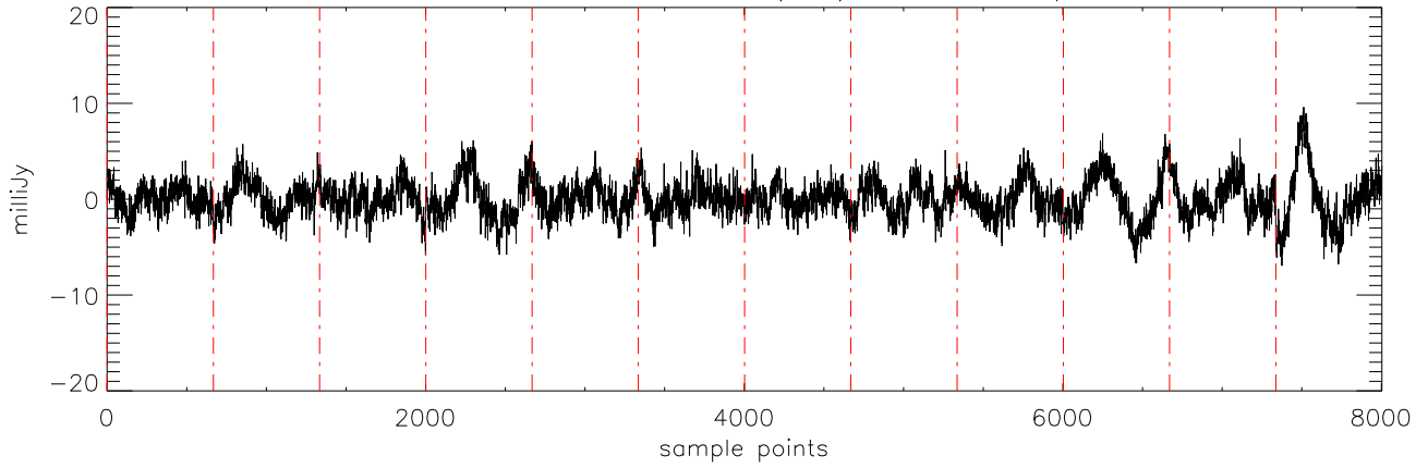
a2471 J10475385 07dec10 (AST) StokesQ freq:4750.
