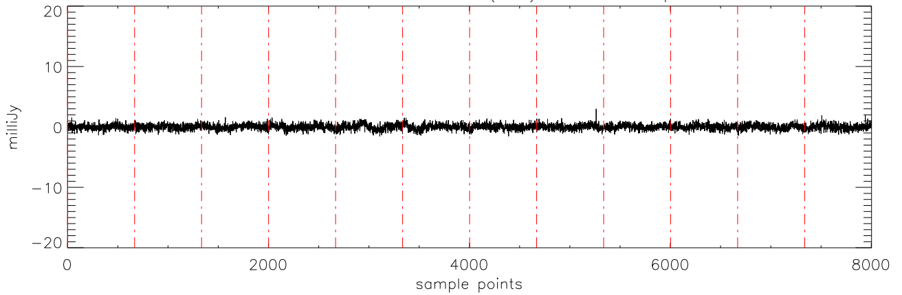
a2471 J10475385 07dec10 (AST) StokesV freq:5176.
