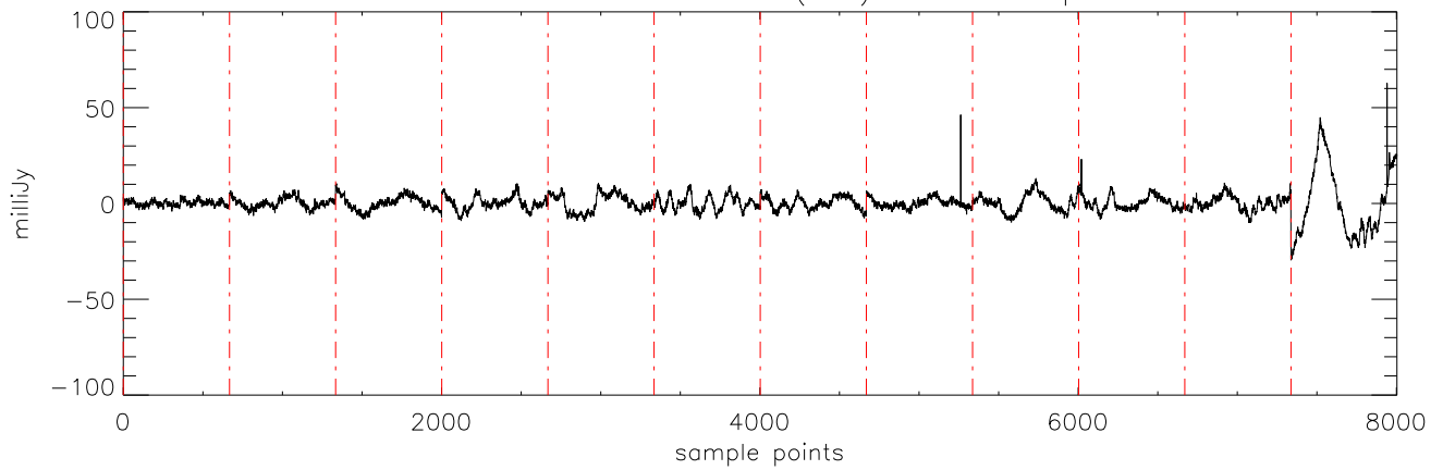
a2471 J10475385 07dec10 (AST) StokesI freq:4608.
