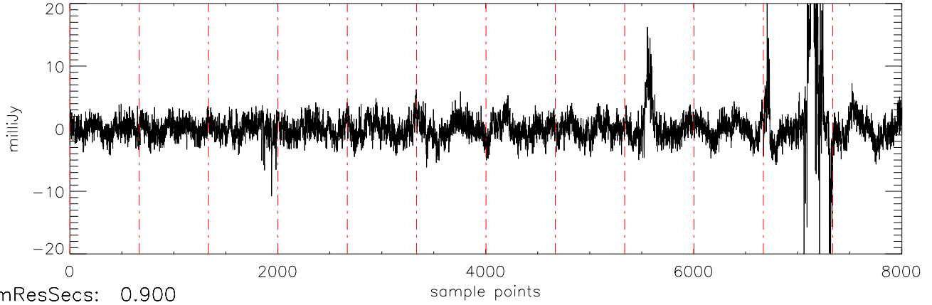
a2471 J10475385 07dec10 (AST) StokesQ freq:4466.
