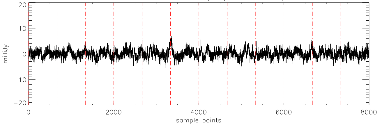
a2471 J10475385 07dec10 (AST) StokesQ freq:5176.
