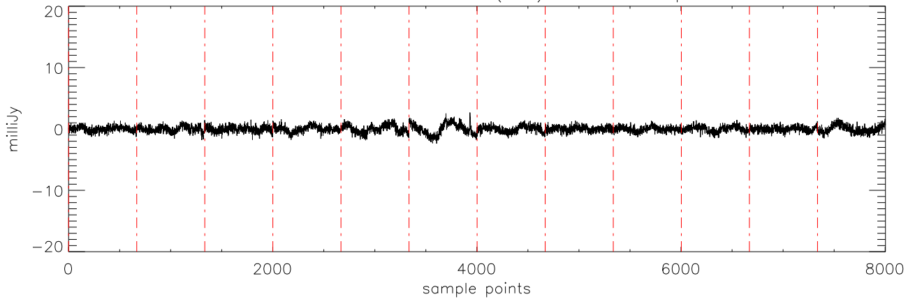
a2471 J10475385 07dec10 (AST) StokesU freq:4750.
