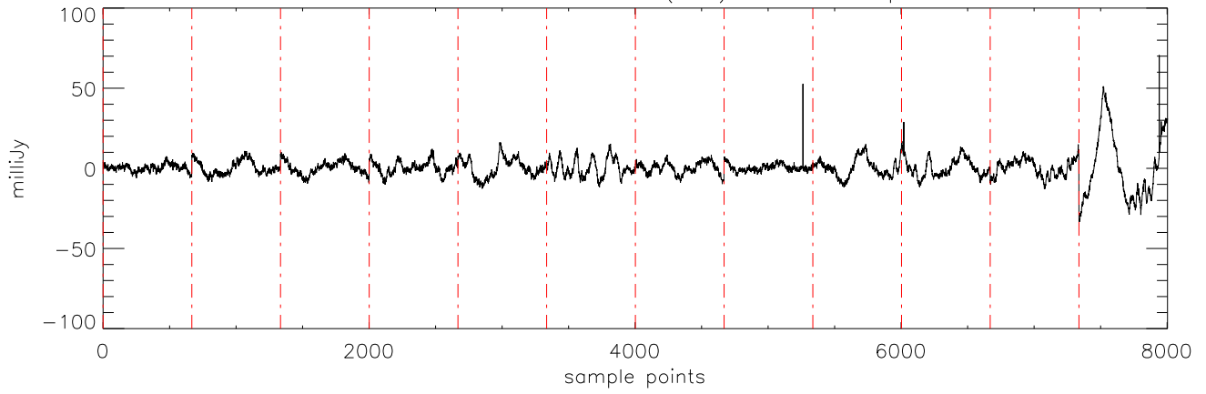
a2471 J10475385 07dec10 (AST) StokesI freq:5176.
