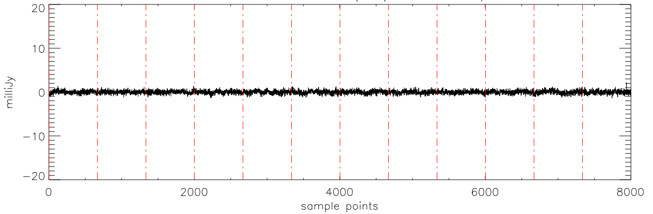
a2471 J10475385 07dec10 (AST) StokesV freq:4608.
