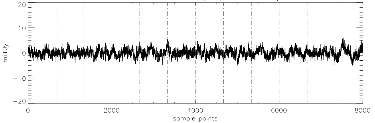
a2471 J10475385 07dec10 (AST) StokesQ freq:4608.
