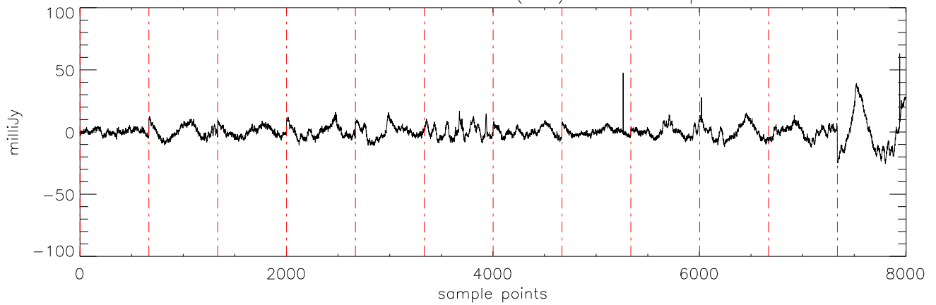
a2471 J10475385 07dec10 (AST) StokesI freq:4750.
