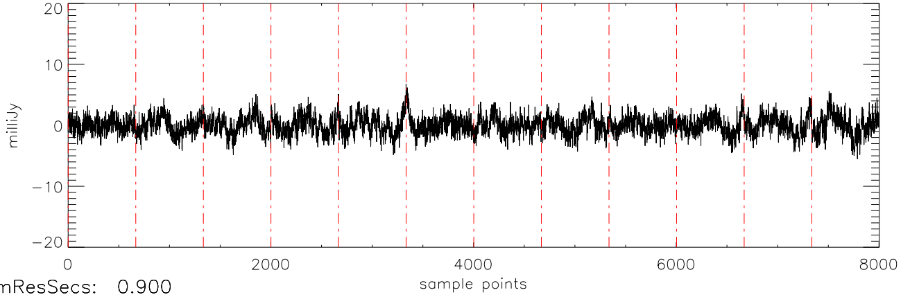
a2471 J10475385 07dec10 (AST) StokesQ freq:5034.
