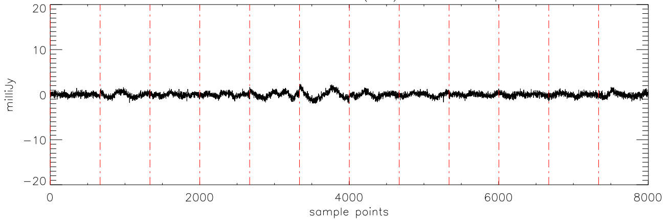
a2471 J10475385 07dec10 (AST) StokesU freq:4608.
