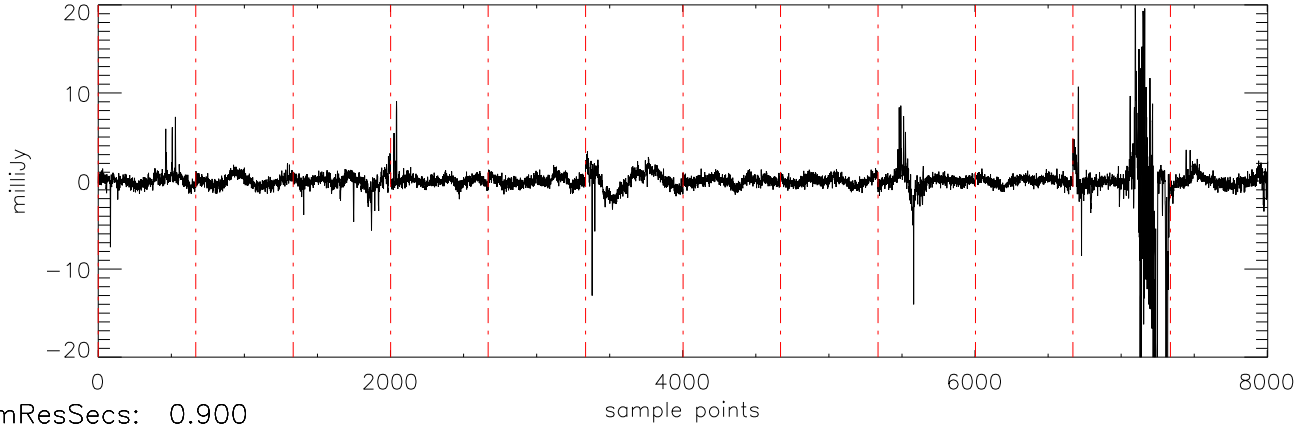
a2471 J10475385 07dec10 (AST) StokesU freq:4466.
