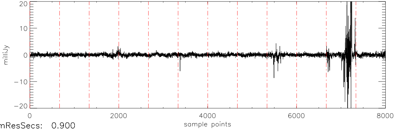
a2471 J10475385 07dec10 (AST) StokesV freq:4466.
