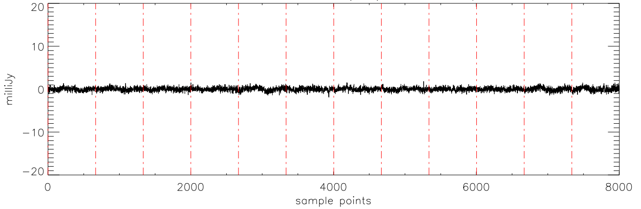
a2471 J10475385 07dec10 (AST) StokesV freq:4750.
