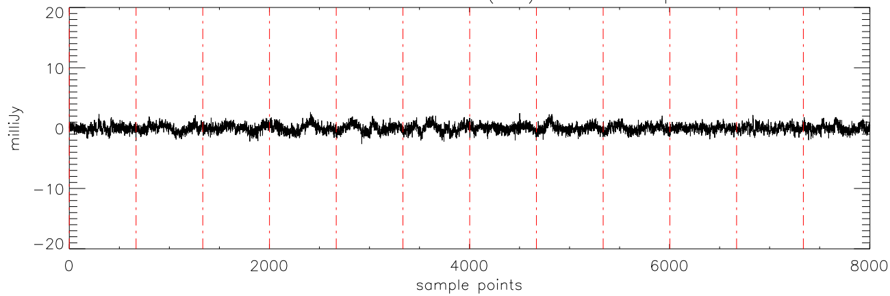
a2471 J10475385 07dec10 (AST) StokesU freq:5176.
