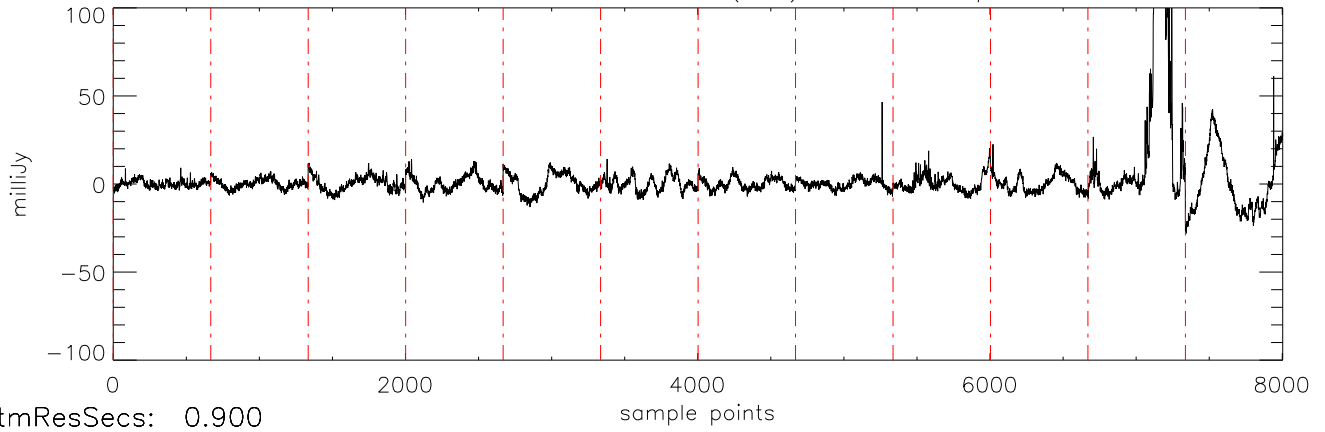
a2471 J10475385 07dec10 (AST) StokesI freq:4466.
