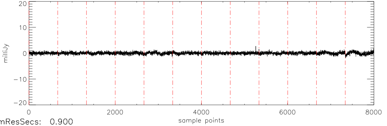
a2471 J10475385 07dec10 (AST) StokesV freq:5034.
