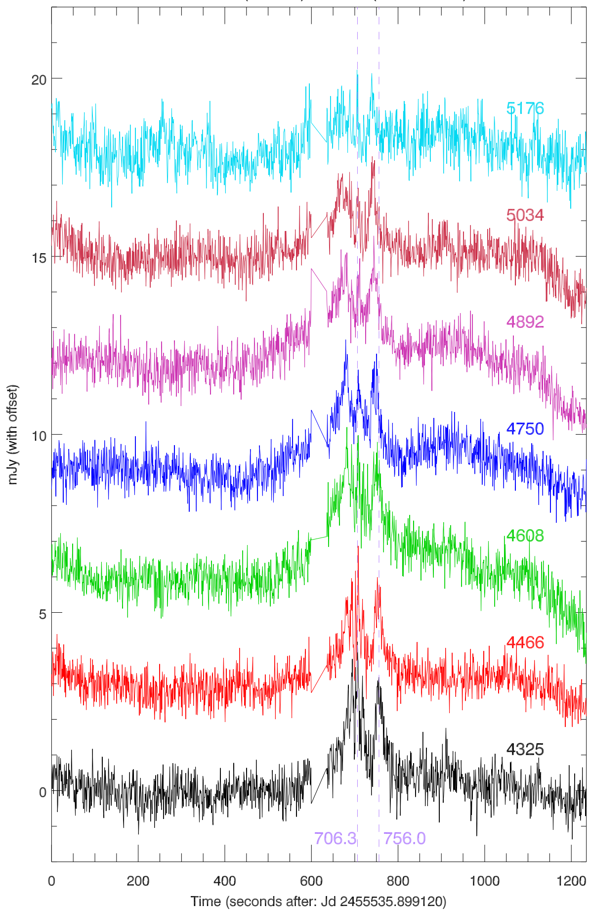
Stokes V (data-fit) vs time (with offsets)
