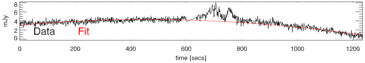
a2471 05dec10 Stokes V vs time during event. 4325 Mhz
