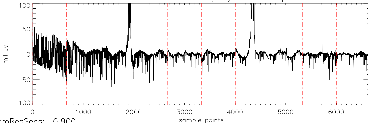
α2471 J10475385 02dec10 (AST) StokesI freq:4466.
