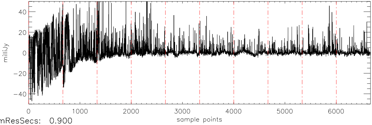
a2471 J10475385 02dec10 (AST) StokesQ freq:5034.
