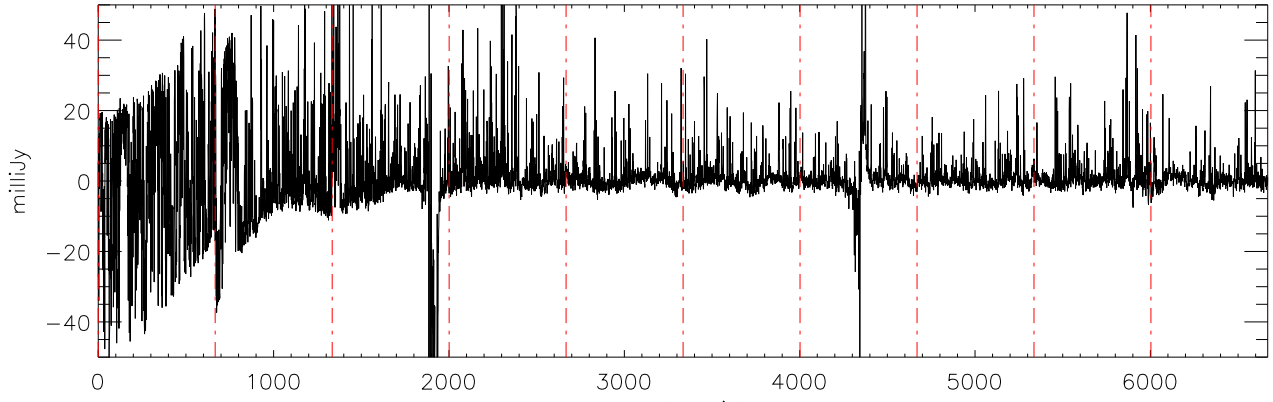
a2471 J10475385 02dec10 (AST) StokesQ freq:4325.
