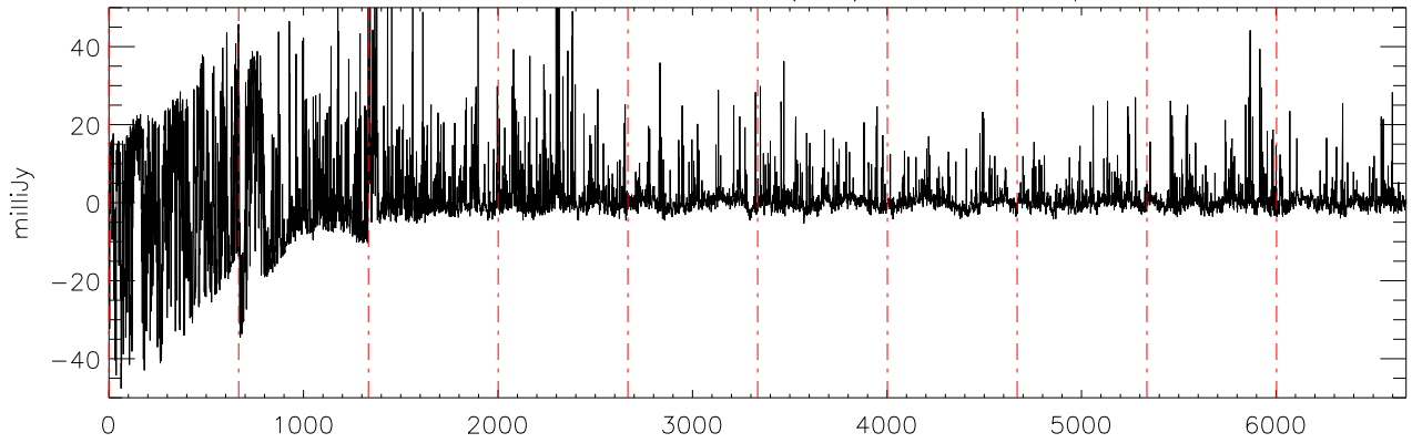
a2471 J10475385 02dec10 (AST) StokesQ freq:4750.
