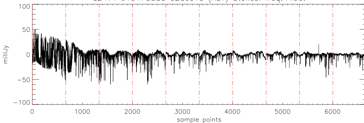
α2471 J10475385 02dec10 (AST) StokesI freq:4608.
