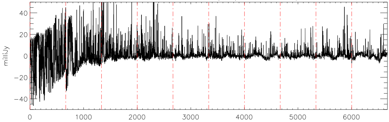
a2471 J10475385 02dec10 (AST) StokesQ freq:4608.
