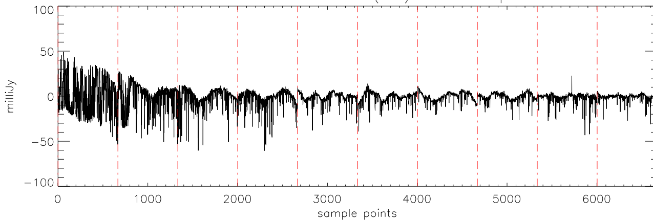
α2471 J10475385 02dec10 (AST) StokesI freq:4750.
