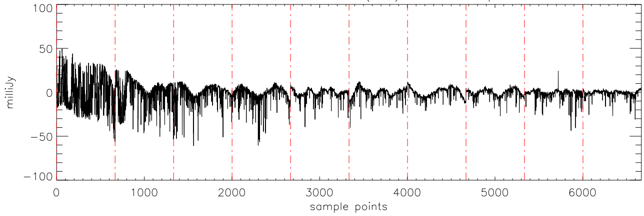
α2471 J10475385 02dec10 (AST) StokesI freq:5176.
