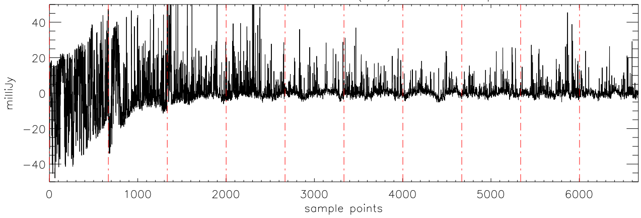
a2471 J10475385 02dec10 (AST) StokesQ freq:5176.
