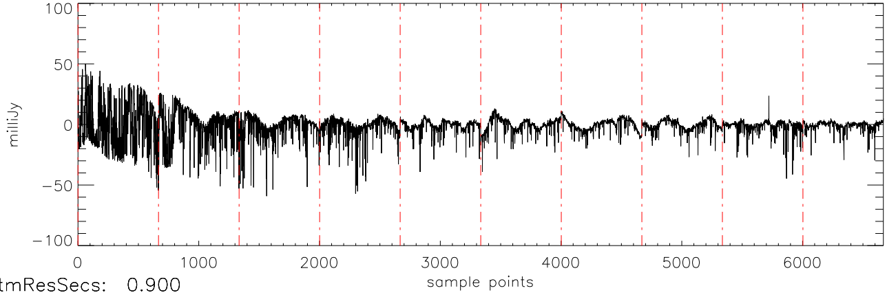
α2471 J10475385 02dec10 (AST) StokesI freq:5034.
