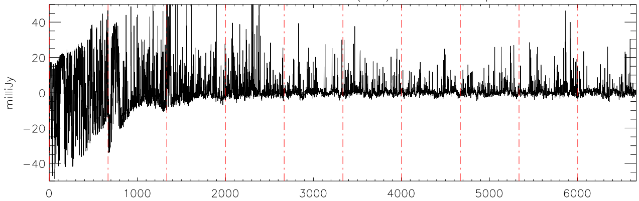
a2471 J10475385 02dec10 (AST) StokesQ freq:4466.
