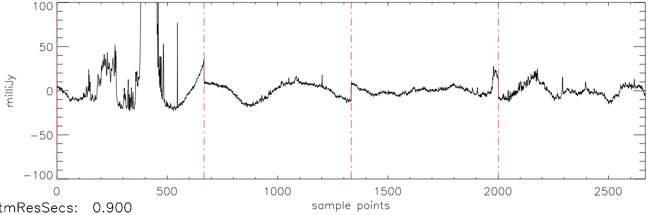
a2471 J07464256 07apr12 (AST) StokesI freq:4466.
