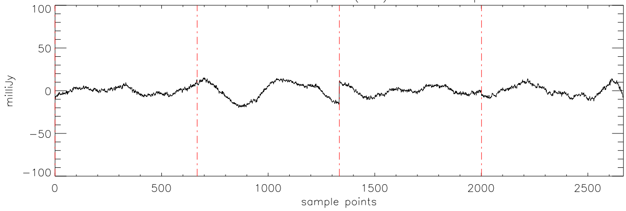
a2471 J07464256 07apr12 (AST) StokesI freq:5176.
