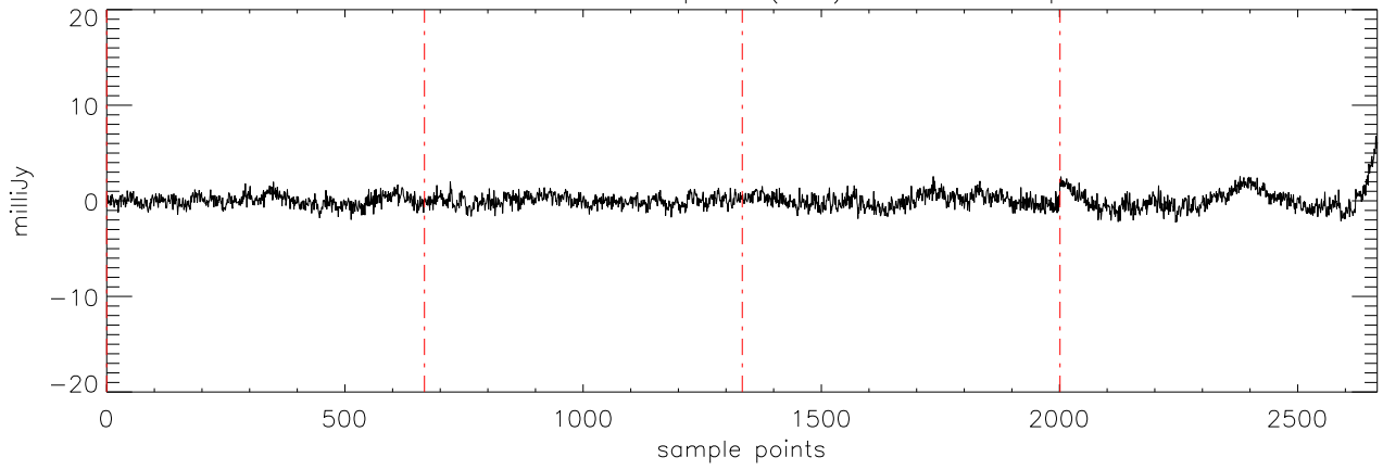
a2471 J07464256 07apr12 (AST) StokesU freq:5176.
