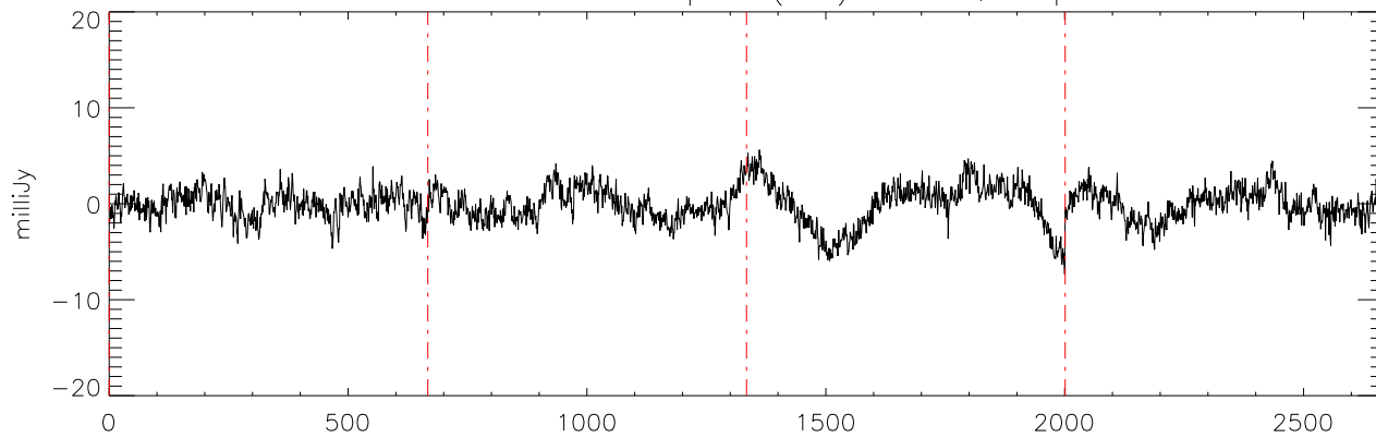
a2471 J07464256 07apr12 (AST) StokesQ freq:4608.
