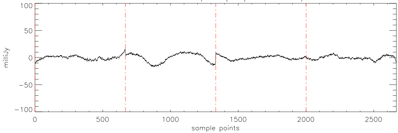
a2471 J07464256 07apr12 (AST) StokesI freq:4608.
