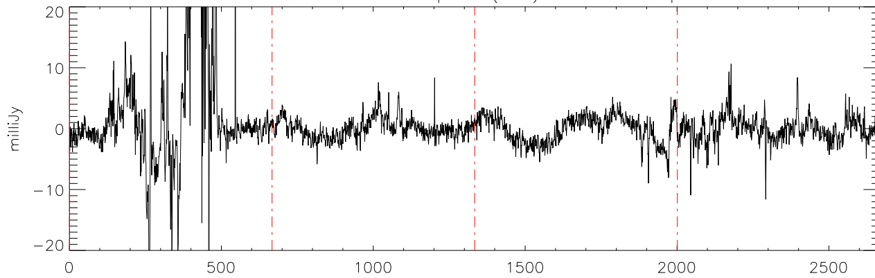
a2471 J07464256 07apr12 (AST) StokesQ freq:4325.
