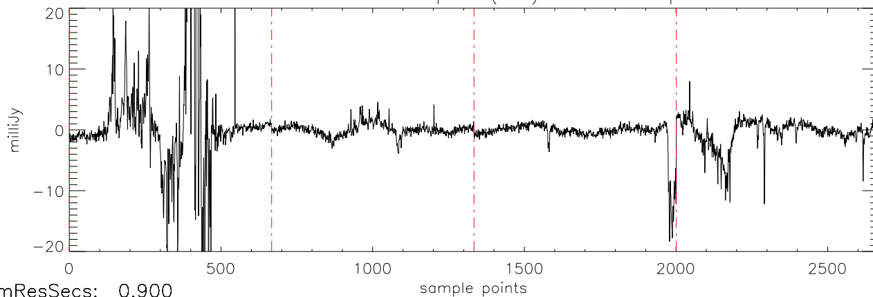
a2471 J07464256 07apr12 (AST) StokesU freq:4466.
