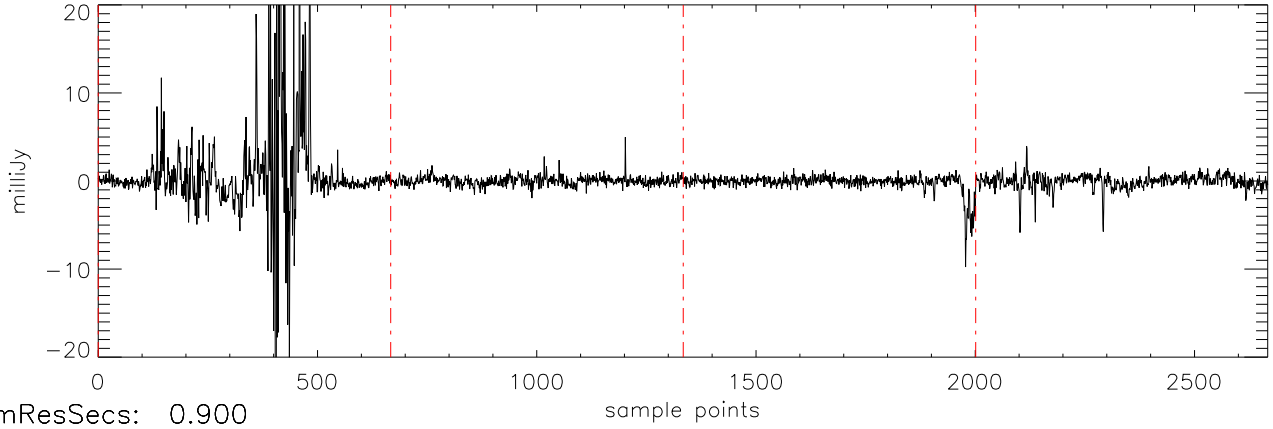
a2471 J07464256 07apr12 (AST) StokesV freq:4466.
