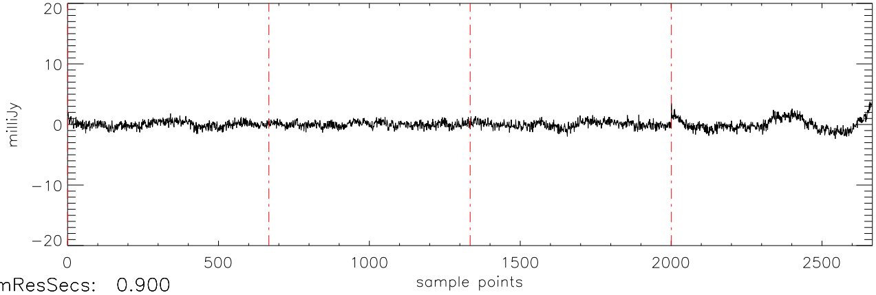
a2471 J07464256 07apr12 (AST) StokesU freq:5034.
