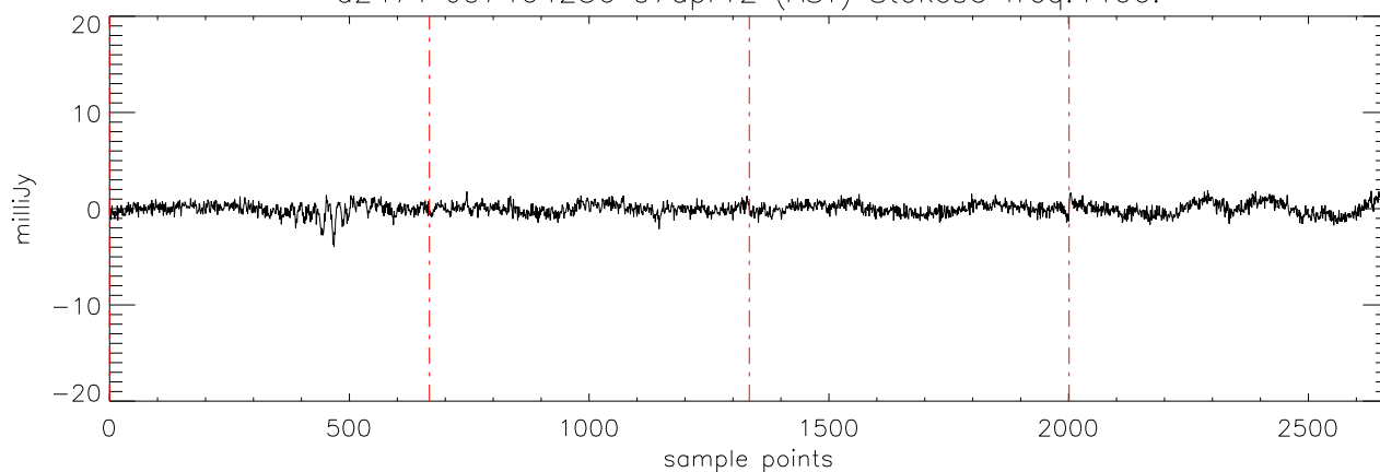
a2471 J07464256 07apr12 (AST) StokesU freq:4608.
