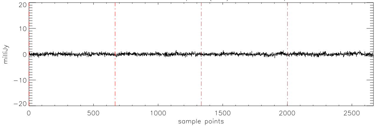
a2471 J07464256 07apr12 (AST) StokesV freq:4608.
