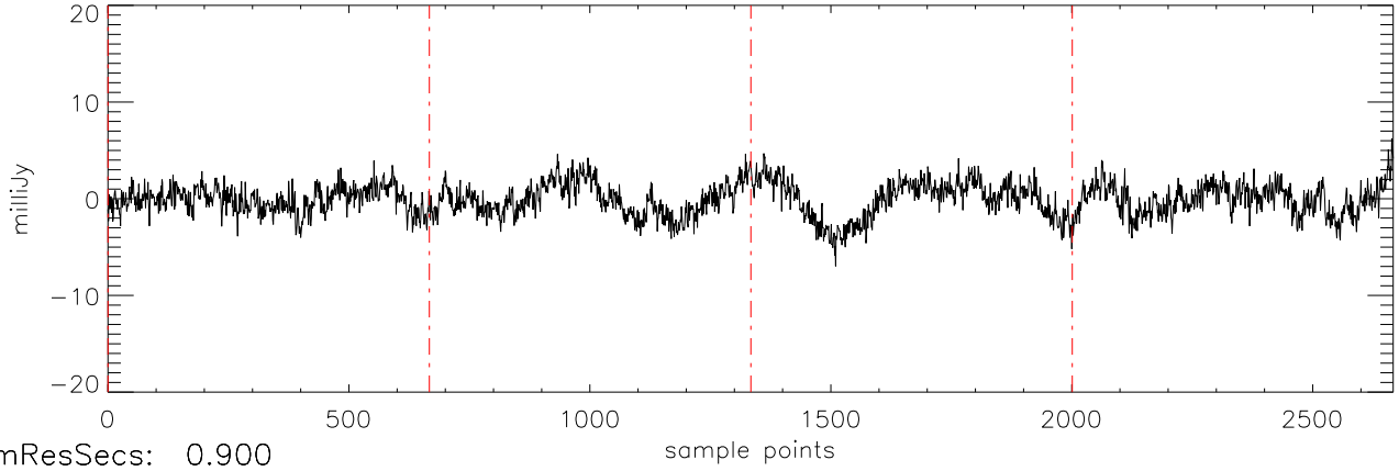
a2471 J07464256 07apr12 (AST) StokesQ freq:5034.
