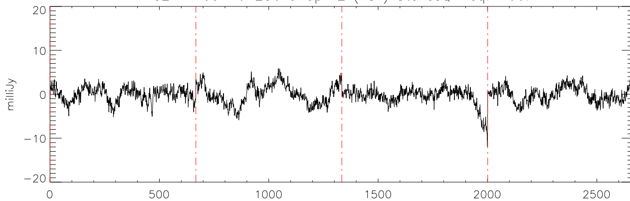
a2471 J07464256 07apr12 (AST) StokesQ freq:4466.
