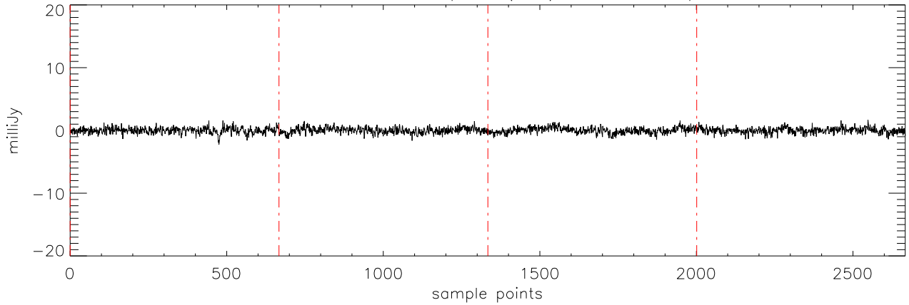
a2471 J07464256 07apr12 (AST) StokesV freq:4750.
