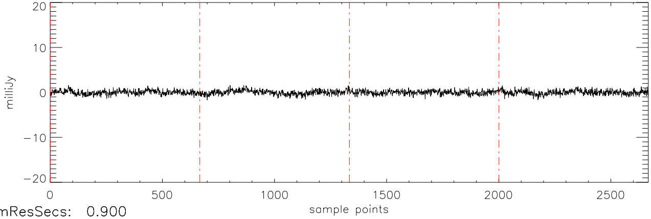
a2471 J07464256 07apr12 (AST) StokesV freq:5034.
