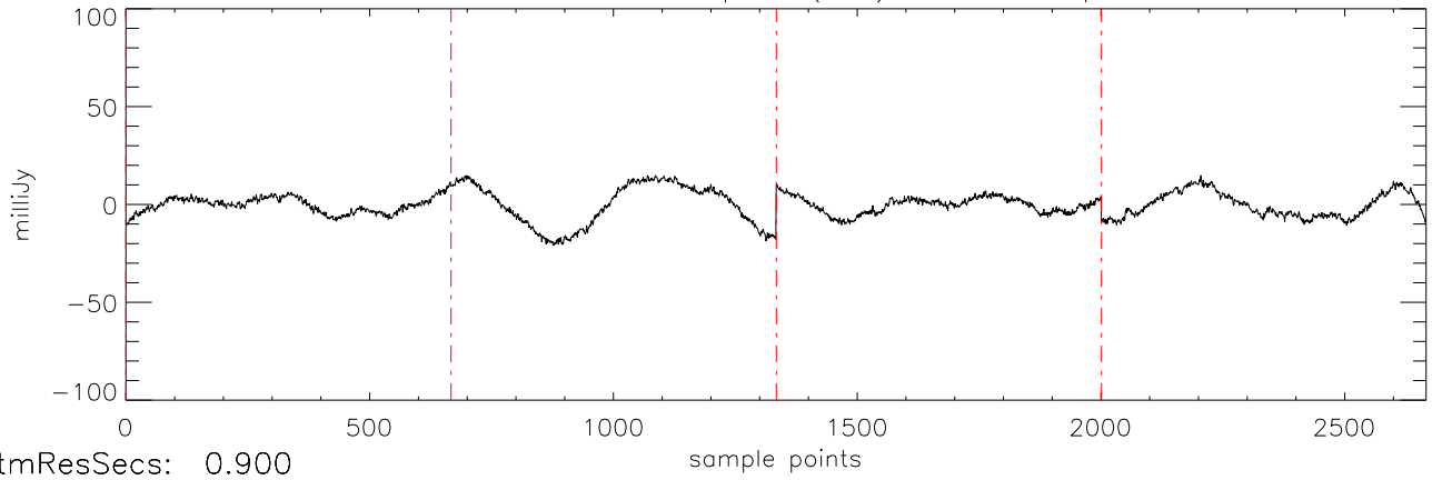
a2471 J07464256 07apr12 (AST) StokesI freq:5034.
