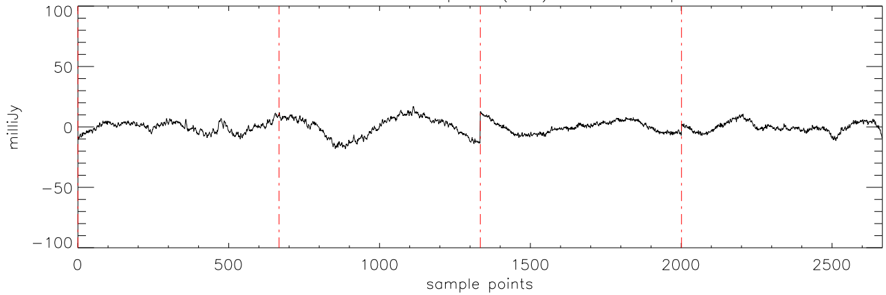
a2471 J07464256 07apr12 (AST) StokesI freq:4750.
