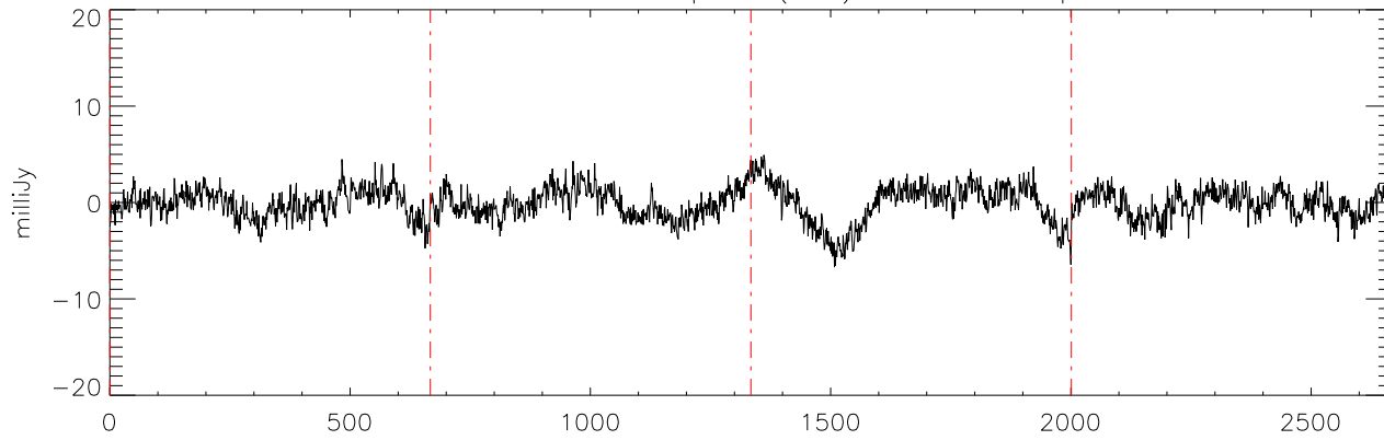
a2471 J07464256 07apr12 (AST) StokesQ freq:4750.
