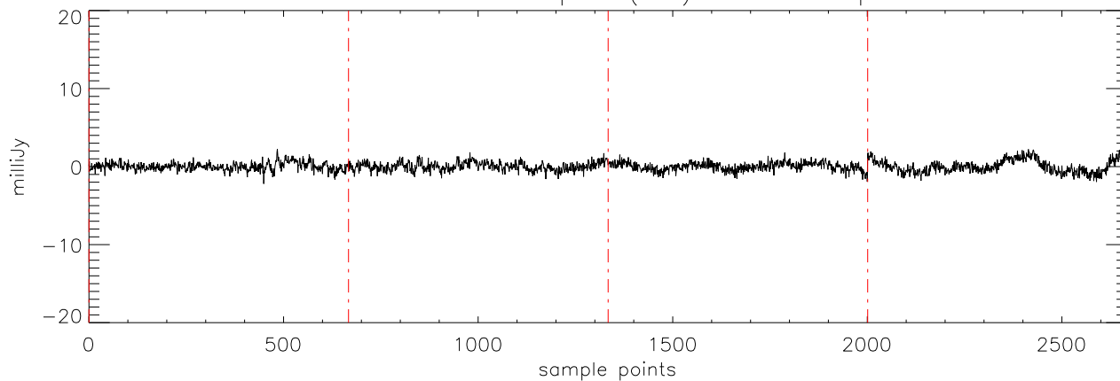
a2471 J07464256 07apr12 (AST) StokesU freq:4750.
