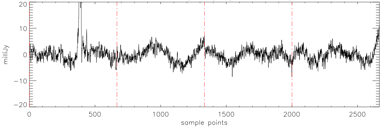
a2471 J07464256 07apr12 (AST) StokesQ freq:5176.
