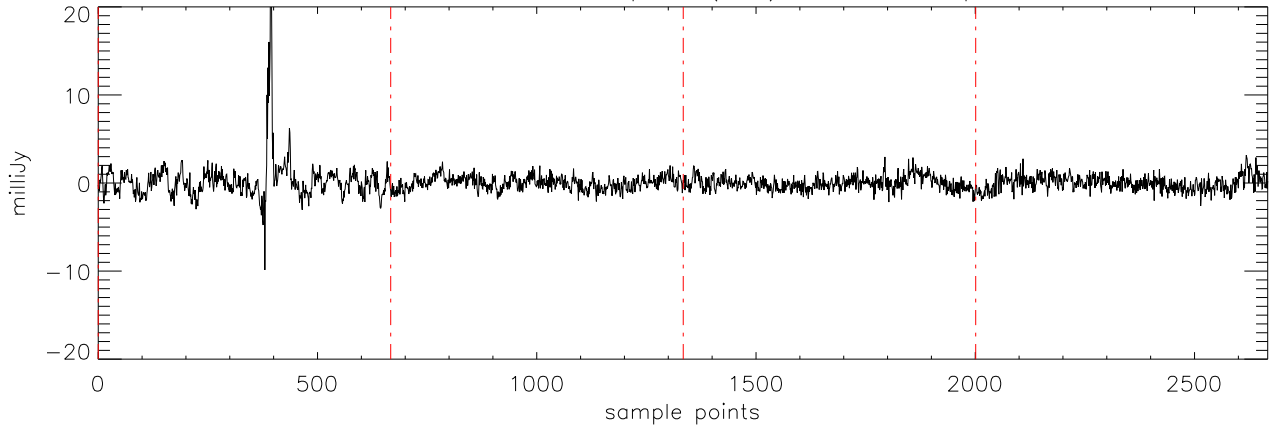
a2471 J07464256 07apr12 (AST) StokesV freq:5176.
