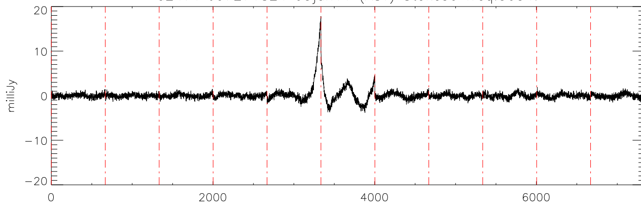
a2471 J07271824 03jan11 (AST) StokesU freq:5034.
