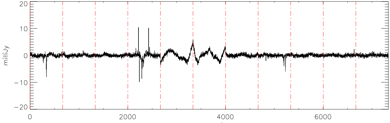
a2471 J07271824 03jan11 (AST) StokesU freq:4325.
