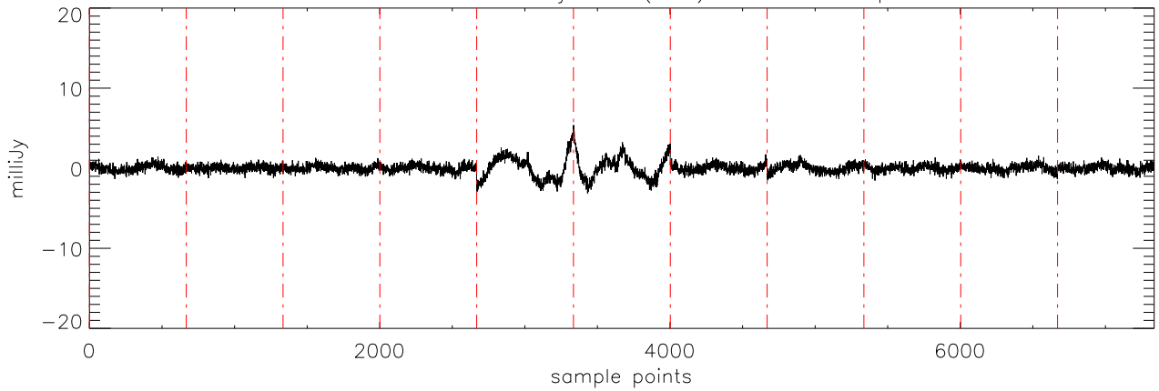
a2471 J07271824 03jan11 (AST) StokesU freq:4608.
