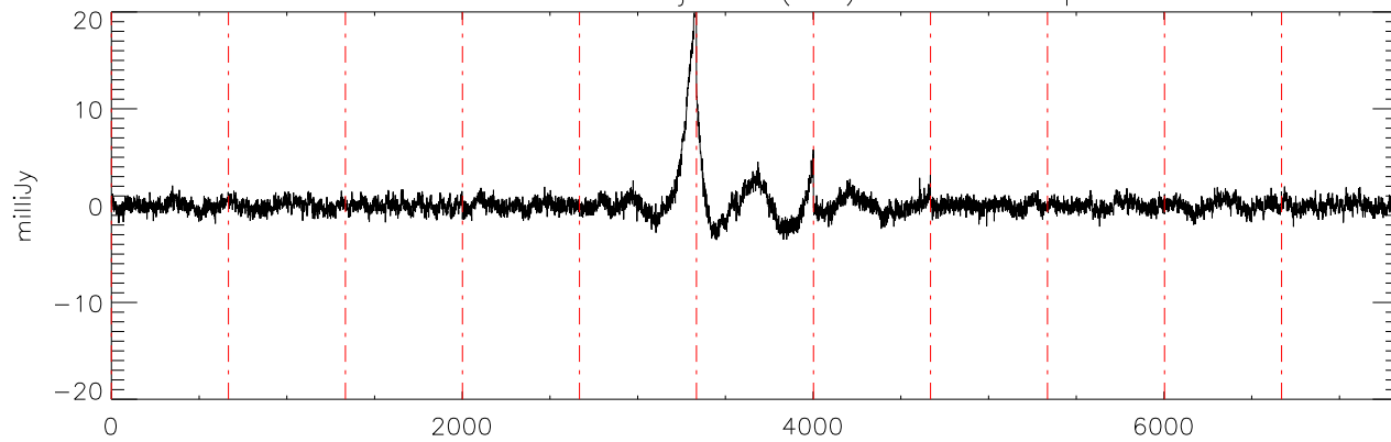
a2471 J07271824 03jan11 (AST) StokesU freq:5176.
