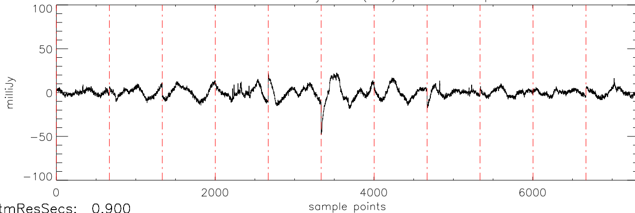
a2471 J07271824 03jan11 (AST) StokesI freq:4466.
