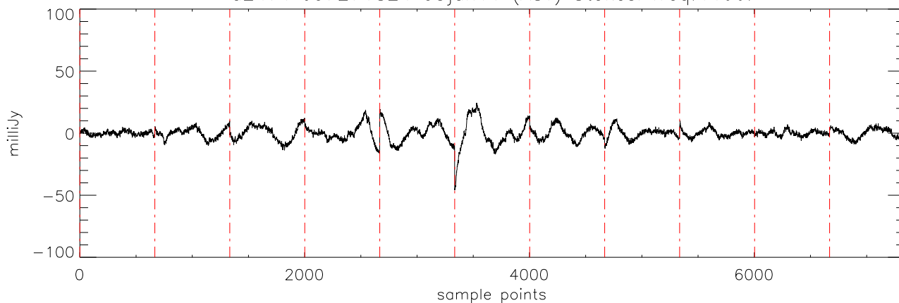
a2471 J07271824 03jan11 (AST) StokesI freq:4608.
