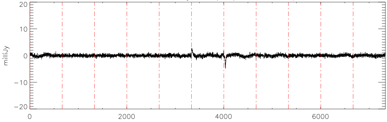
a2471 J07271824 03jan11 (AST) StokesV freq:4750.
