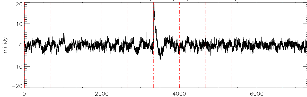
a2471 J07271824 03jan11 (AST) StokesQ freq:4892.
