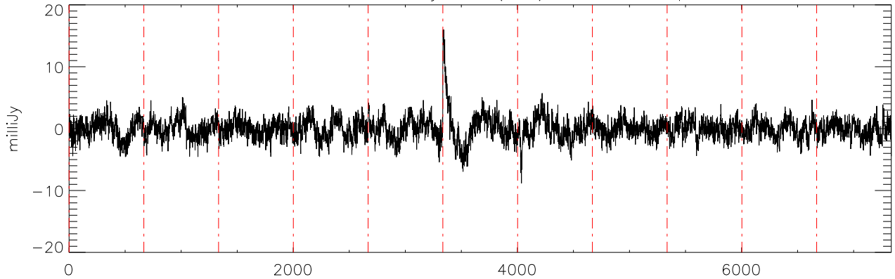
a2471 J07271824 03jan11 (AST) StokesQ freq:4750.
