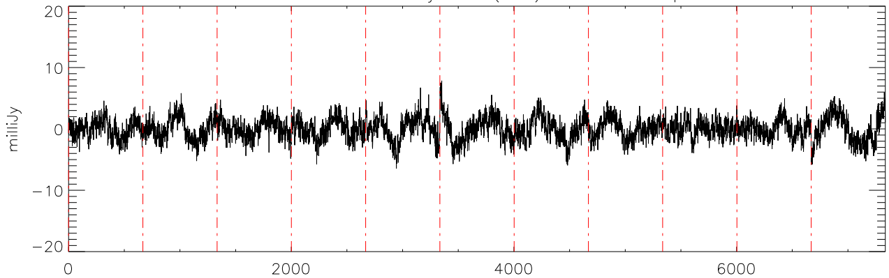
a2471 J07271824 03jan11 (AST) StokesQ freq:4466.
