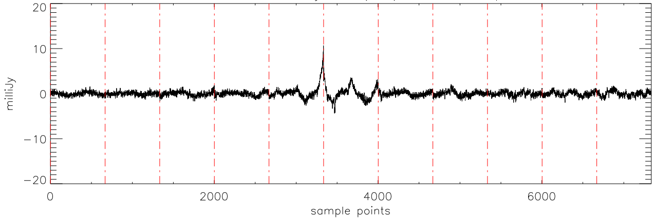
a2471 J07271824 03jan11 (AST) StokesU freq:4750.
