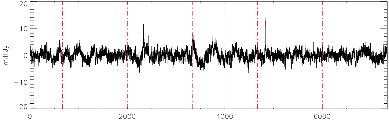
a2471 J07271824 03jan11 (AST) StokesQ freq:4325.
