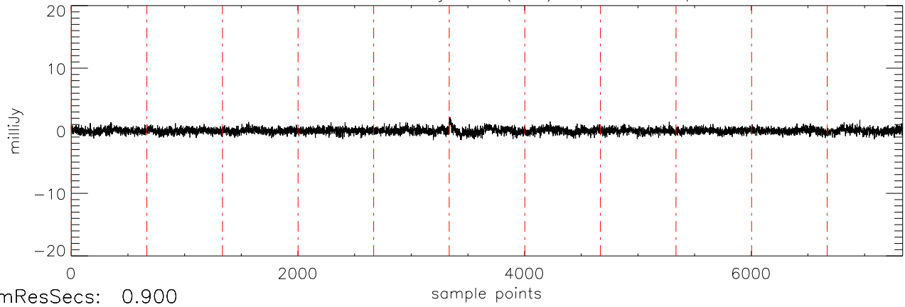
a2471 J07271824 03jan11 (AST) StokesV freq:5034.
