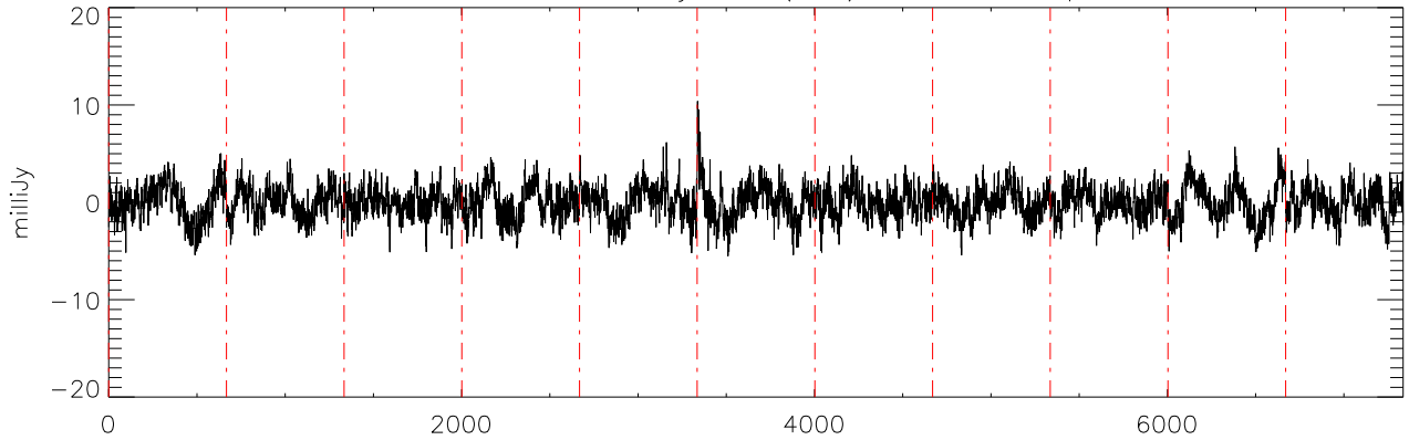
a2471 J07271824 03jan11 (AST) StokesQ freq:4608.
