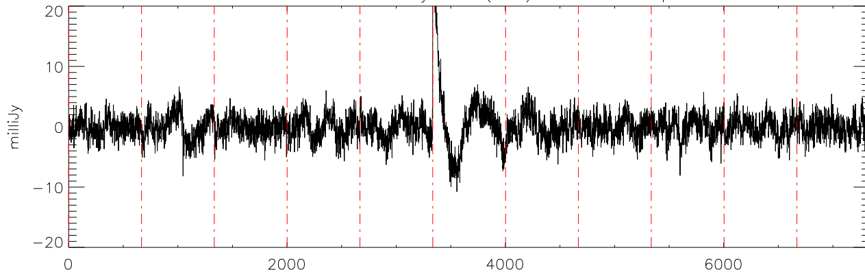
a2471 J07271824 03jan11 (AST) StokesQ freq:5176.
