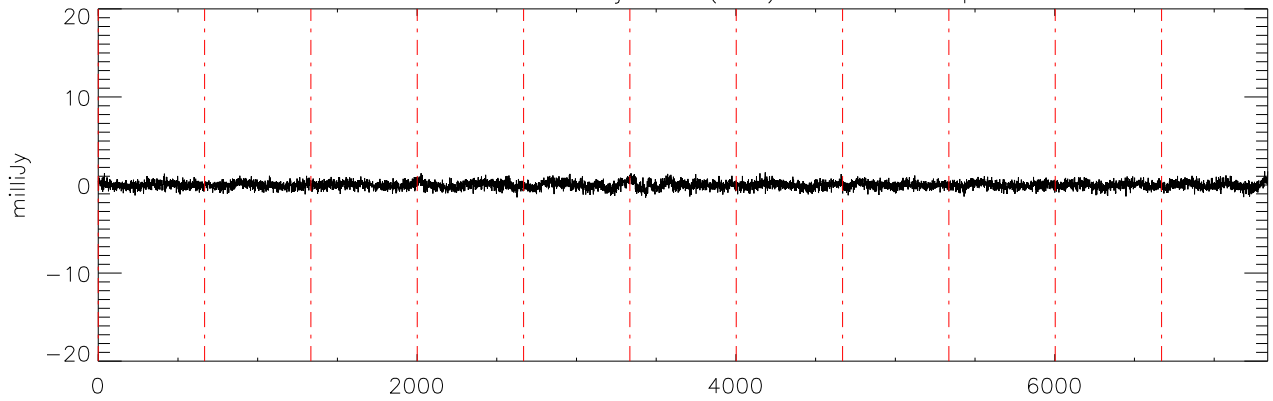
a2471 J07271824 03jan11 (AST) StokesV freq:4466.
