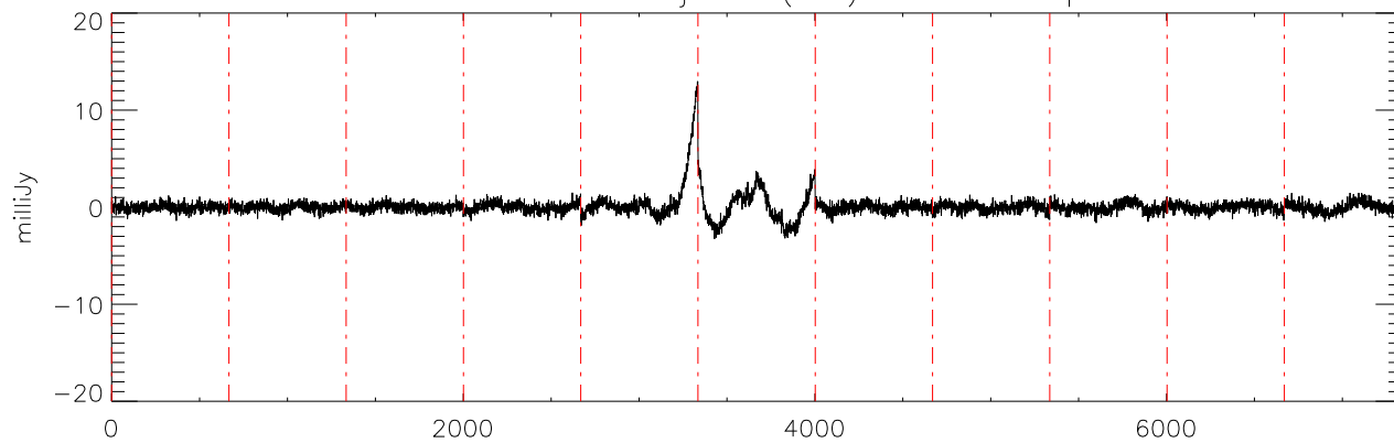
a2471 J07271824 03jan11 (AST) StokesU freq:4892.
