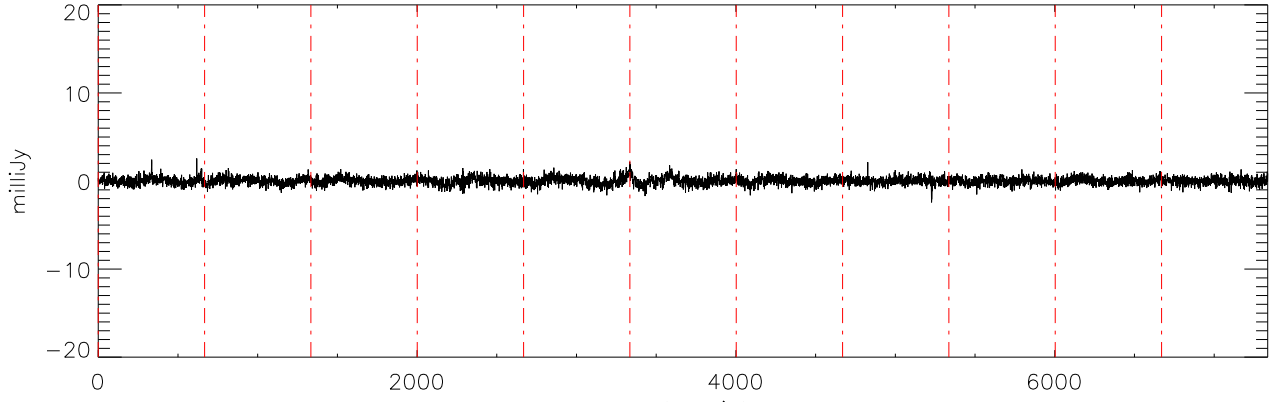
a2471 J07271824 03jan11 (AST) StokesV freq:4325.
