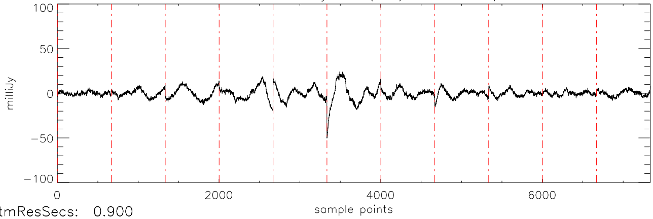
a2471 J07271824 03jan11 (AST) StokesI freq:5034.
