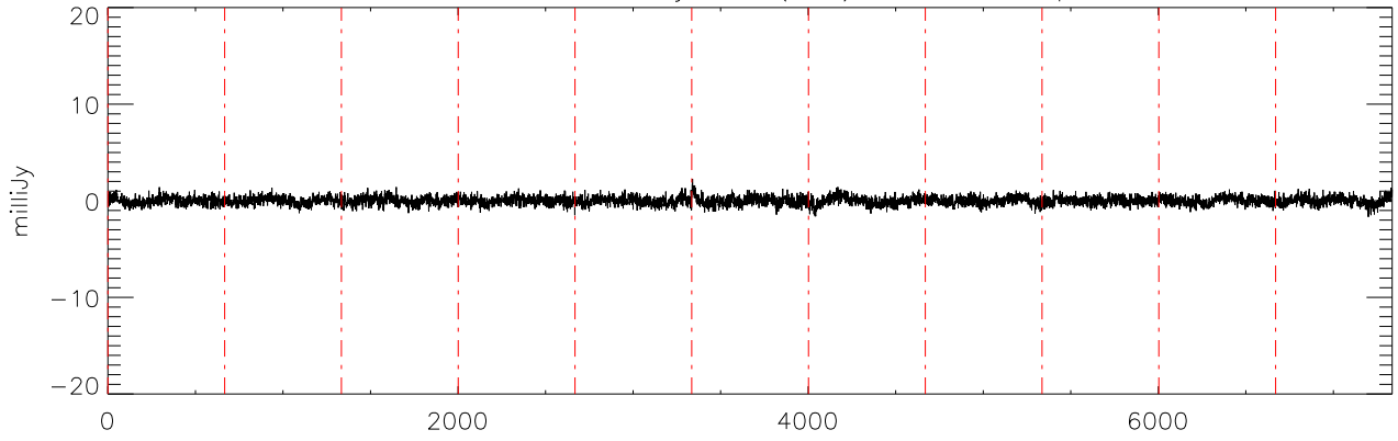
a2471 J07271824 03jan11 (AST) StokesV freq:4608.
