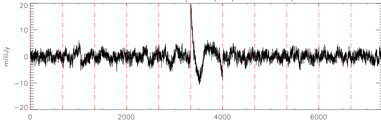
a2471 J07271824 03jan11 (AST) StokesQ freq:5034.
