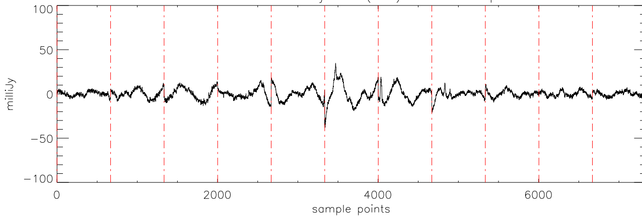
a2471 J07271824 03jan11 (AST) StokesI freq:4750.
