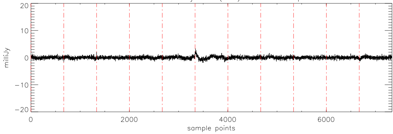
a2471 J07271824 03jan11 (AST) StokesV freq:5176.
